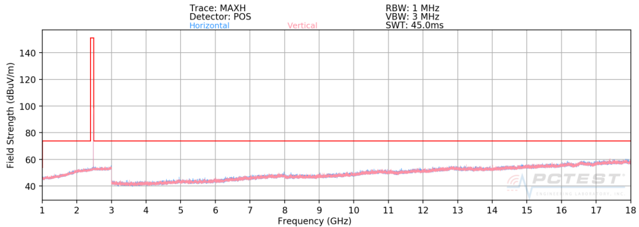
Plot 7-47. Radiated Spurious Plot ((HDR, ePA), 4Mbps, ePA – Ch. 75, Ant. Pol. H & V)
