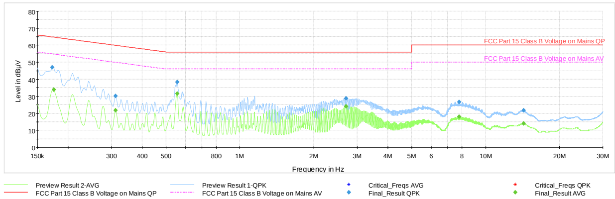
Plot 7-60. Line Conducted Plot with Bluetooth HDR (N, with WCP + Laptop)
