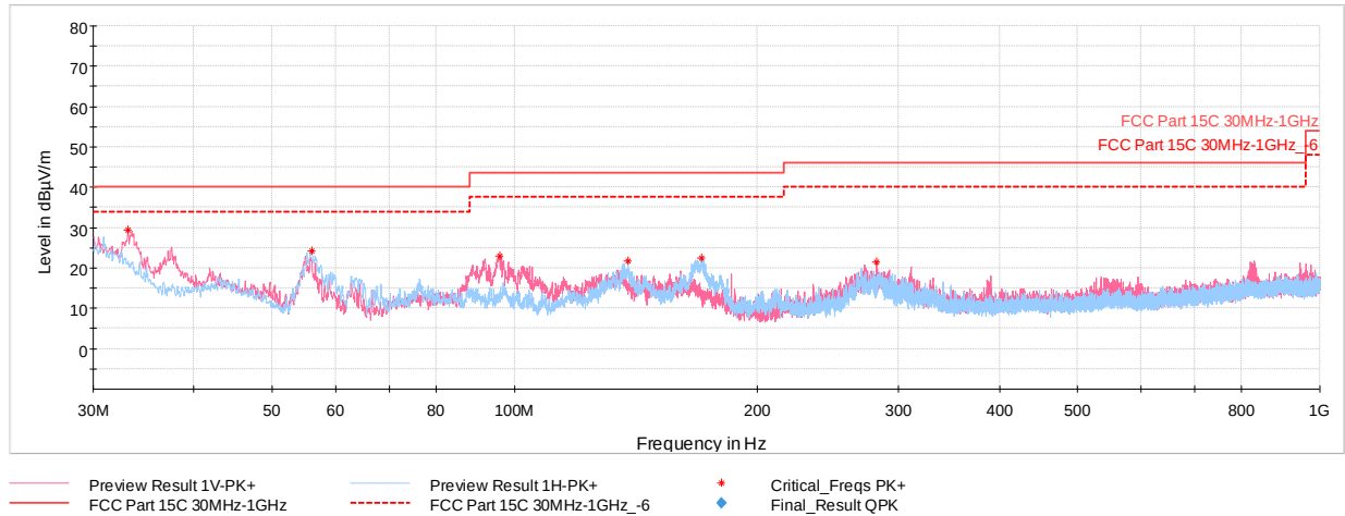
Plot 7-58. Radiated Spurious Plot below 1GHz (8Mbps, ePA, Pol. H & V, with WCP + Laptop)
