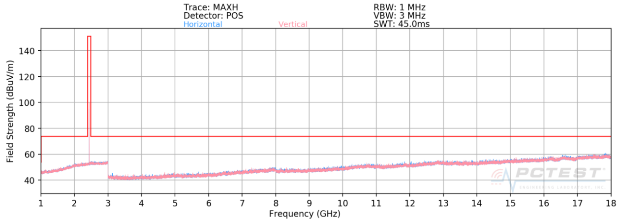
Plot 7-46. Radiated Spurious Plot ((HDR, ePA), 4Mbps, ePA – Ch. 38, Ant. Pol. H & V)
