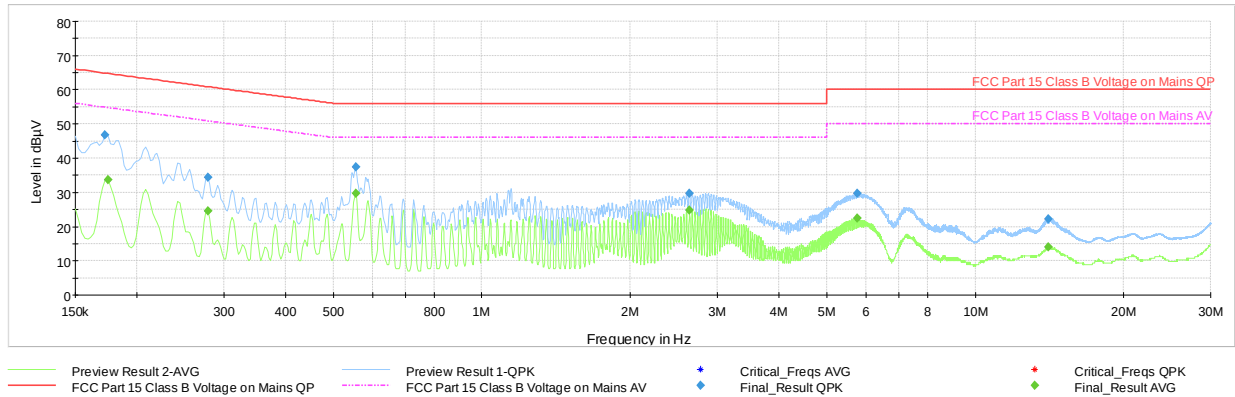
Plot 7-59. Line Conducted Plot with Bluetooth HDR (L1, with WCP + Laptop)
