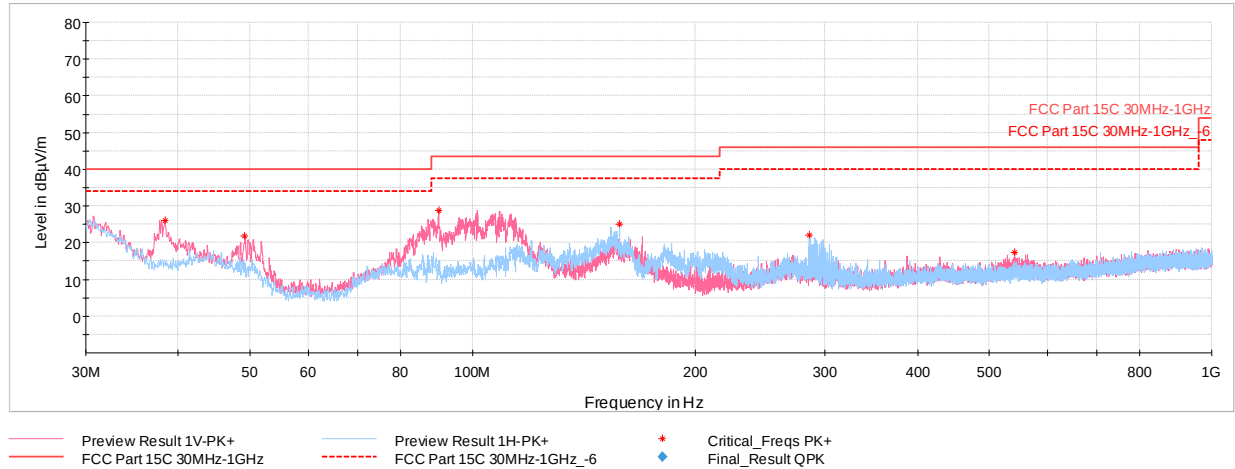
Plot 7-54. Radiated Spurious Plot below 1GHz (1Mbps, ePA, Pol. H & V, with WCP + Laptop)
