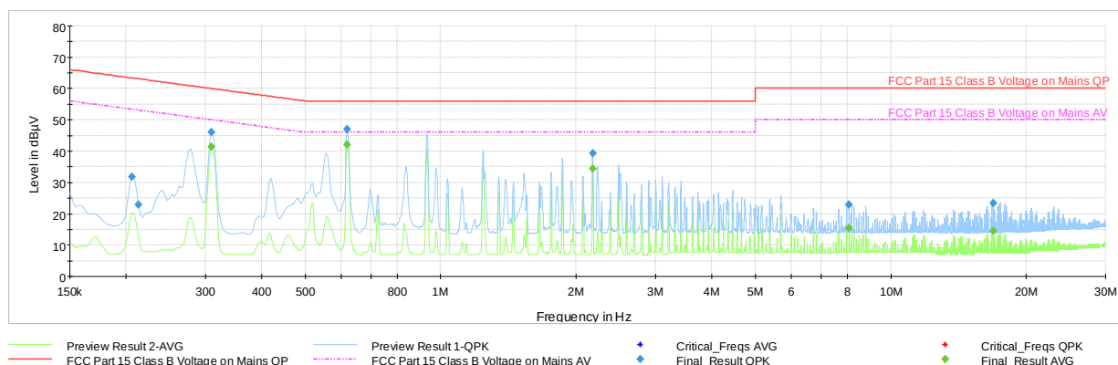
Plot 7-55. Line Conducted Plot with Bluetooth LE (L1, with WCP + AC/DC Adapter)
