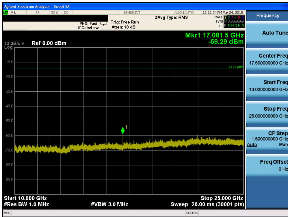
Plot 7-42. Conducted Spurious Plot (Bluetooth (LE), 1Mbps, iPA – Ch. 19)
