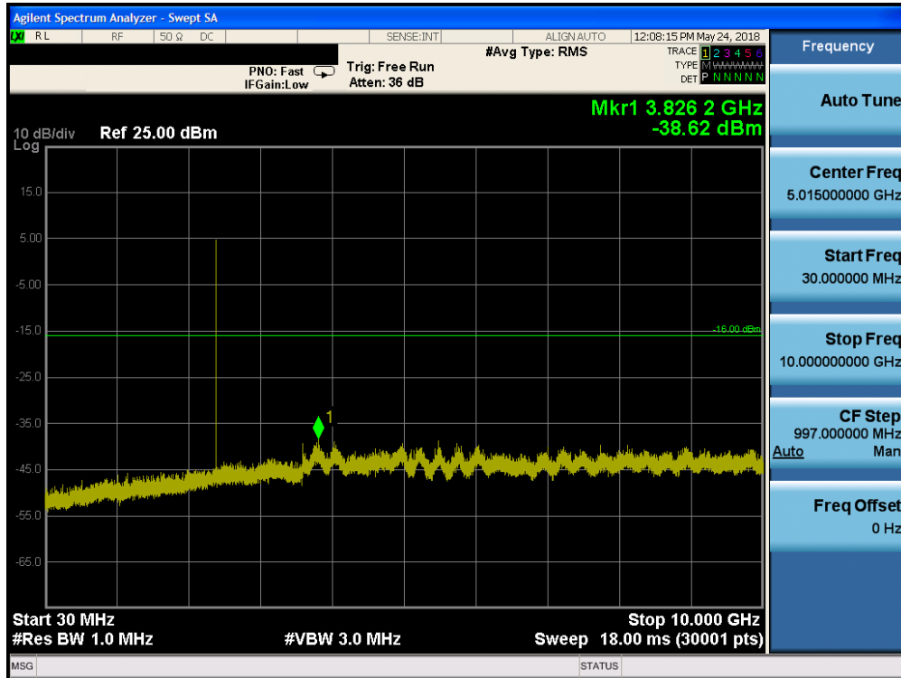
Plot 7-39. Conducted Spurious Plot (Bluetooth (LE), 1Mbps, iPA – Ch. 0)
