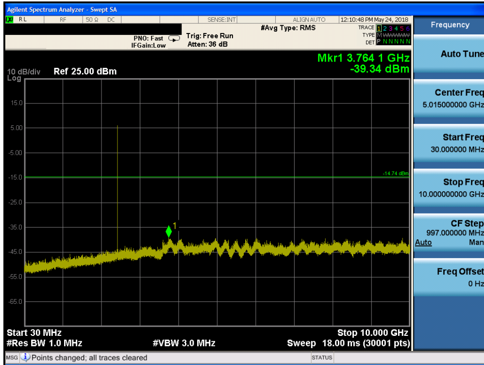
Plot 7-41. Conducted Spurious Plot (Bluetooth (LE), 1Mbps, iPA – Ch. 19)
