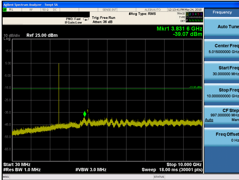
Plot 7-43. Conducted Spurious Plot (Bluetooth (LE), 1Mbps, iPA – Ch. 39)
