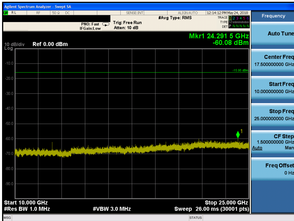
Plot 7-44. Conducted Spurious Plot (Bluetooth (LE), 1Mbps, iPA – Ch. 39)
