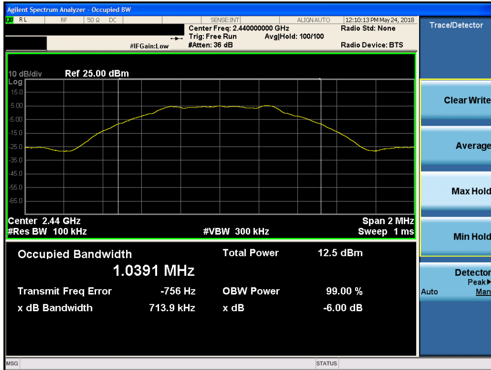
Plot 7-5. 6dB Bandwidth Plot (Bluetooth (LE), iPA, 1Mbps – Ch. 19)
