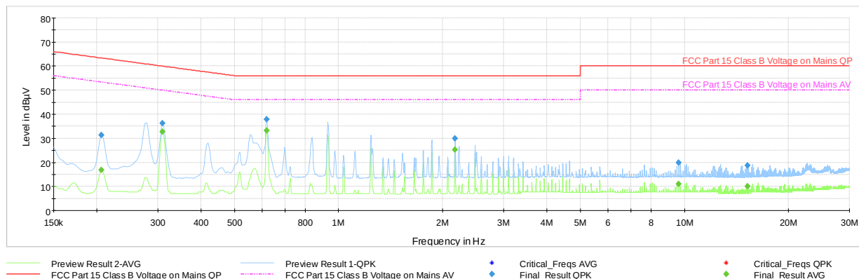
Plot 7-56. Line Conducted Plot with Bluetooth LE (N, with WCP + AC/DC Adapter)
