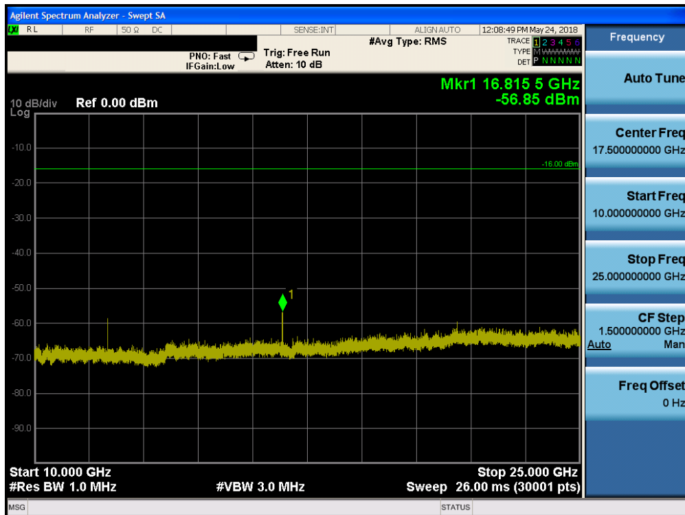
Plot 7-40. Conducted Spurious Plot (Bluetooth (LE), 1Mbps, iPA – Ch. 0)
