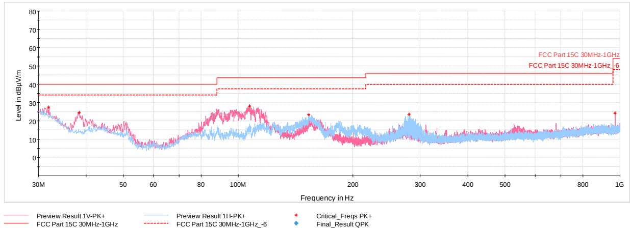
Plot 7-74. Radiated Spurious Plot below 1GHz (GFSK ePA, Pol. H & V, with WCP + Laptop)
