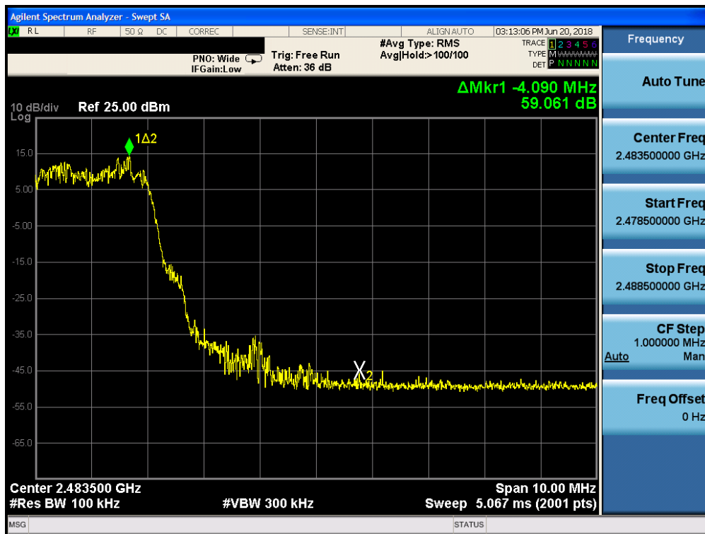
Plot 7-36. Band Edge Plot (Bluetooth with Hopping Enabled, 8DPSK, ePA)
