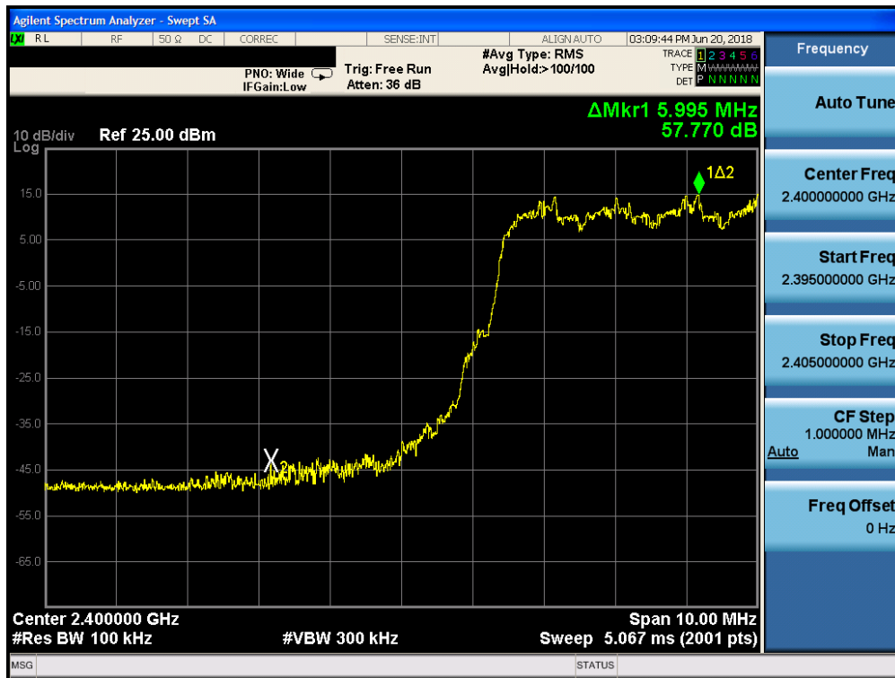
Plot 7-35. Band Edge Plot (Bluetooth with Hopping Enabled, 8DPSK, ePA)
