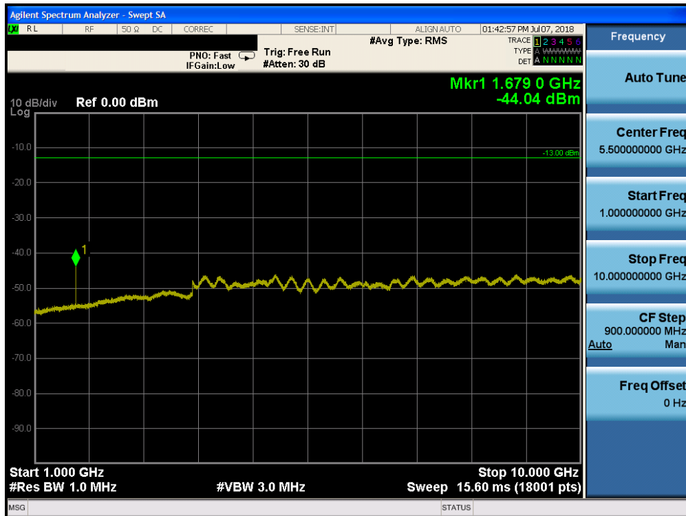
Plot 7-42. Conducted Spurious Plot (Band 26/5 - 10.0MHz QPSK - RB Size 1, RB Offset 0 - High Channel)
