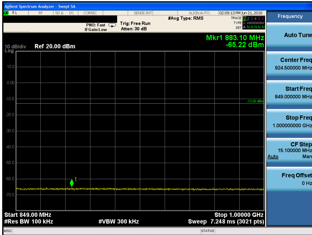
Plot 7-35. Conducted Spurious Plot (Band 26/5 - 10.0MHz QPSK - RB Size 1, RB Offset 0 - Low Channel)
