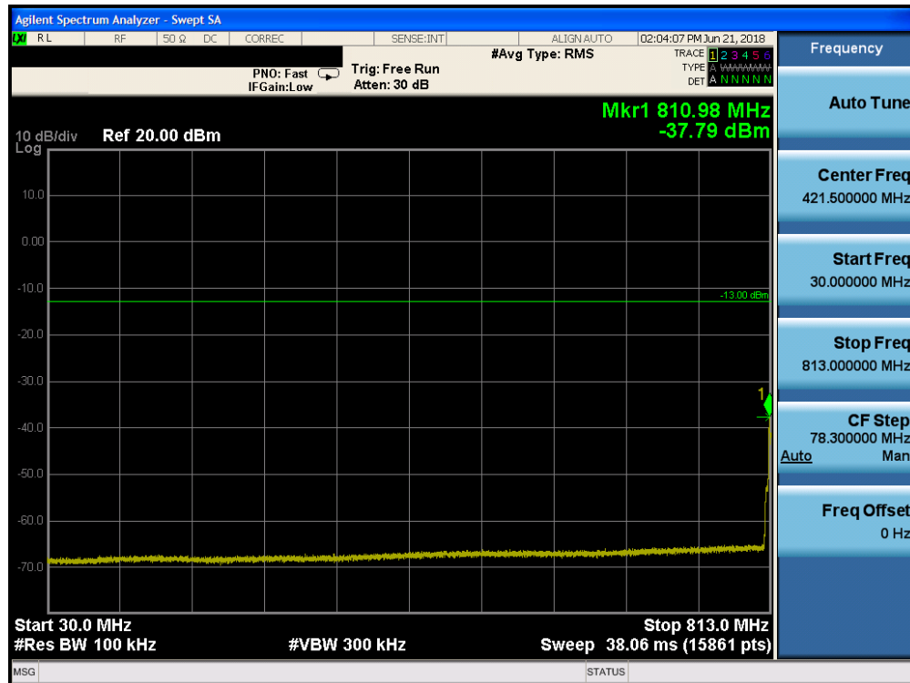
Plot 7-34. Conducted Spurious Plot (Band 26/5 - 10.0MHz QPSK - RB Size 1, RB Offset 0 - Low Channel)
