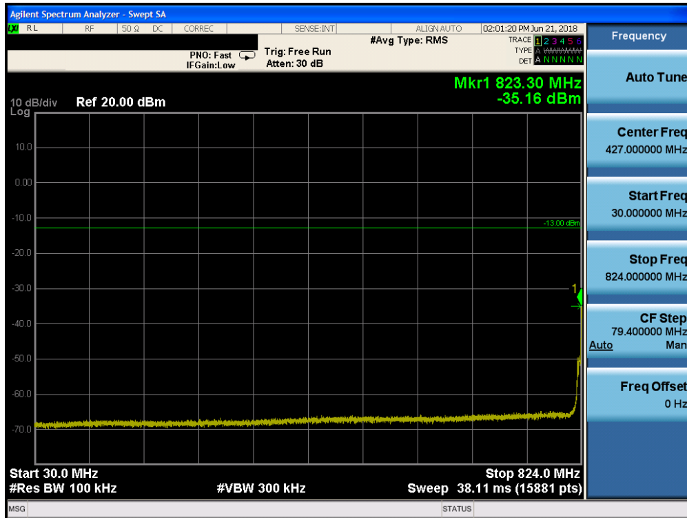
Plot 7-37. Conducted Spurious Plot (Band 26/5 - 10.0MHz QPSK - RB Size 1, RB Offset 0 - Mid Channel)
