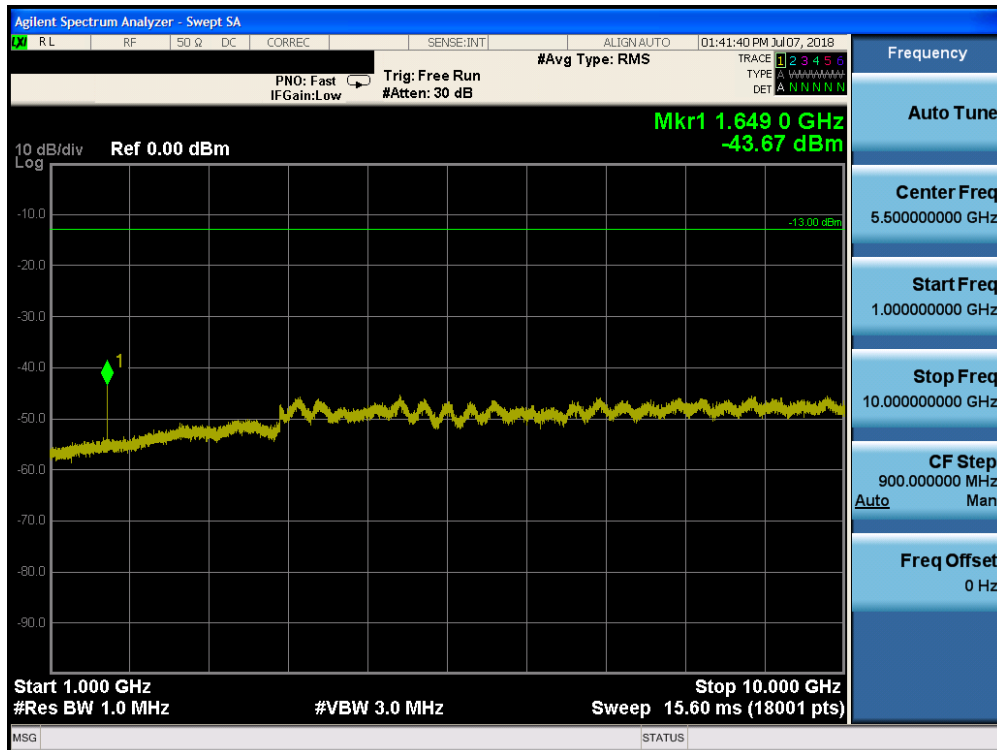
Plot 7-36. Conducted Spurious Plot (Band 26/5 - 10.0MHz QPSK - RB Size 1, RB Offset 0 - Low Channel)
