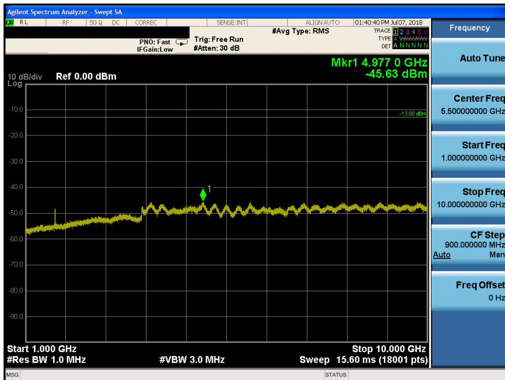
Plot 7-38. Conducted Spurious Plot (Band 26/5 - 10.0MHz QPSK - RB Size 1, RB Offset 0 - Mid Channel)
