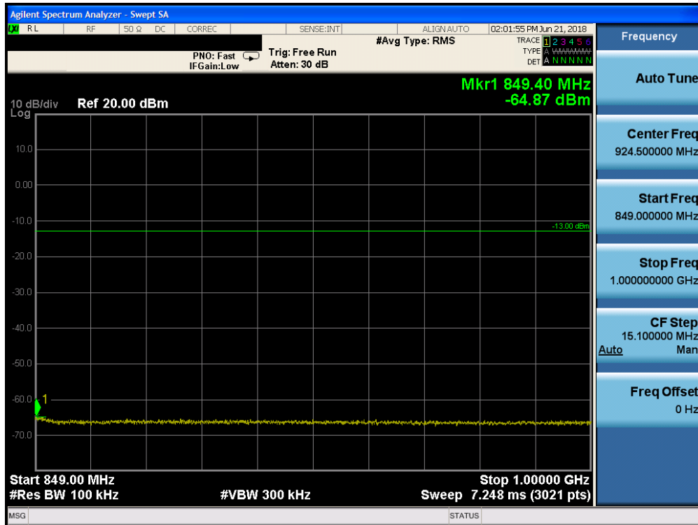
Plot 7-39. Conducted Spurious Plot (Band 26/5 - 10.0MHz QPSK - RB Size 1, RB Offset 0 - Mid Channel)
