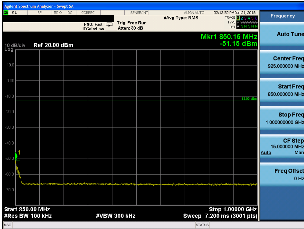
Plot 7-41. Conducted Spurious Plot (Band 26/5 - 10.0MHz QPSK - RB Size 1, RB Offset 0 - High Channel)
