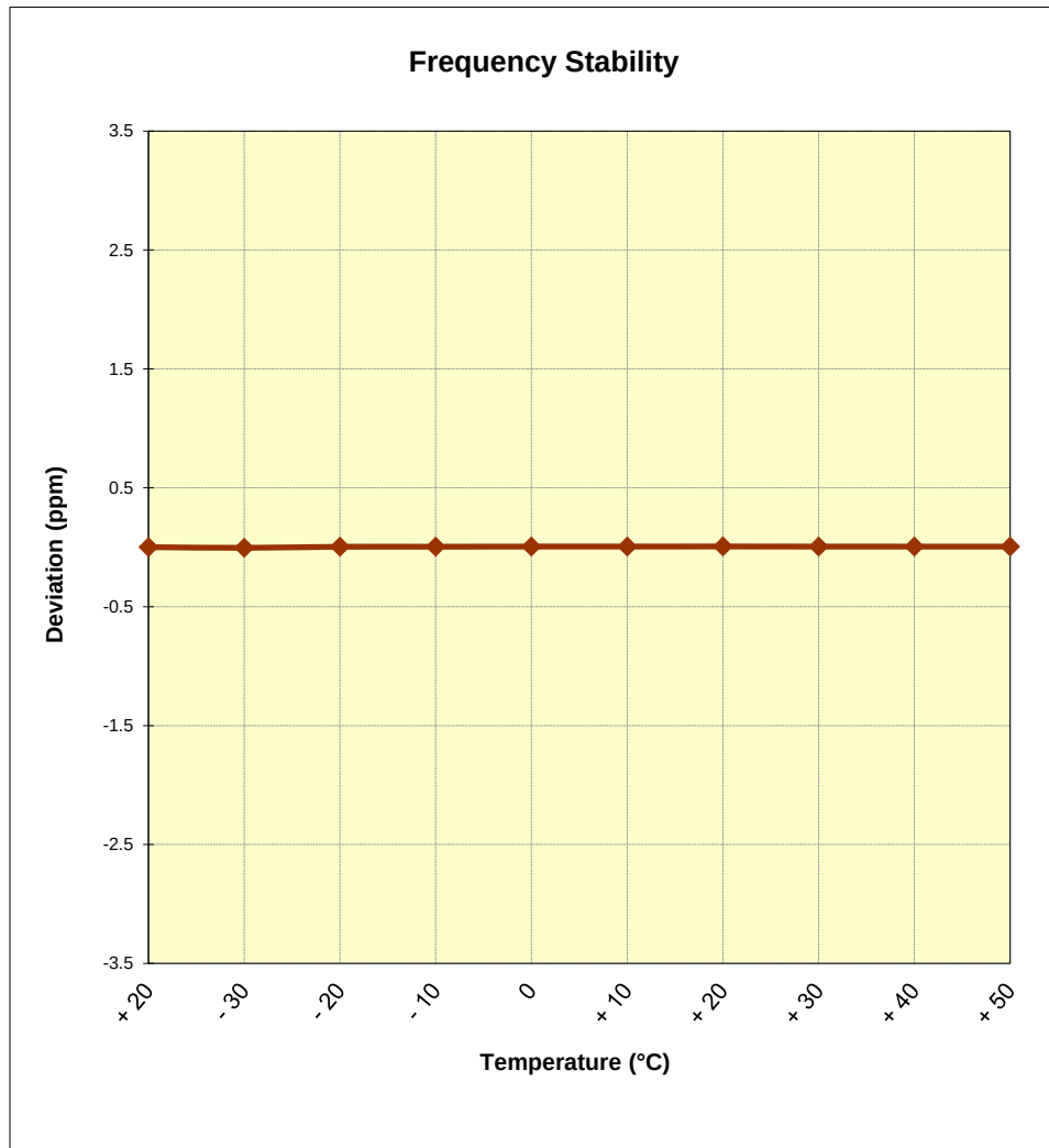
Figure 7-6. Frequency Stability Graph (Band 26/5)
