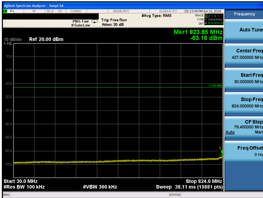
Plot 7-40. Conducted Spurious Plot (Band 26/5 - 10.0MHz QPSK - RB Size 1, RB Offset 0 - High Channel)
