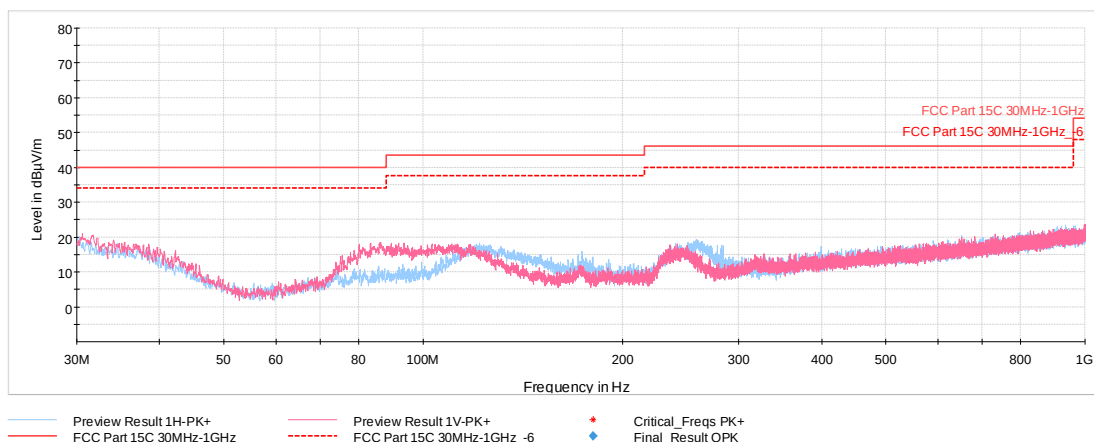
Plot 7-6. Radiated Spurious Plot 30MHz – 1GHz (Reader 100 Ask 1 out of 4, Pol. H & V, with WCP + AC/DC Adapter attached)
