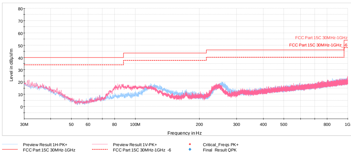
Plot 7-5. Radiated Spurious Plot 30MHz – 1GHz (CE A 848kbps, Pol. H & V, with WCP + AC/DC Adapter attached)
