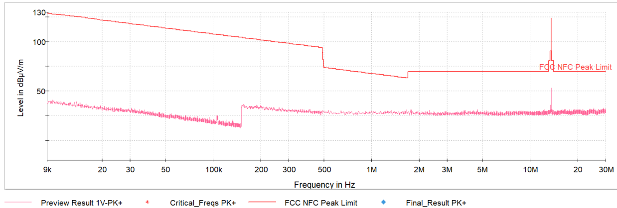
Plot 7-4. Radiated Spurious Plot 9kHz – 30MHz (Reader 100 Ask 1 out of 4, Pol. X)
