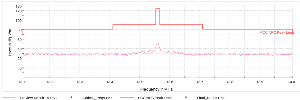
Plot 7-2. In Band Radiated Spurious Plot (Reader 100 Ask 1 out of 4, Pol. X)
