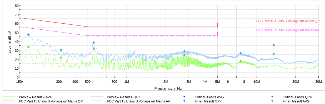
Plot 7-8. Line-Conducted Test Plot (N, with WCP + Laptop)
