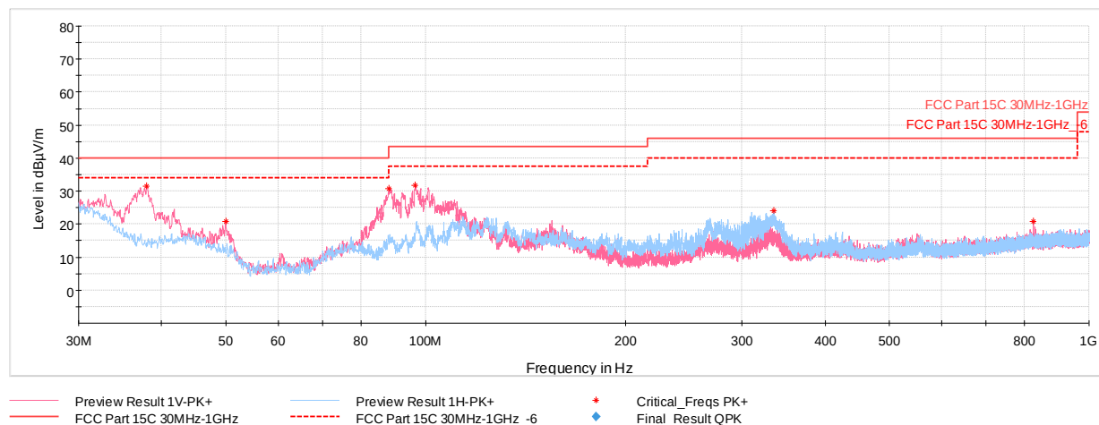
Plot 7-45. Radiated Spurious Plot below 1GHz (802.11b – Ch. 7, Pol. H & V, with WCP + Laptop)
