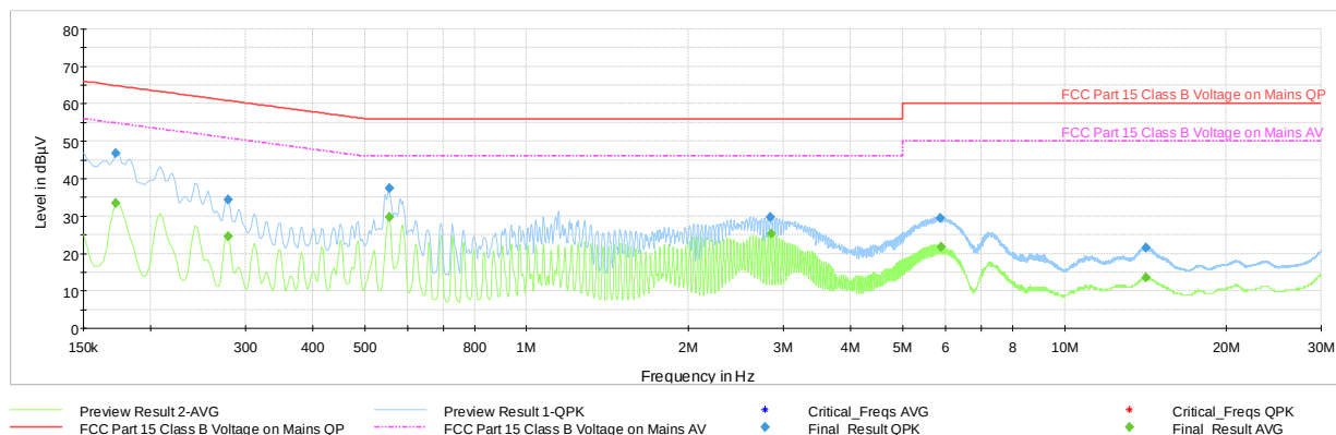
Plot 7-46. Line Conducted Plot with 802.11b (L1, with WCP + Laptop)
