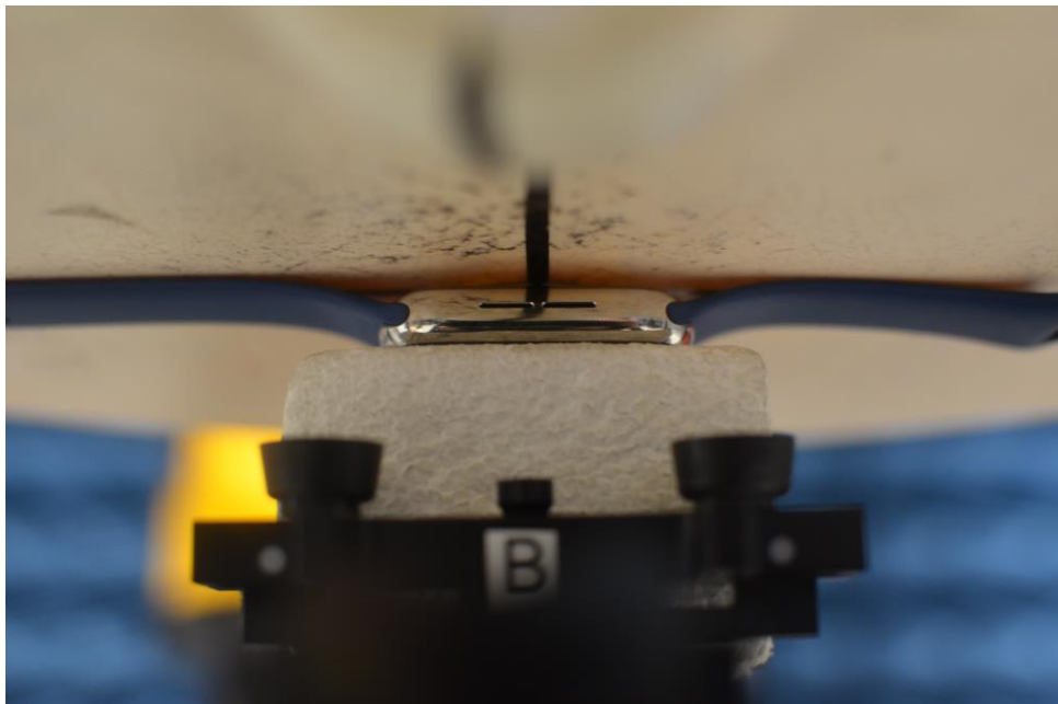
SAR Test Setup Photo 12: Stainless Steel with Sport Wristband, Back side at 0.0 cm
