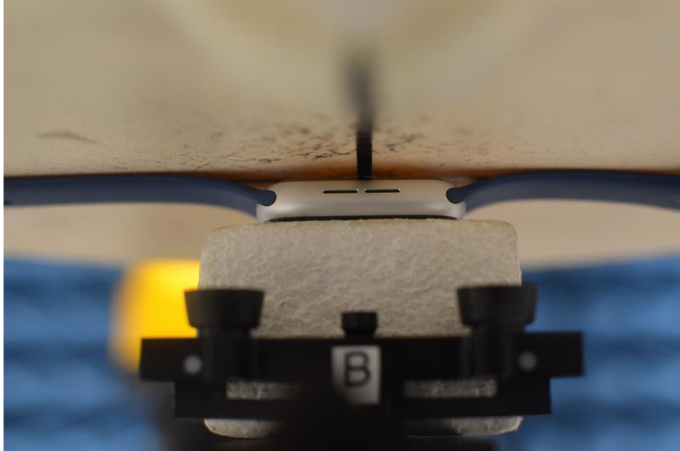
SAR Test Setup Photo 9: Aluminum with Sport Wristband, Back side at 0.0 cm
