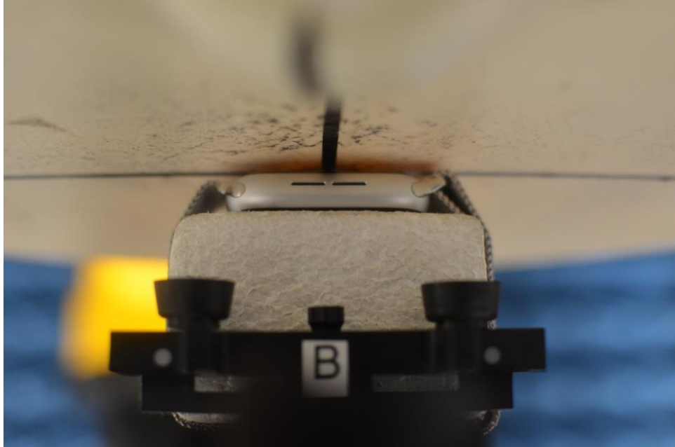
SAR Test Setup Photo 7: Aluminum with Metal Loop Wristband, Back side at 0.0 cm
