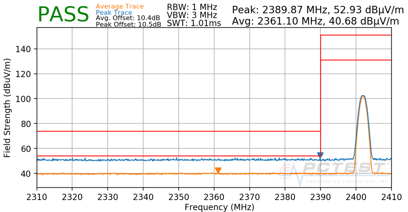
Plot 7-34. Radiated Restricted Lower Band Edge Measurement
