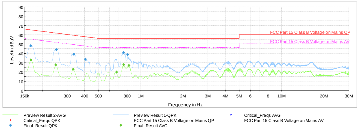
Plot 7-40. Line-Conducted Test Plot – Ch.39 (N, with WCP + AC/DC Adapter)
