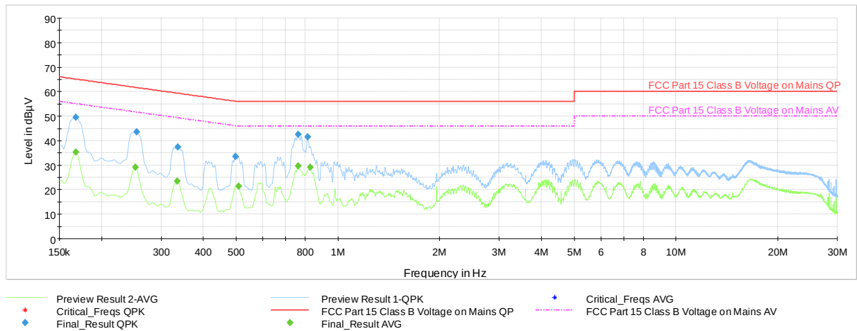
Plot 7-39. Line-Conducted Test Plot – Ch.39 (L1, with WCP + AC/DC Adapter)
