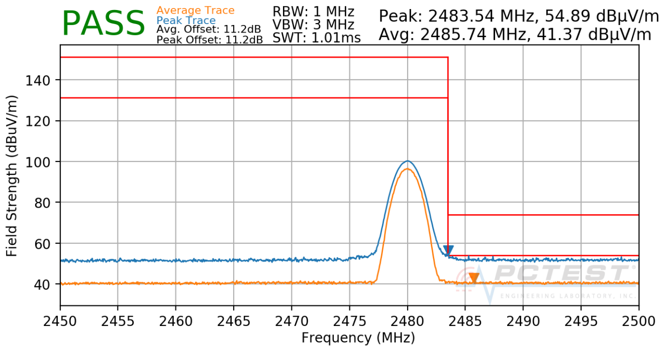
Plot 7-37. Radiated Restricted Upper Band Edge Measurement
