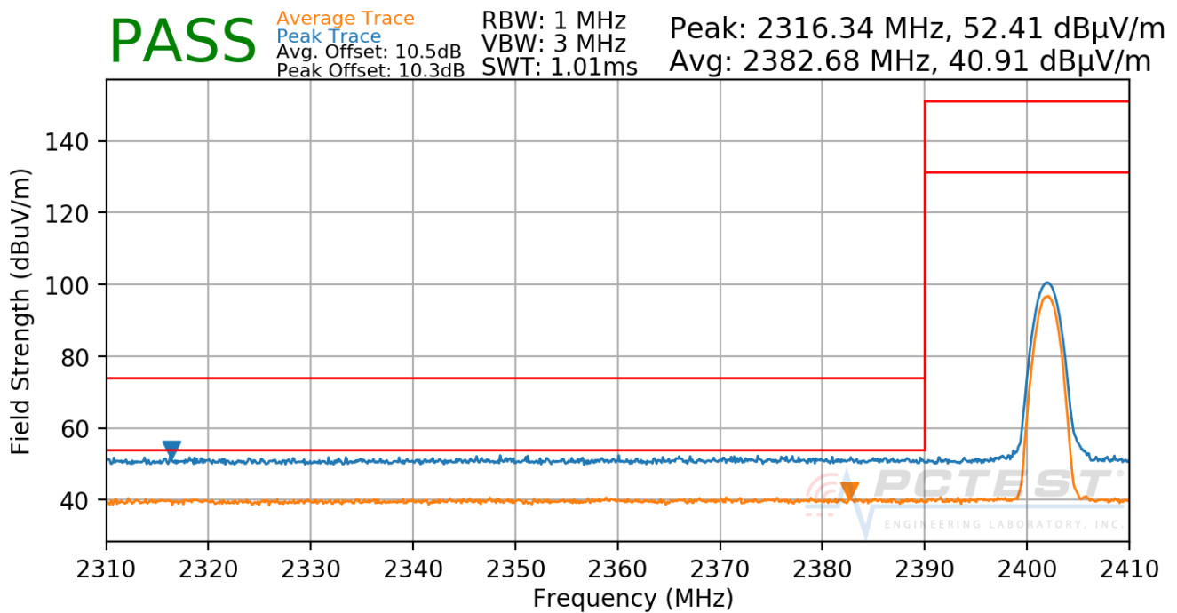
Plot 7-35. Radiated Restricted Lower Band Edge Measurement
