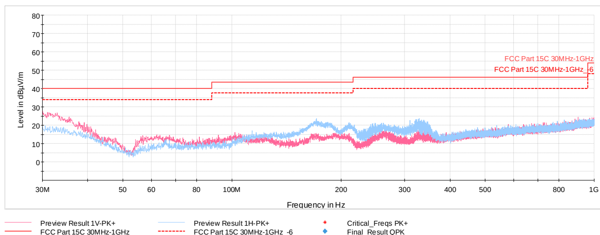
Plot 7-38. Radiated Spurious Plot below 1GHz GFSK ePA – Ch.39, with WCP + AC/DC Adapter
