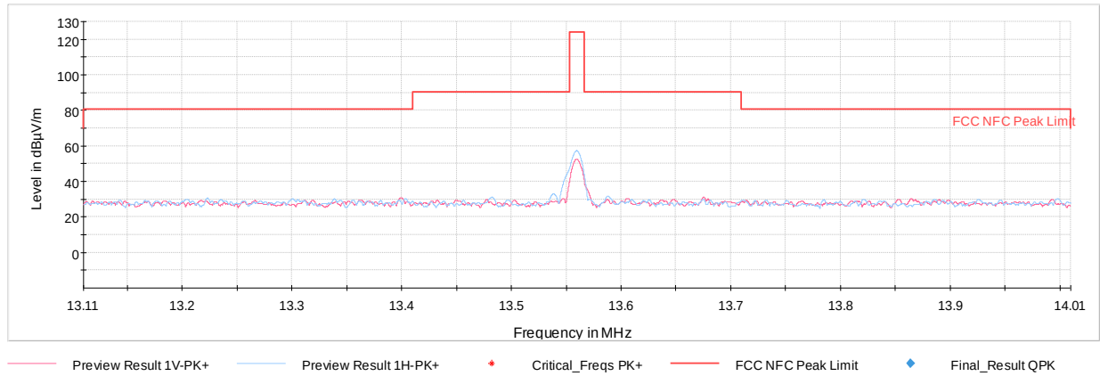
Plot 7-6. In Band Radiated Spurious Plot (CE A 848kbps)
