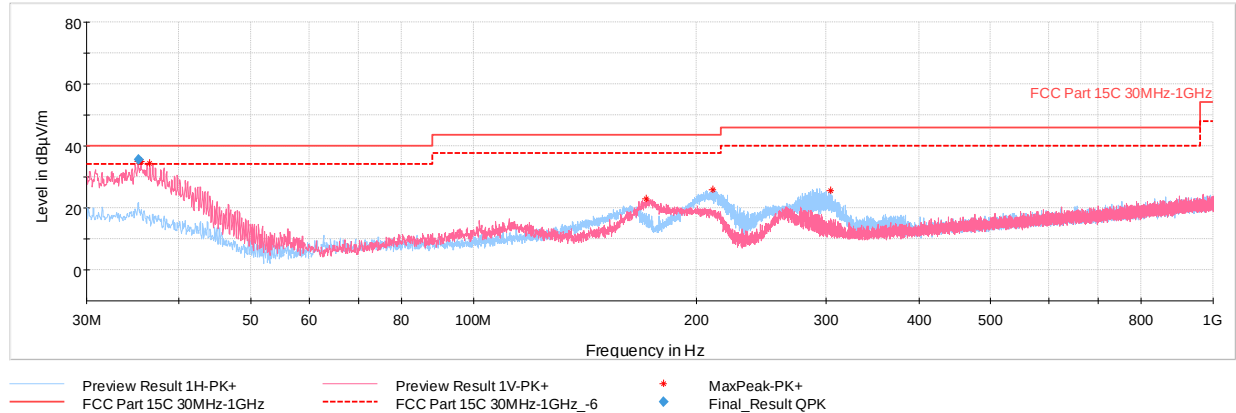
Plot 7-11. Radiated Spurious Plot 30MHz – 1GHz (Reader 10% Ask 1 out of 256, with WCP + AC/DC Adapter)
