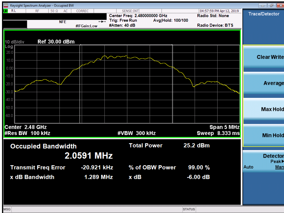
Plot 7-6. 6dB Bandwidth Plot (Bluetooth (LE), ePA – Ch. 39)
