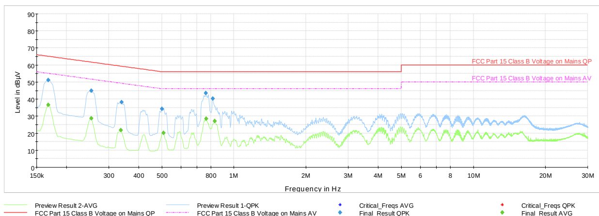
Plot 7-39. Line-Conducted Test Plot – Ch.39 (L1, with WCP + AC/DC Adapter)
