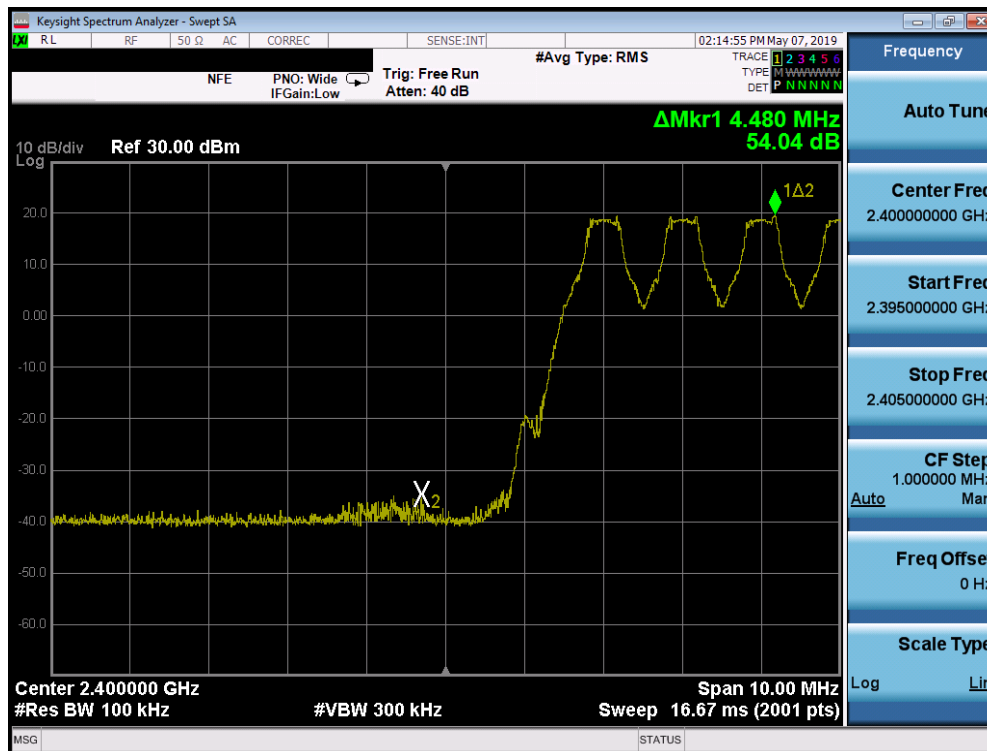
Plot 7-9. Band Edge Plot (Bluetooth with Hopping Enabled, GFSK, ePA)
