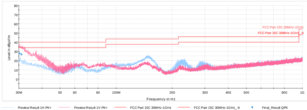
Plot 7-52. Radiated Spurious Plot below 1GHz (802.11b – Ch.6, with WCP + AC/DC Adapter)
