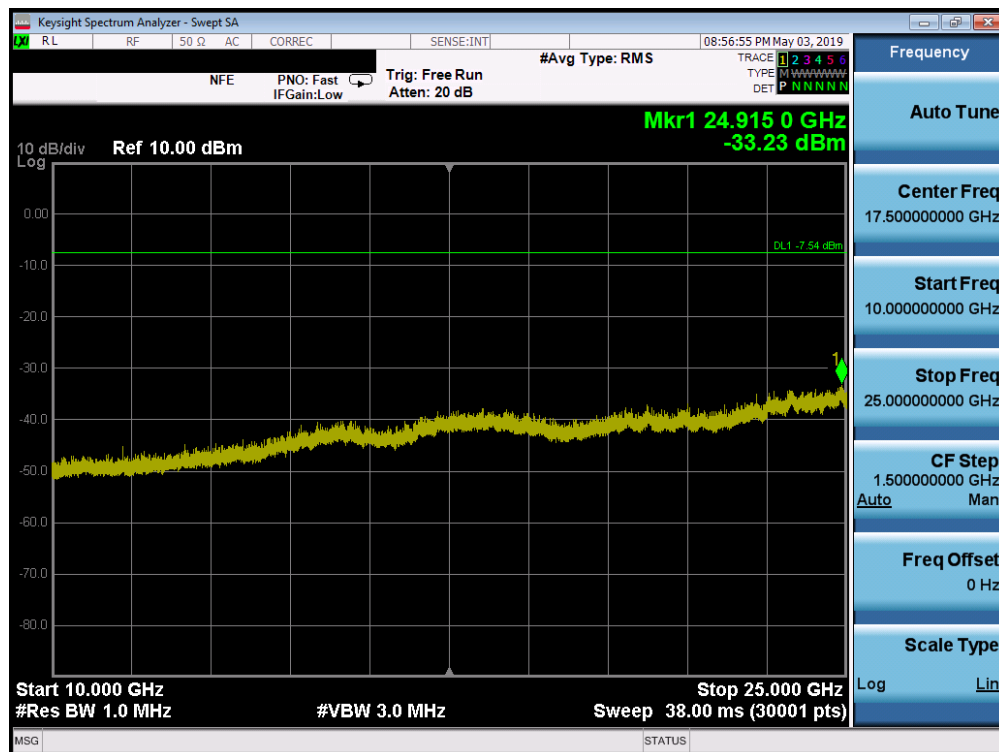
Plot 7-26. Conducted Spurious Plot (Bluetooth (HDR4), 4Mbps – Ch. 38)
