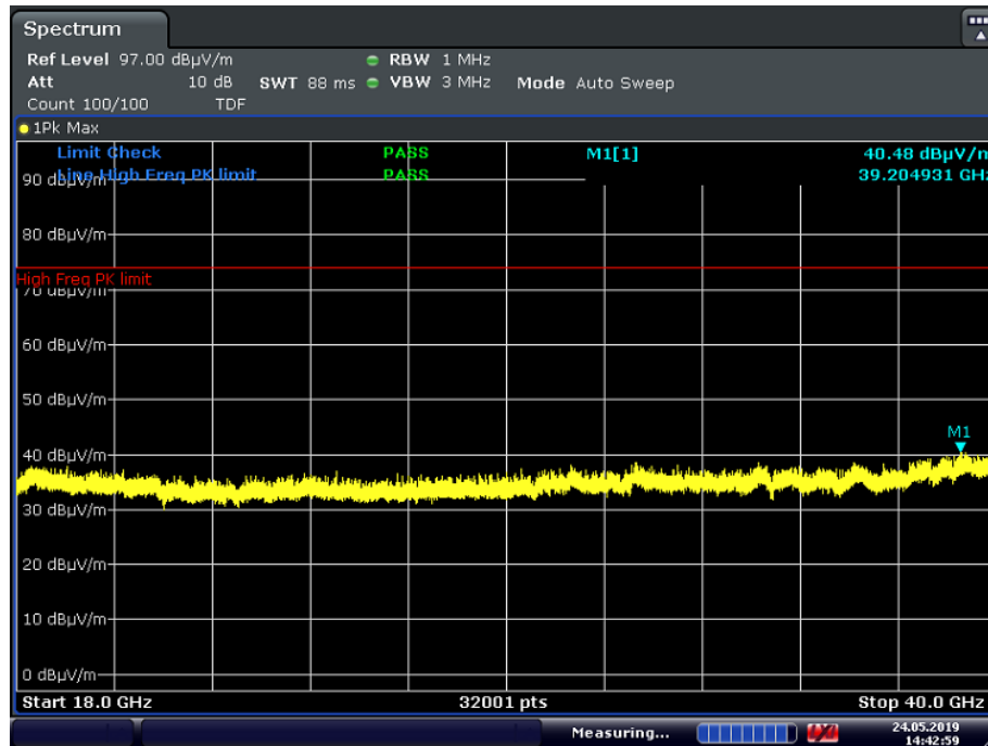
Plot 7-32. Radiated Spurious Plot Above 18GHz (4Mbps, HDR4, ePA – Ch. 38, Ant. Pol. H)
