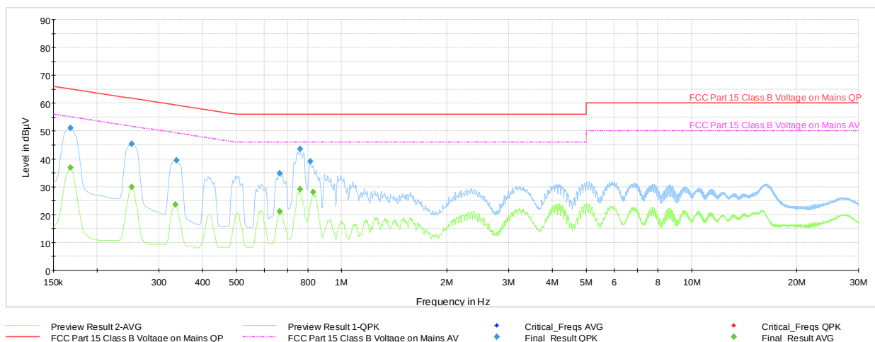
Plot 7-39. Line Conducted Plot with Bluetooth HDR (L1- 4Mbps, ePA, Ch.38 with WCP + AC/DC Adapter)
