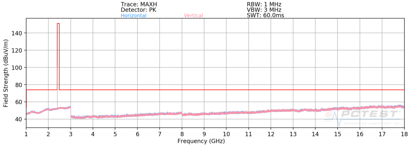
Plot 7-29. Radiated Spurious Plot Above 1GHz (4Mbps, HDR4, ePA – Ch. 1, Ant. Pol. H & V)
