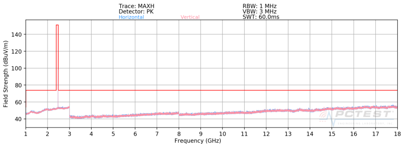
Plot 7-31. Radiated Spurious Plot Above 1GHz (4Mbps, HDR4, ePA – Ch. 75, Ant. Pol. H & V)
