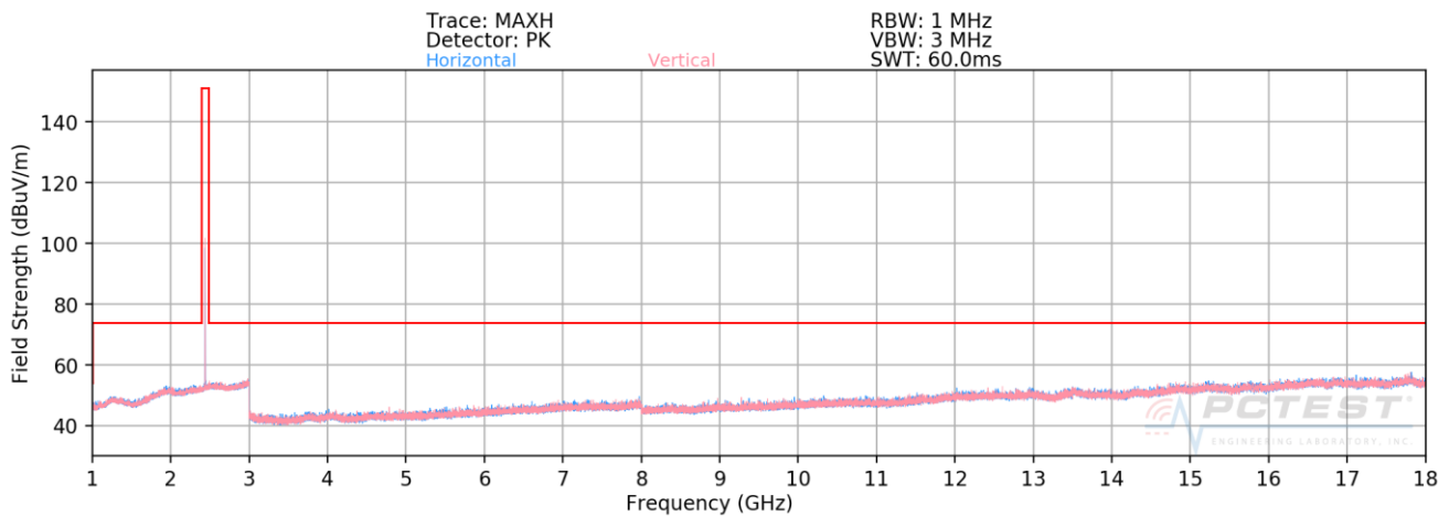
Plot 7-30. Radiated Spurious Plot Above 1GHz (4Mbps, HDR4, ePA – Ch. 38, Ant. Pol. H & V)
