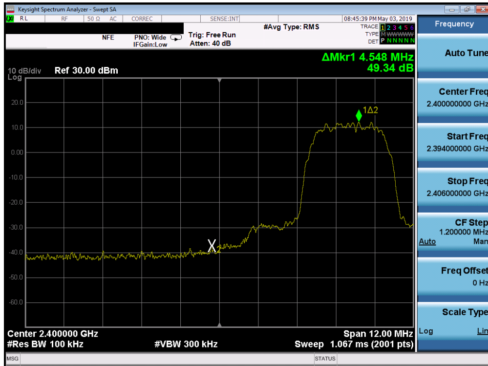
Plot 7-19. Band Edge Plot (Bluetooth (HDR4), ePA – Ch. 1)
