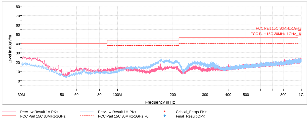
Plot 7-38. Radiated Spurious Plot below 1GHz (4Mbps, ePA – Ch.38 with WCP + AC/DC Adapter attached)
