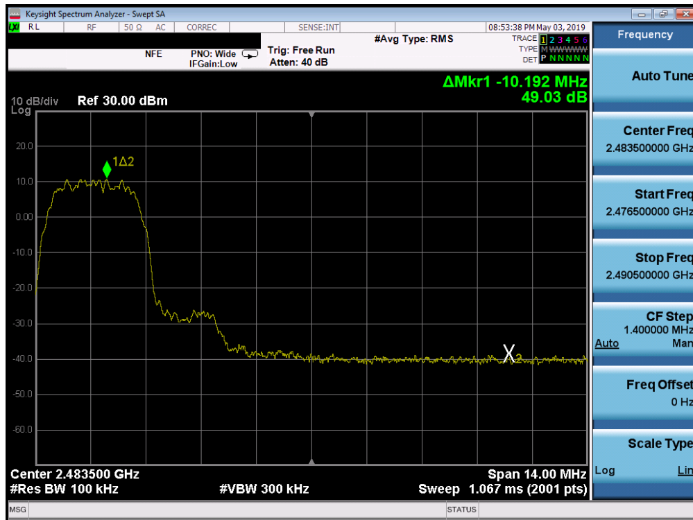
Plot 7-20. Band Edge Plot (Bluetooth (HDR4), ePA – Ch. 75)
