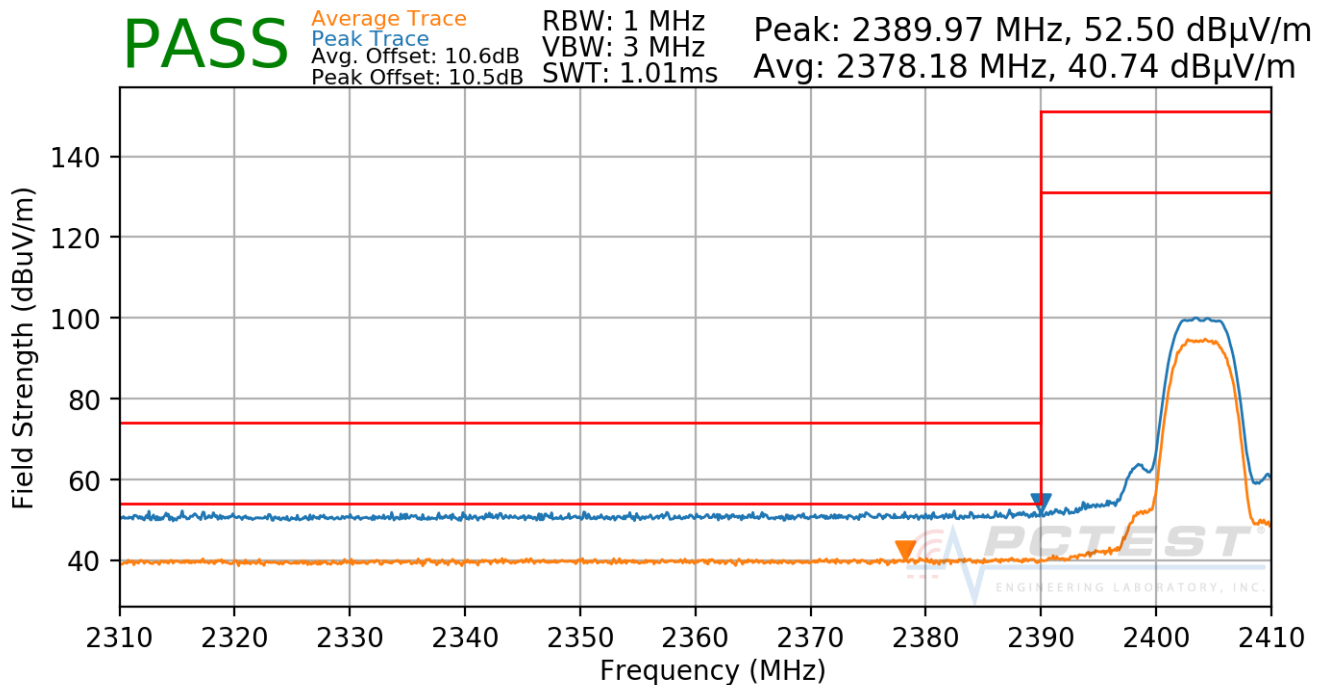
Plot 7-35. Radiated Restricted Lower Band Edge Measurement (Average & Peak)
