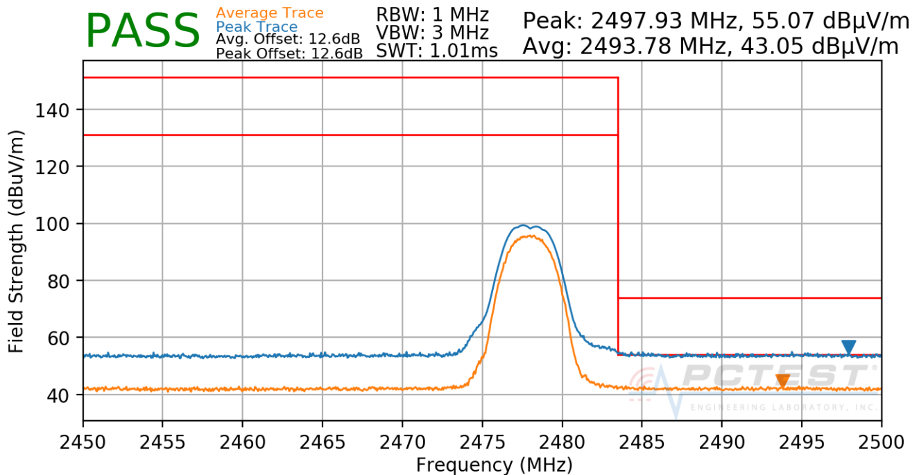
Plot 7-36. Radiated Restricted Upper Band Edge Measurement (Average & Peak)
