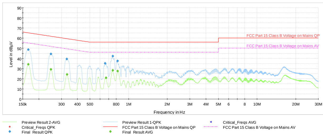
Plot 7-40. Line Conducted Plot with Bluetooth HDR (N- 4Mbps, ePA, Ch.38 with WCP + AC/DC Adapter)
