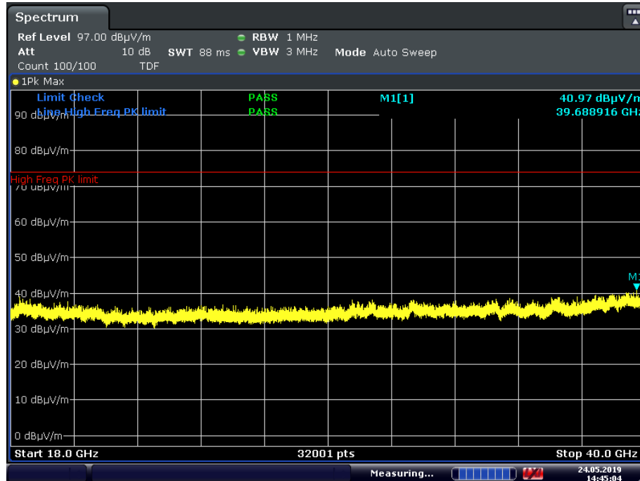
Plot 7-33. Radiated Spurious Plot Above 18GHz (4Mbps, HDR4, ePA – Ch. 38, Ant. Pol. V)
