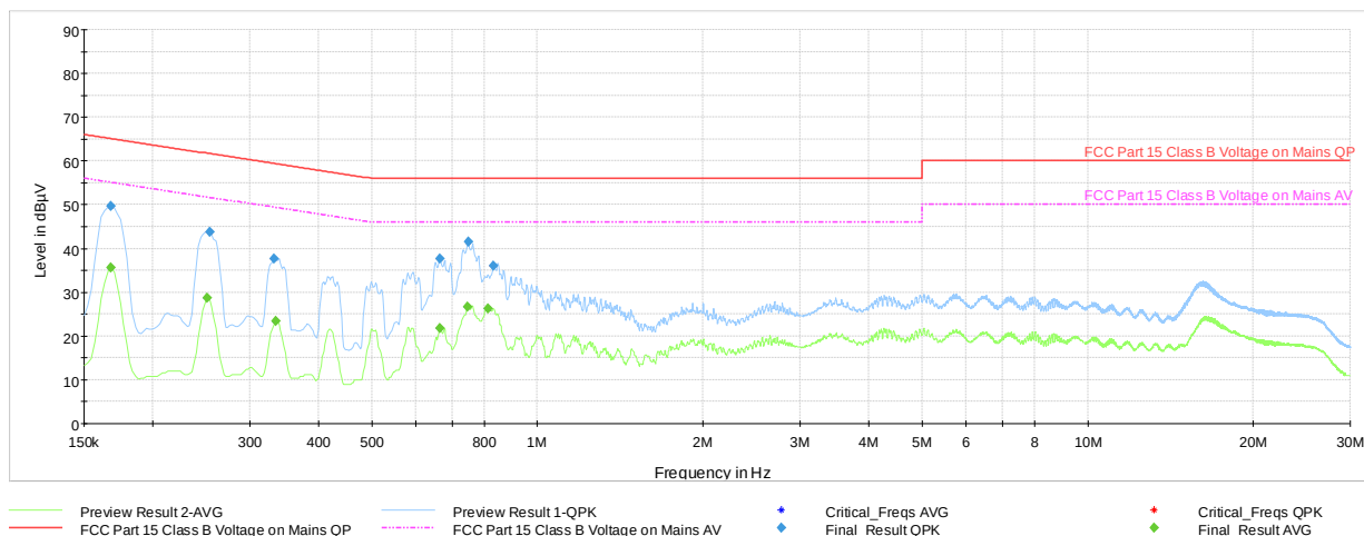
Plot 7-40. Line Conducted Plot with Bluetooth LE (N - 1Mbps, ePA, Ch.19 with WCP + AC/DC Adapter)
