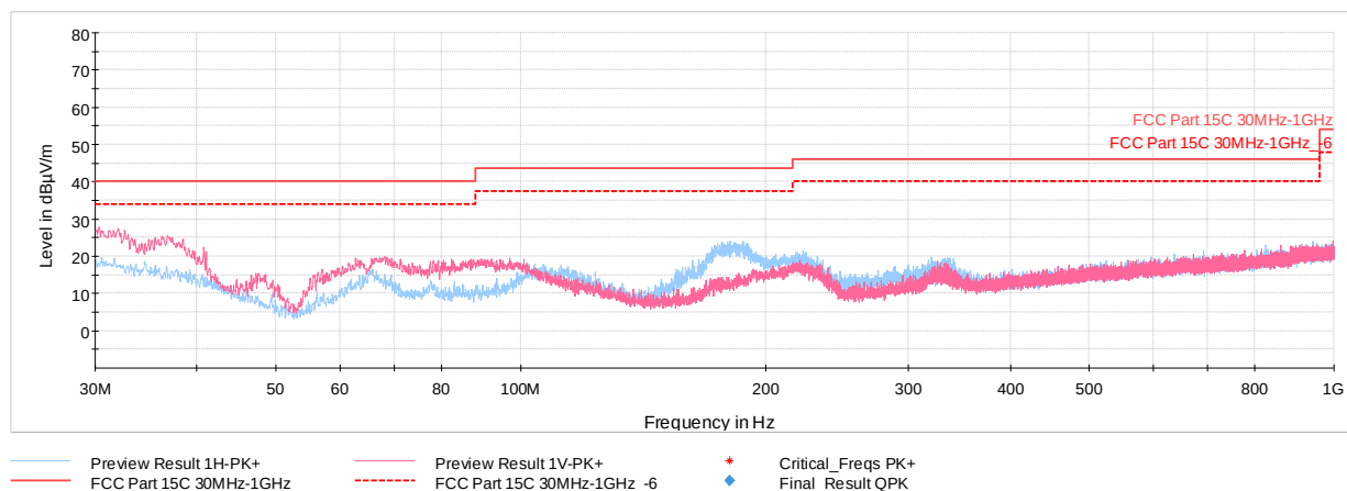
Plot 7-38. Radiated Spurious Plot below 1GHz GFSK ePA – Ch.39, with WCP + AC/DC Adapter
