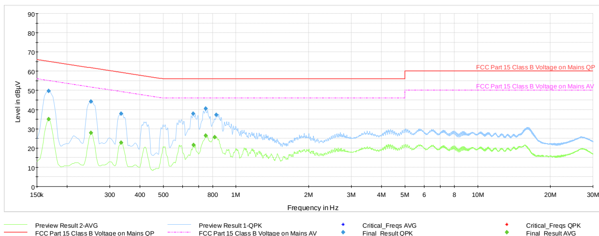
Plot 7-39. Line-Conducted Test Plot – GFSK ePA Ch.39 (L1, with WCP + AC/DC Adapter)
