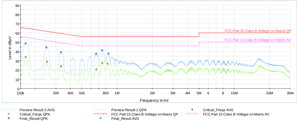
Plot 7-40. Line-Conducted Test Plot – GFSK ePA Ch.39 (N, with WCP + AC/DC Adapter)
