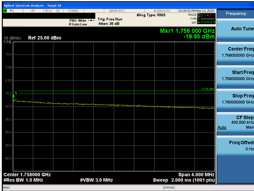
Plot 7-203. Upper Extended Band Edge Plot (Band 4 - 20.0MHz QPSK - Full RB Configuration)
