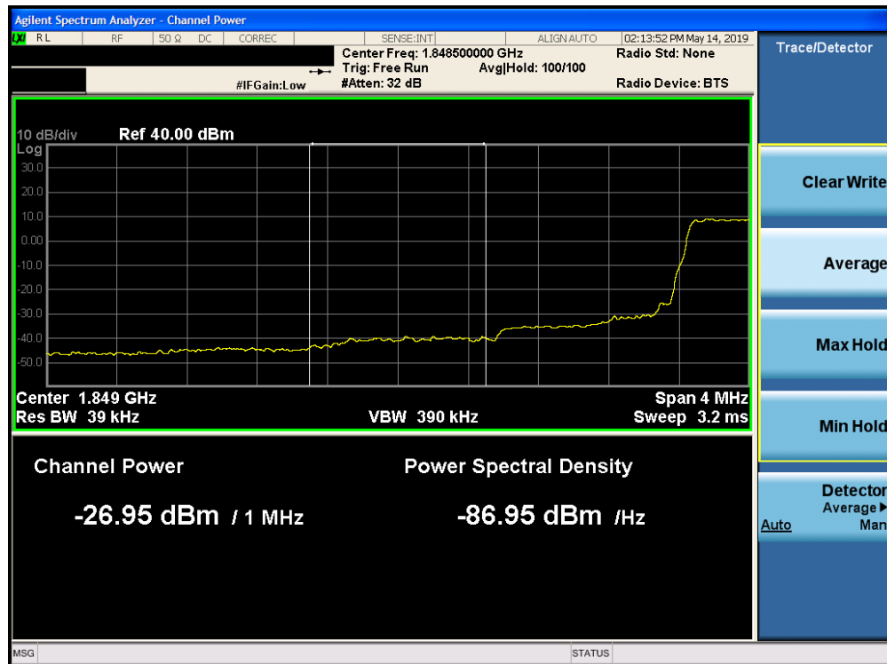
Plot 7-205. Lower Extended Band Edge Plot (Band 25 - 1.4MHz QPSK - Full RB Configuration)
