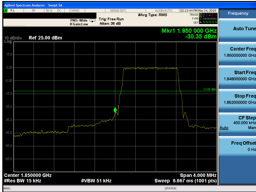
Plot 7-204. Lower Band Edge Plot (Band 25 - 1.4MHz QPSK - Full RB Configuration)
