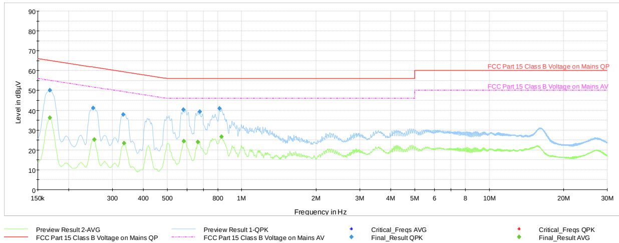
Plot 7-56. Line Conducted Plot with 802.11b Ch.6 (L1, with WCP + AC/DC Adapter)
