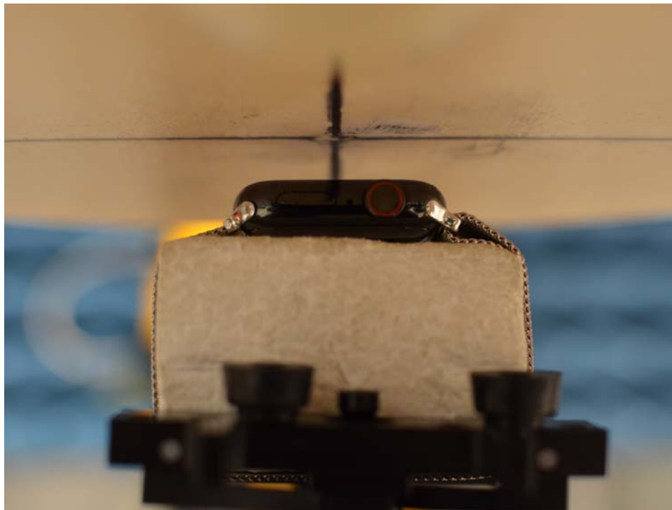
SAR Test Setup Photo 6: Stainless Steel with Metal Loop Wristband, Front side at 1.0 cm
