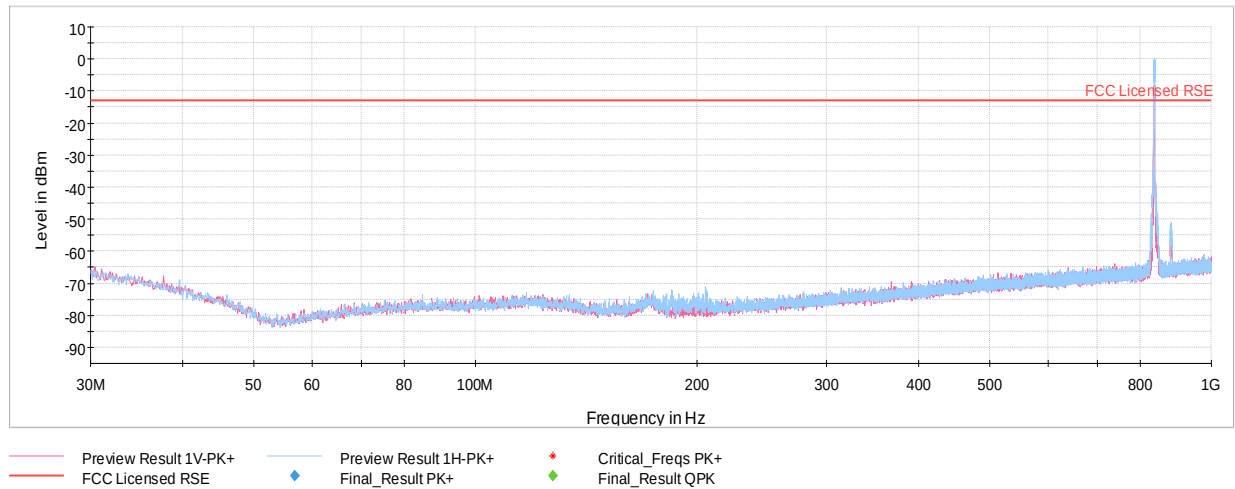
Plot 7-44. Radiated Spurious Plot Below 1GHz (Cellular WCDMA Mode – Ch. 4183)
