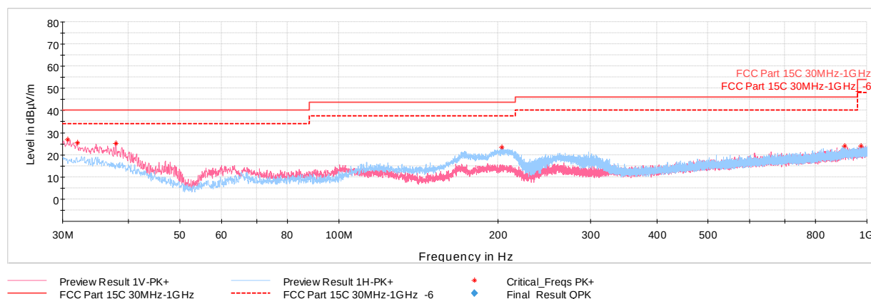
Plot 7-38. Radiated Spurious Plot below 1GHz (4Mbps, ePA – Ch.38 with WCP + AC/DC Adapter)
