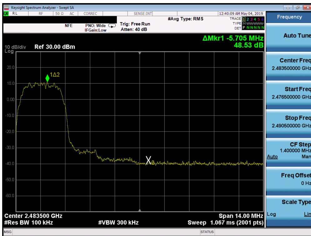
Plot 7-20. Band Edge Plot (Bluetooth (HDR4), ePA – Ch. 75)
