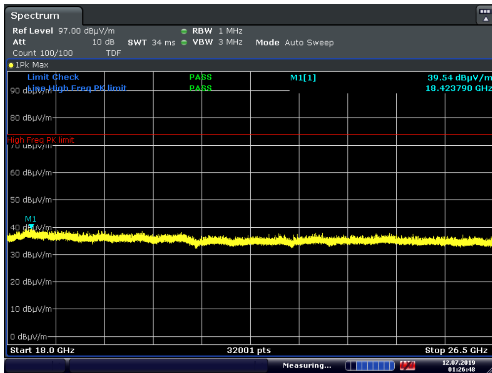
Plot 7-36. Radiated Spurious Plot Above 18GHz (Ant. Pol. V)
