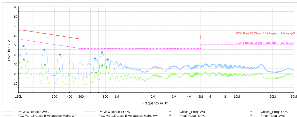
Plot 7-43. Line-Conducted Test Plot – GFSK ePA Ch.39 (L1, with WCP + AC/DC Adapter)
