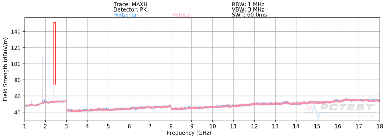
Plot 7-34. Radiated Spurious Plot above 1GHz
