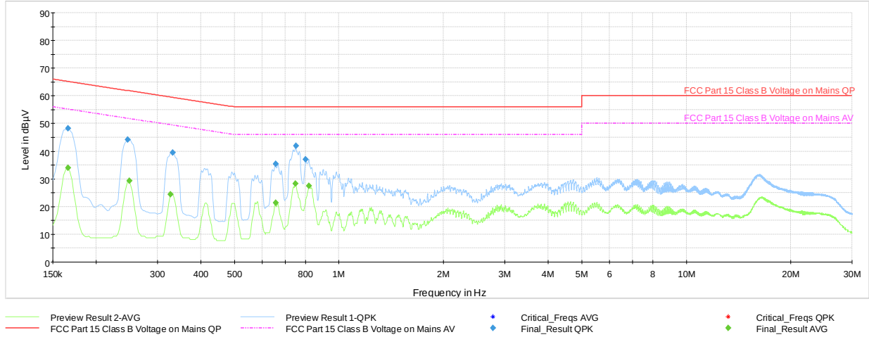
Plot 7-44. Line-Conducted Test Plot – GFSK ePA Ch.39 (N, with WCP + AC/DC Adapter)
