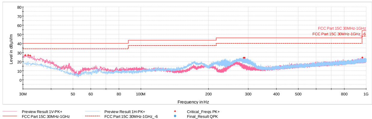
Plot 7-41. Radiated Spurious Plot below 1GHz GFSK ePA – Ch.39, with WCP + AC/DC Adapter
