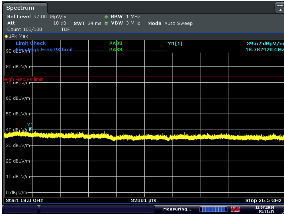
Plot 7-35. Radiated Spurious Plot Above 18GHz (Ant. Pol. H)
