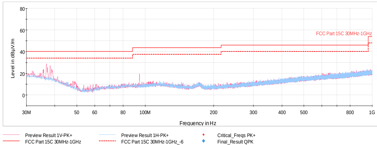
Plot 7-42. Radiated Spurious Plot Below 1GHz (with WCP + AC/DC Adapter)
