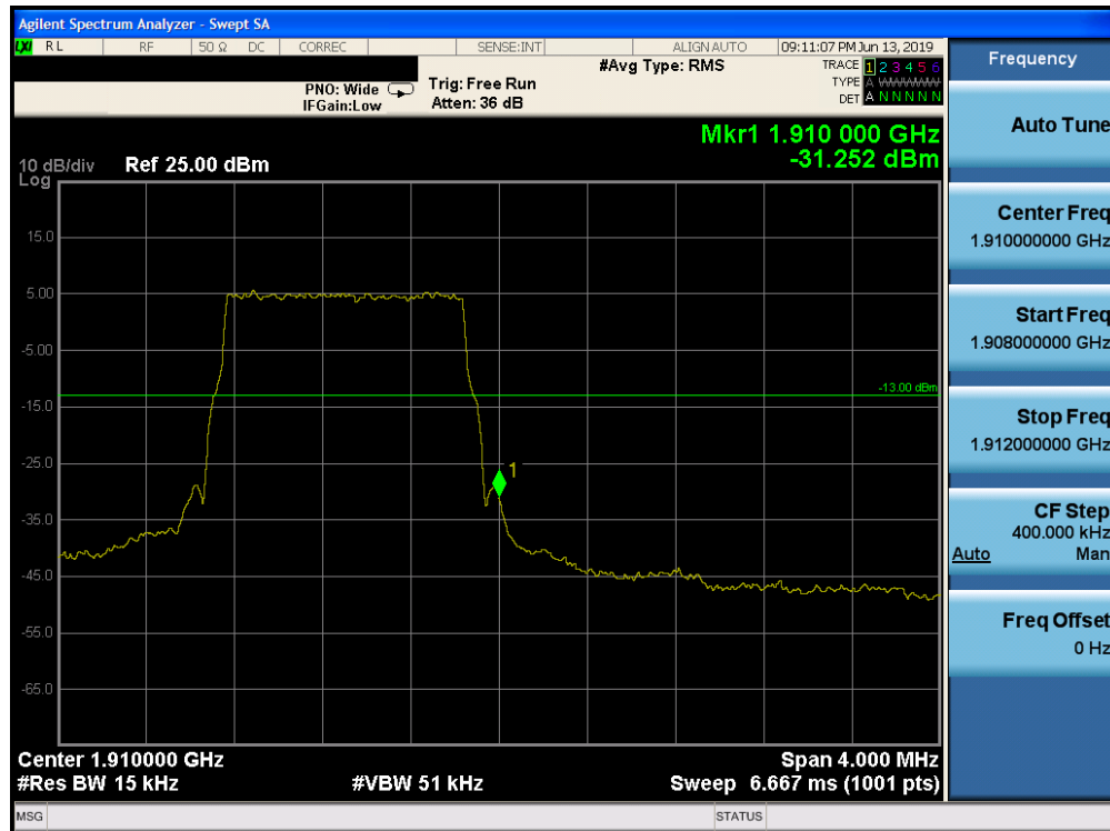
Plot 7-230. Upper Band Edge Plot (Band 2 - 1.4.0MHz QPSK - Full RB Configuration)
