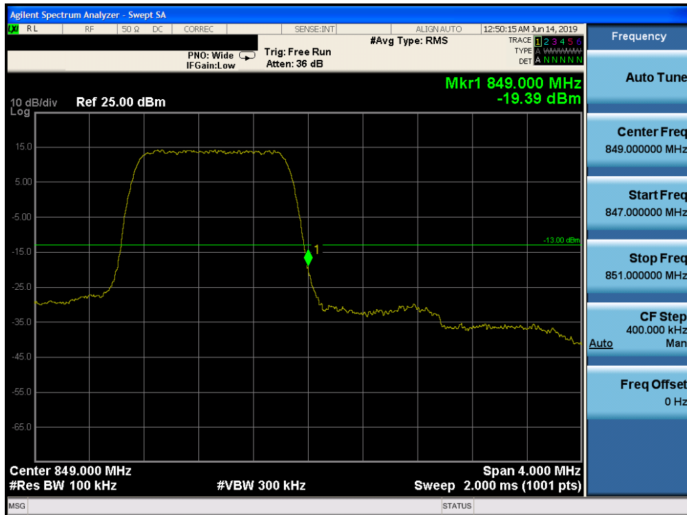
Plot 7-149. Upper Band Edge Plot (Band 5 - 1.4.0MHz QPSK - Full RB Configuration)
