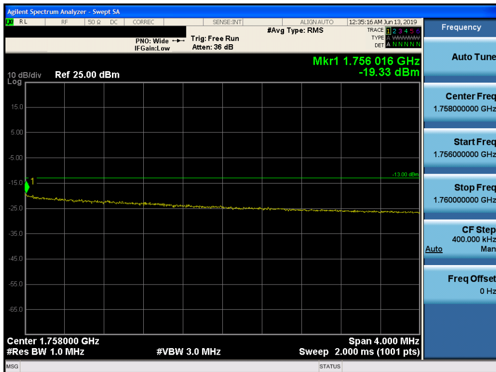
Plot 7-195. Upper Extended Band Edge Plot (Band 4 - 10.0MHz QPSK - Full RB Configuration)
