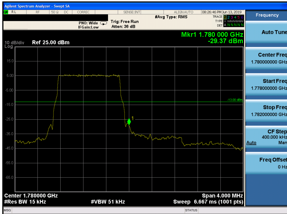
Plot 7-158. Upper Band Edge Plot (Band 66 - 1.4.0MHz QPSK - Full RB Configuration)
