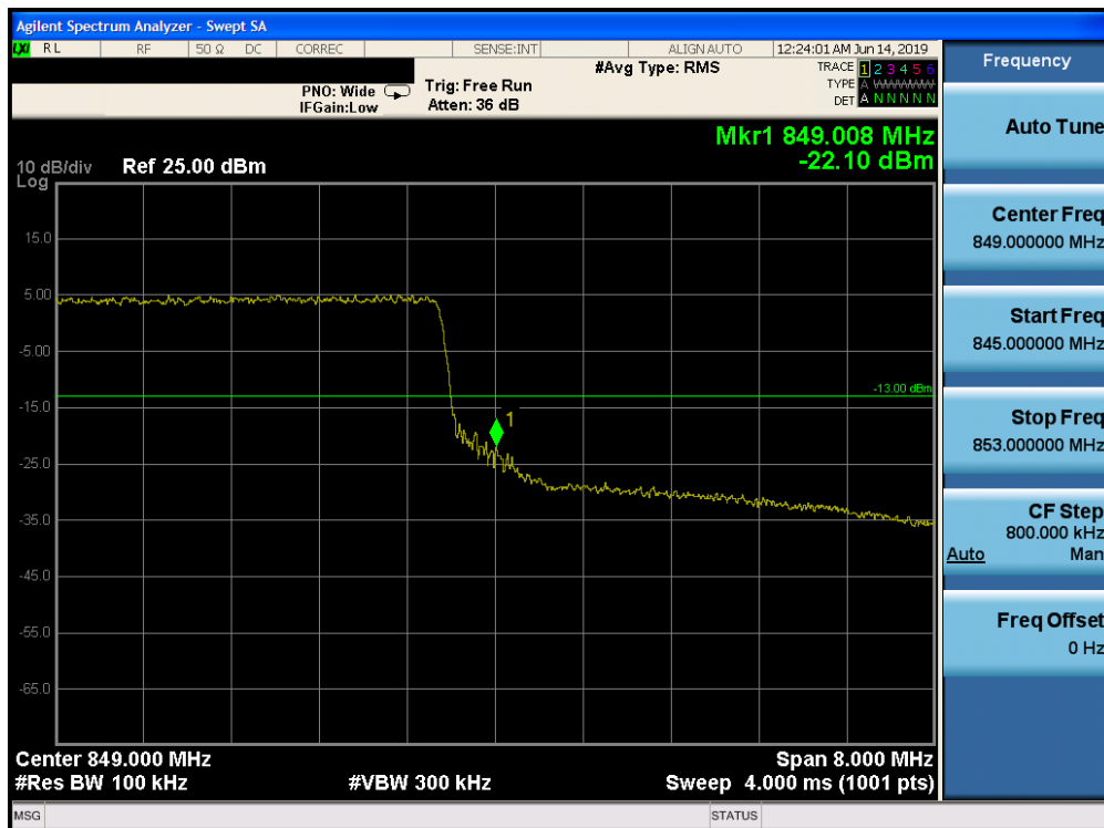
Plot 7-155. Upper Band Edge Plot (Band 5 - 10.0MHz QPSK - Full RB Configuration)
