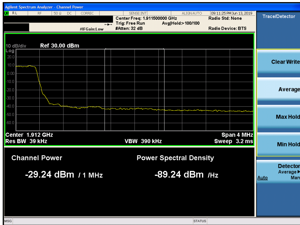
Plot 7-231. Upper Extended Band Edge Plot (Band 2 - 1.4.0MHz QPSK - Full RB Configuration)
