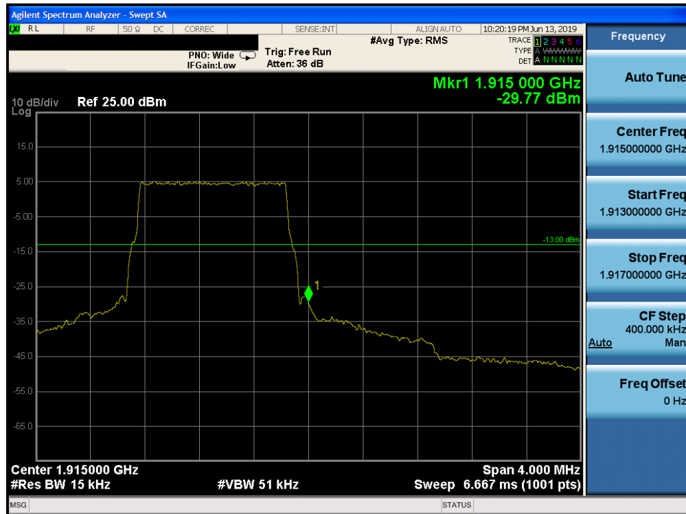
Plot 7-206. Upper Band Edge Plot (Band 25 - 1.4.0MHz QPSK - Full RB Configuration)
