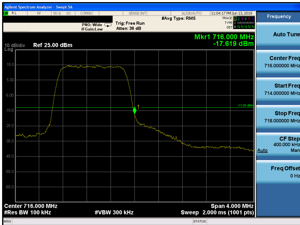
Plot 7-125. Upper Band Edge Plot (Band 12 - 1.4.0MHz QPSK - Full RB Configuration)
