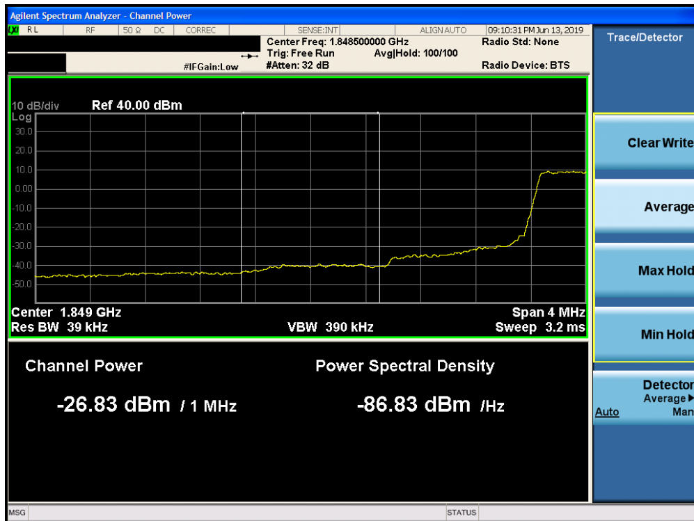
Plot 7-229. Lower Extended Band Edge Plot (Band 2 - 1.4.0MHz QPSK - Full RB Configuration)
