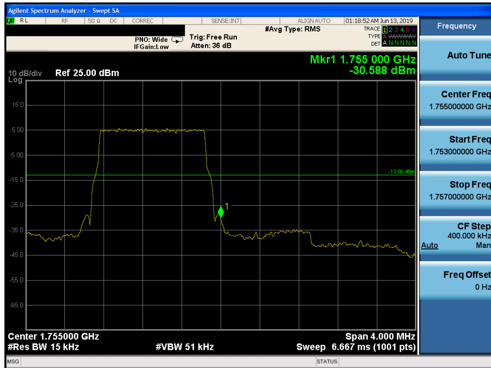
Plot 7-182. Upper Band Edge Plot (Band 4 - 1.4.0MHz QPSK - Full RB Configuration)
