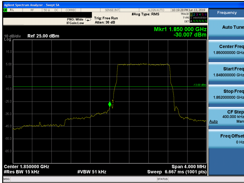
Plot 7-204. Lower Band Edge Plot (Band 25 - 1.4.0MHz QPSK - Full RB Configuration)
