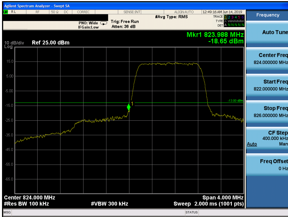
Plot 7-148. Lower Band Edge Plot (Band 5 - 1.4.0MHz QPSK - Full RB Configuration)
