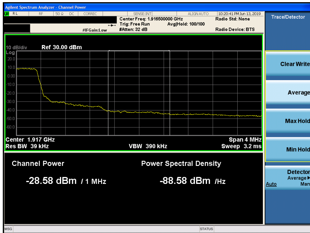
Plot 7-207. Upper Extended Band Edge Plot (Band 25 - 1.4.0MHz QPSK - Full RB Configuration)
