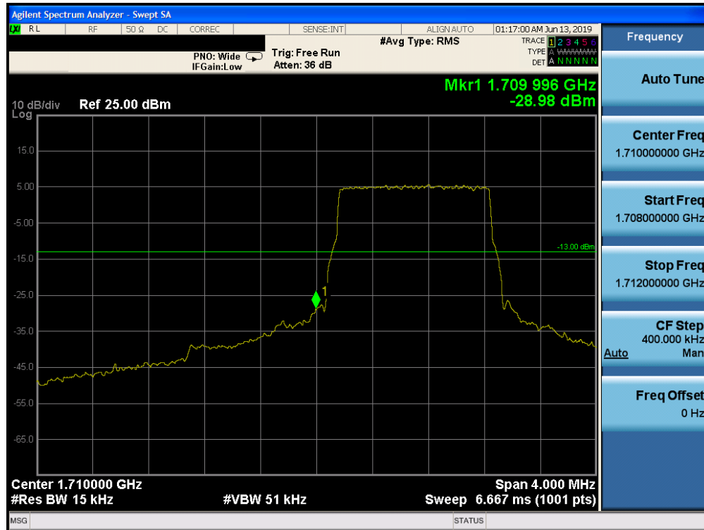
Plot 7-180. Lower Band Edge Plot (Band 4 - 1.4.0MHz QPSK - Full RB Configuration)
