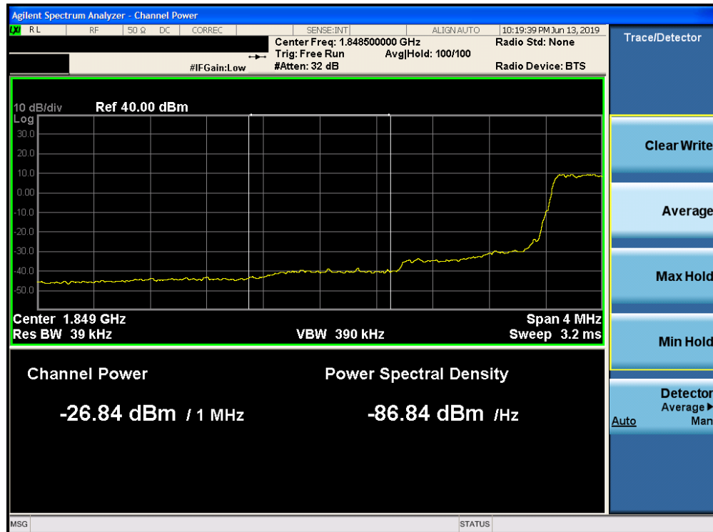
Plot 7-205. Lower Extended Band Edge Plot (Band 25 - 1.4.0MHz QPSK - Full RB Configuration)
