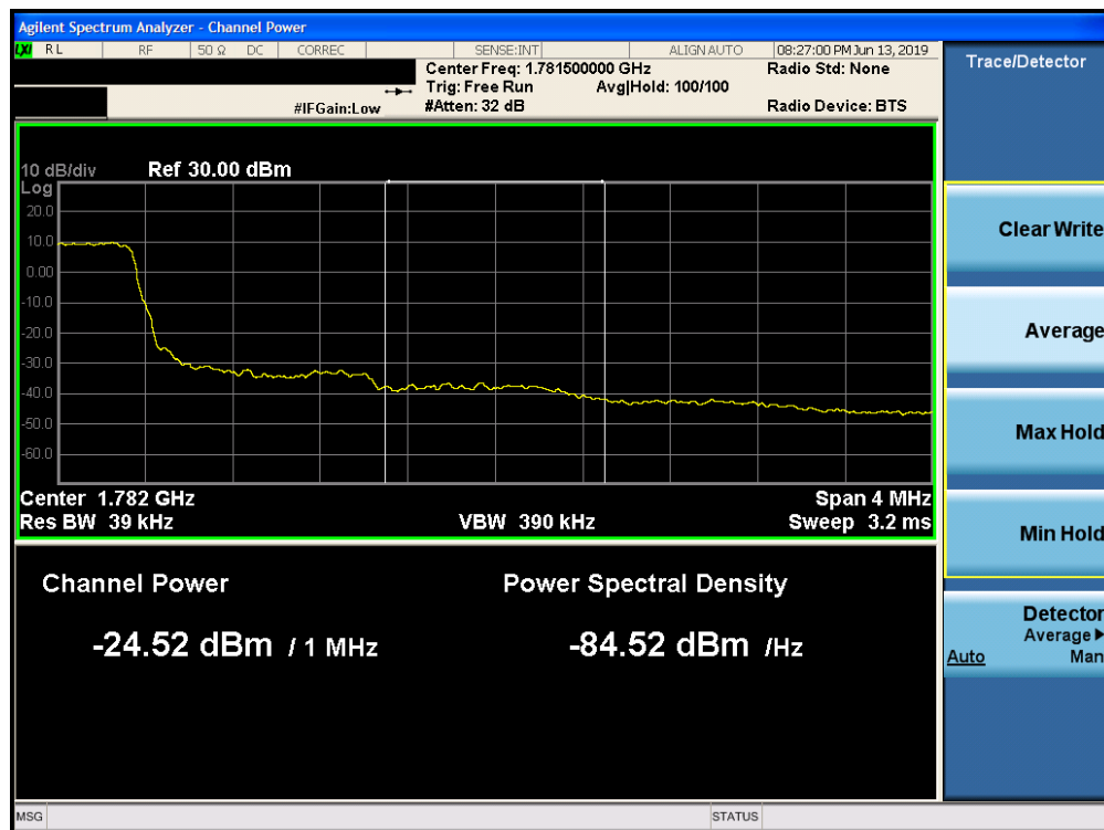
Plot 7-159. Upper Extended Band Edge Plot (Band 66 - 1.4.0MHz QPSK - Full RB Configuration)
