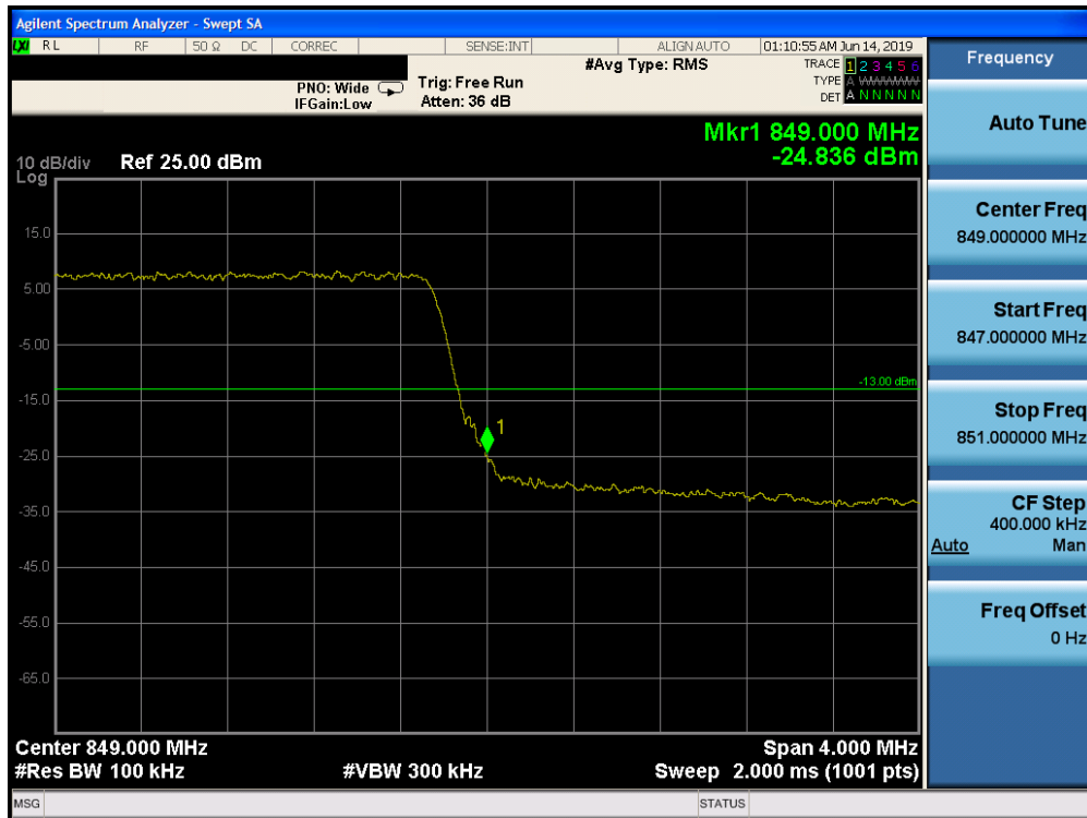
Plot 7-145. Upper Band Edge Plot (Band 26 - 5.0MHz QPSK - Full RB Configuration)
