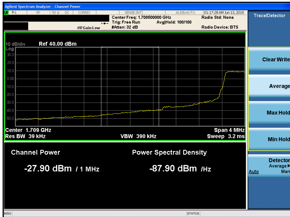
Plot 7-181. Lower Extended Band Edge Plot (Band 4 - 1.4.0MHz QPSK - Full RB Configuration)
