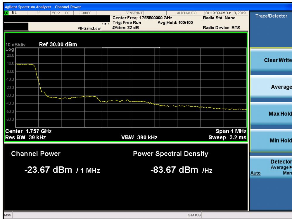
Plot 7-183. Upper Extended Band Edge Plot (Band 4 - 1.4.0MHz QPSK - Full RB Configuration)
