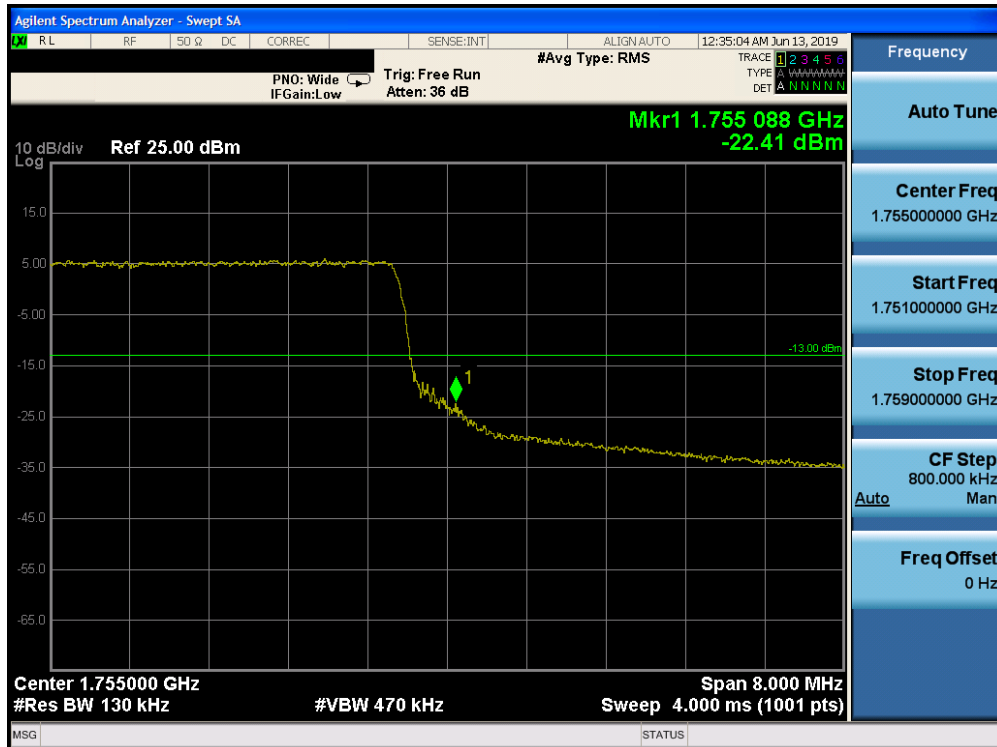
Plot 7-194. Upper Band Edge Plot (Band 4 - 10.0MHz QPSK - Full RB Configuration)
