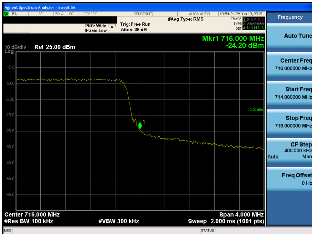
Plot 7-129. Upper Band Edge Plot (Band 12 - 5.0MHz QPSK - Full RB Configuration)
