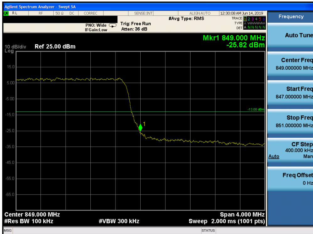
Plot 7-153. Upper Band Edge Plot (Band 5 - 5.0MHz QPSK - Full RB Configuration)
