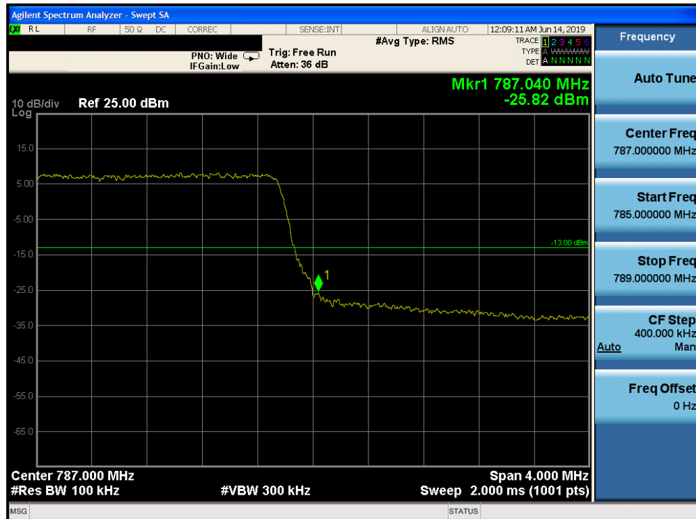
Plot 7-137. Upper Band Edge Plot (Band 13 - 5.0MHz QPSK - Full RB Configuration)
