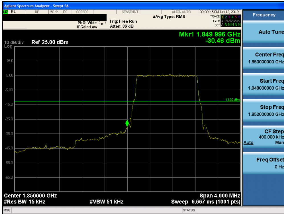
Plot 7-228. Lower Band Edge Plot (Band 2 - 1.4.0MHz QPSK - Full RB Configuration)
