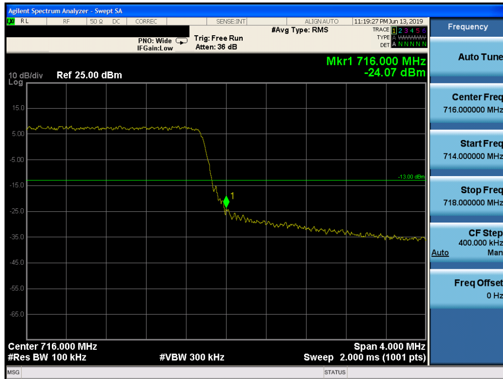
Plot 7-133. Upper Band Edge Plot (Band 17 - 5.0MHz QPSK - Full RB Configuration)
