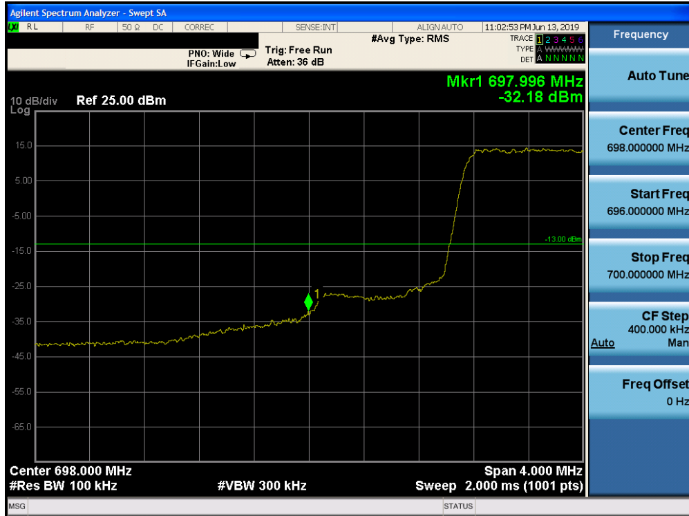
Plot 7-124. Lower Band Edge Plot (Band 12 - 1.4.0MHz QPSK - Full RB Configuration)
