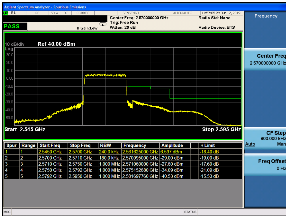
Plot 7-255. Upper ACP Plot (Band 7 - 10.0MHz QPSK - Full RB Configuration)
