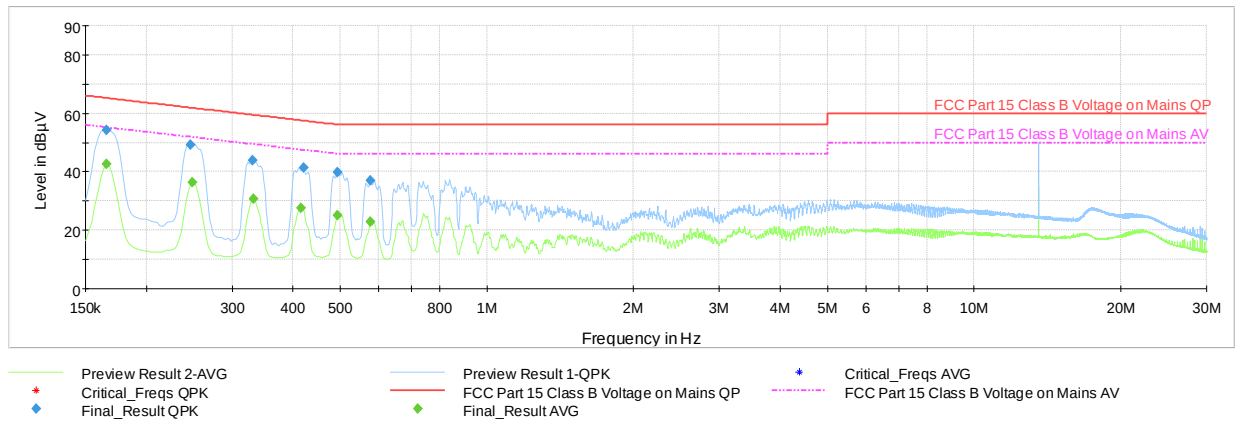
Plot 7-12. Line-Conducted Test Plot (L1, with WCP + AC/DC Adapter attached)
