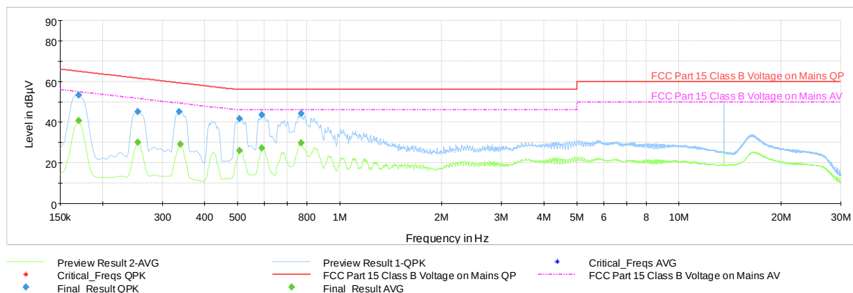
Plot 7-13. Line-Conducted Test Plot (N, with WCP + AC/DC Adapter attached)
