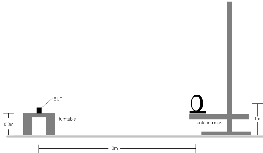
Figure 7-5. Radiated Test Setup
