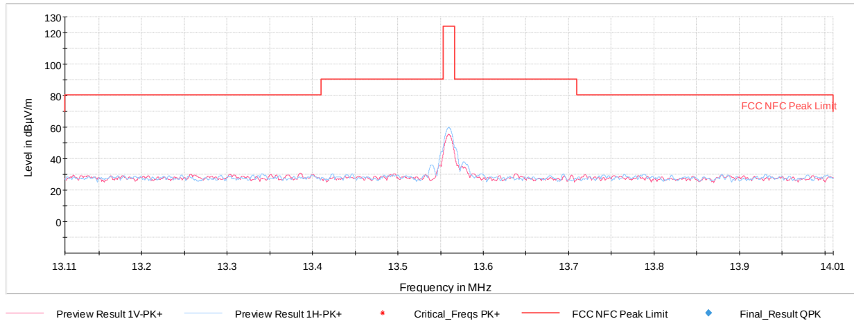
Plot 7-6. In Band Radiated Spurious Plot (CE A 848kbps)
