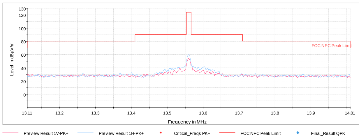
Plot 7-7. In Band Radiated Spurious Plot (Reader 10% Ask 1 out of 256)
