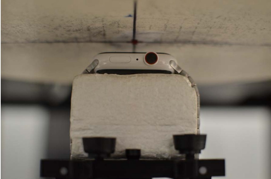
SAR Test Setup Photo 11: Ceramic with Metal Links Wristband, Front side at 1.0 cm
