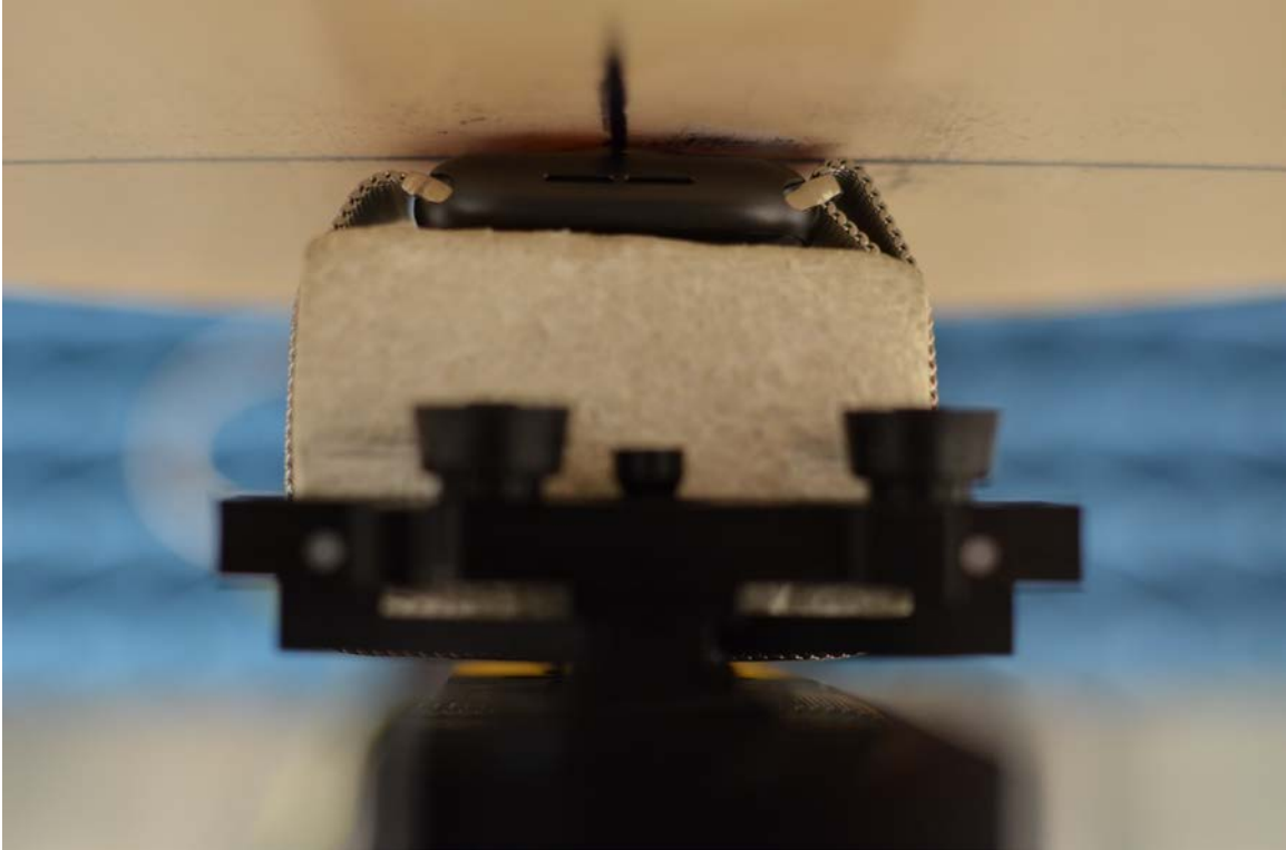
SAR Test Setup Photo 15: Aluminum with Metal Loop Wristband, Back side at 0.0 cm
