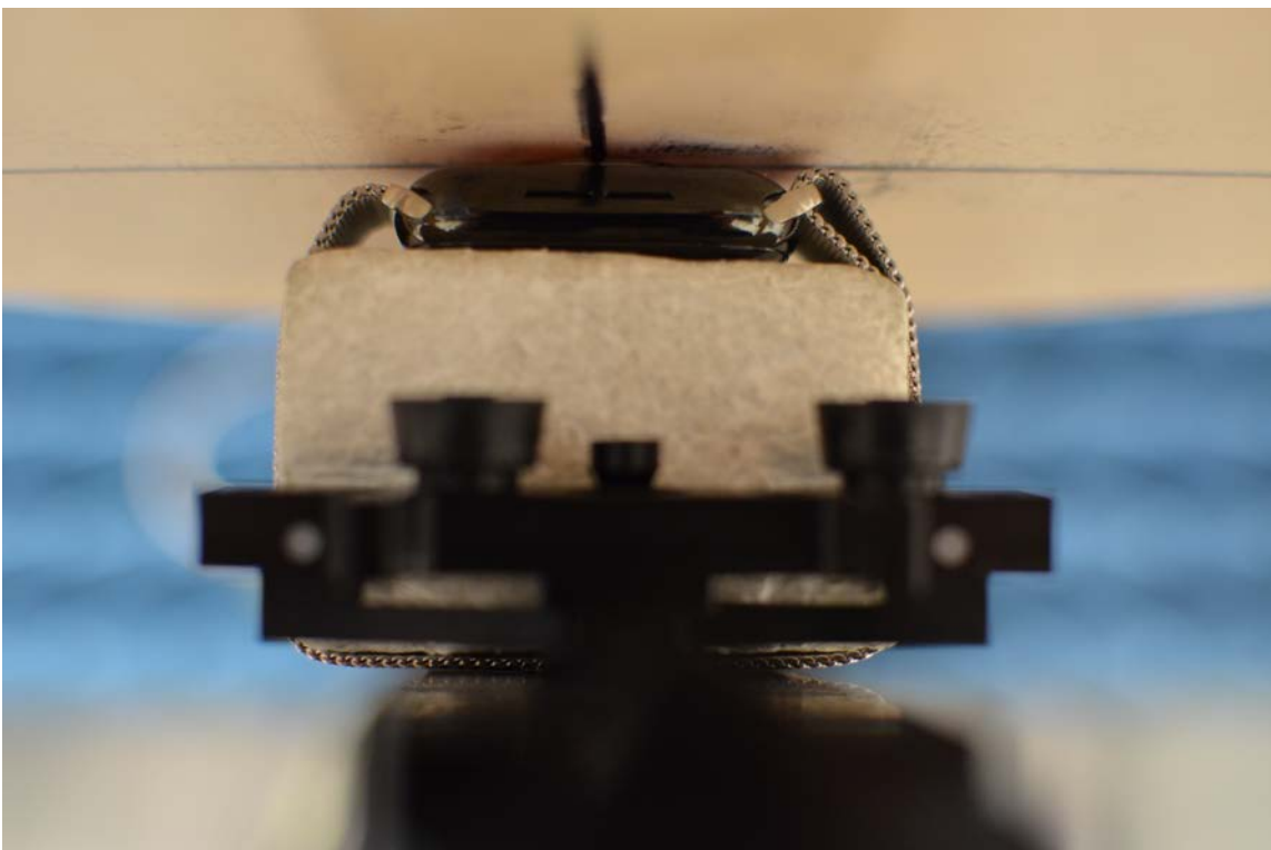
SAR Test Setup Photo 18: Stainless Steel with Metal Loop Wristband, Back side at 0.0 cm
