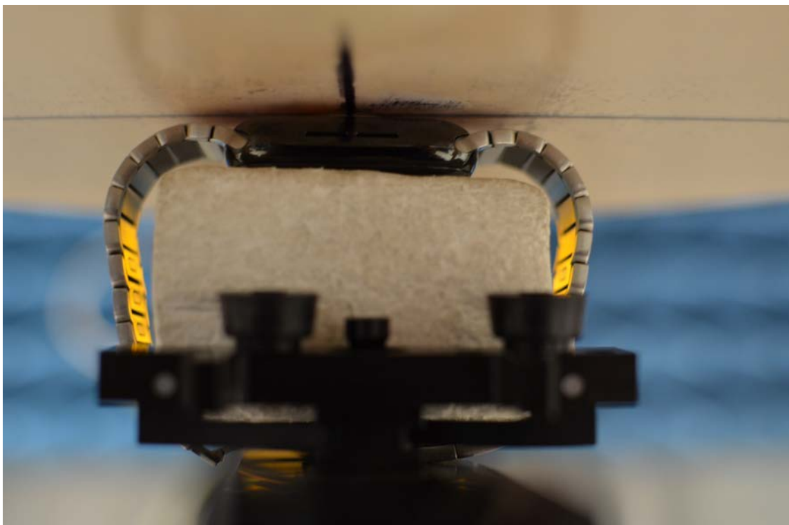
SAR Test Setup Photo 17: Stainless Steel with Metal Links Wristband, Back side at 0.0 cm
