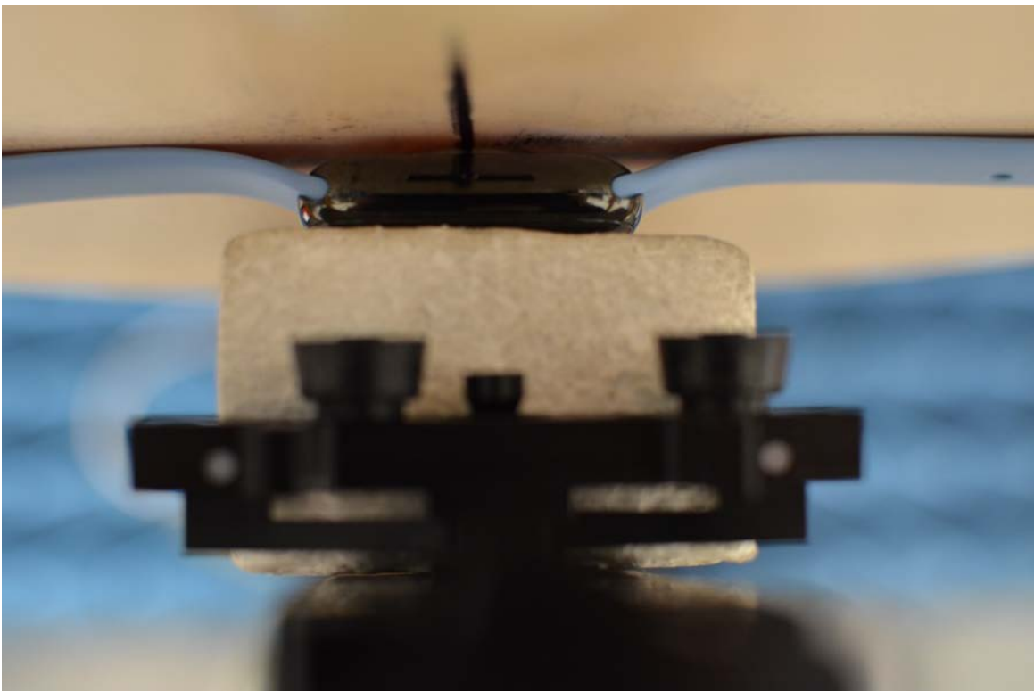
SAR Test Setup Photo 16: Stainless Steel with Sport Wristband, Back side at 0.0 cm
