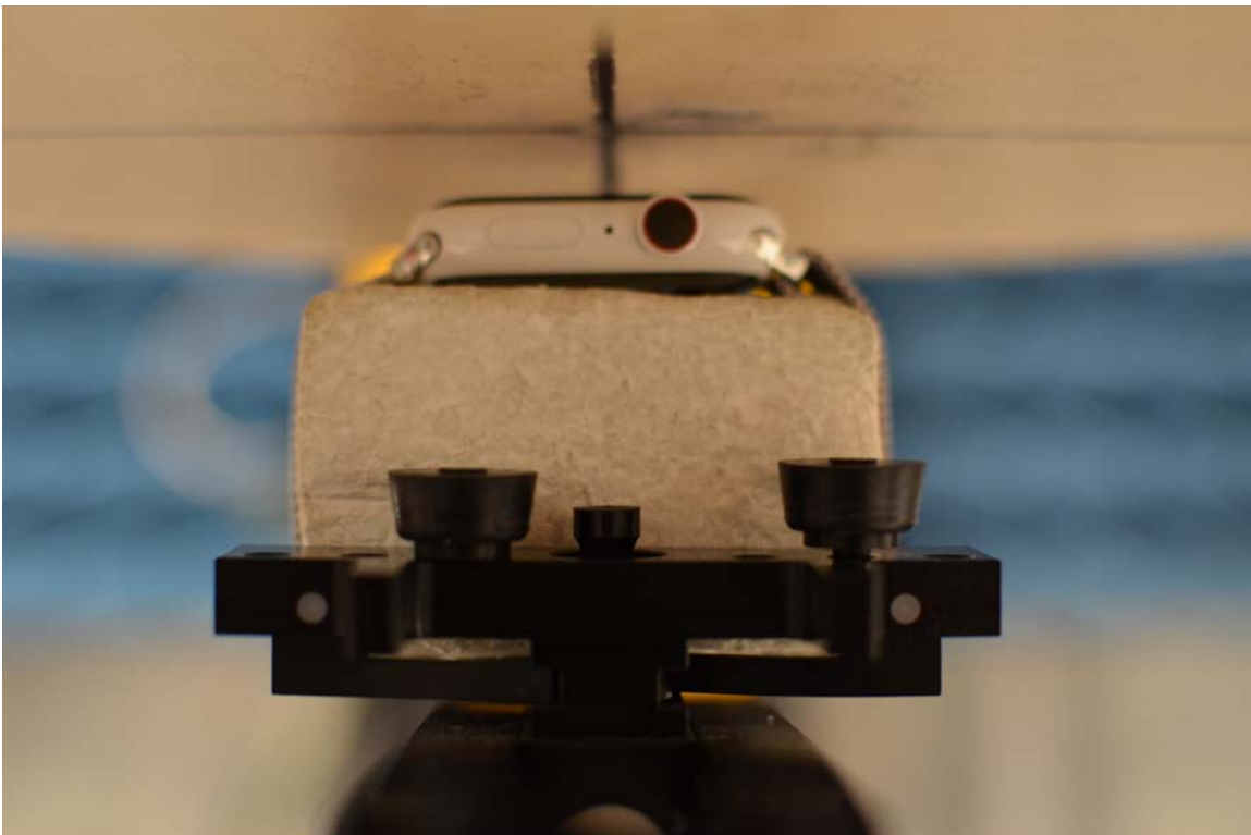
SAR Test Setup Photo 12: Ceramic with Metal Loop Wristband, Front side at 1.0 cm
