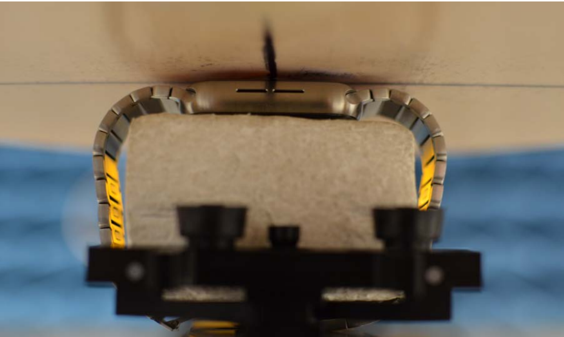
SAR Test Setup Photo 20: Titanium with Metal Links Wristband, Back side at 0.0 cm
