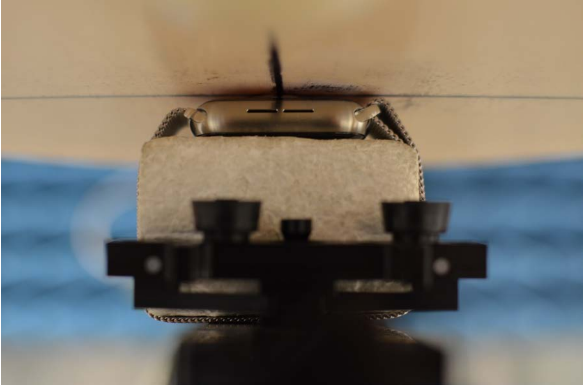
SAR Test Setup Photo 21: Titanium with Metal Loop Wristband, Back side at 0.0 cm
