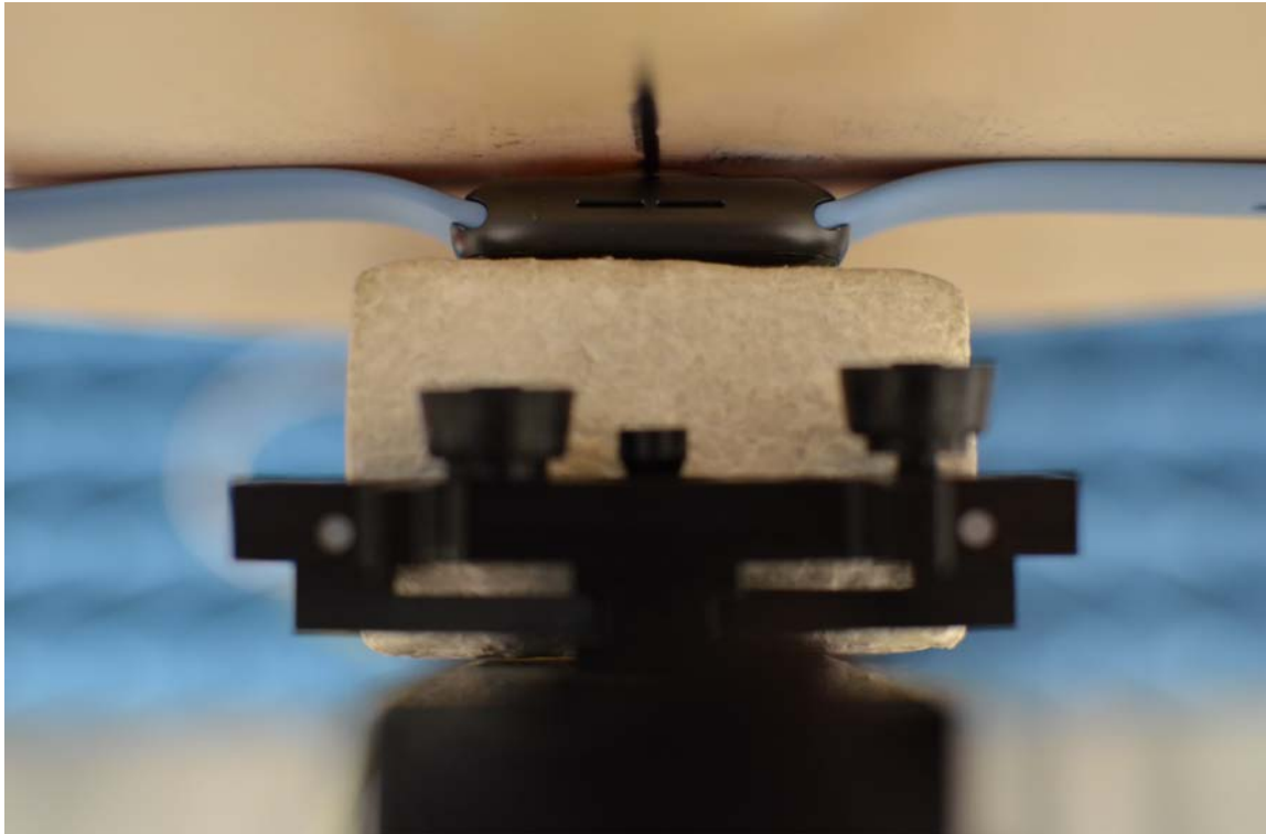
SAR Test Setup Photo 13: Aluminum with Sport Wristband, Back side at 0.0 cm
