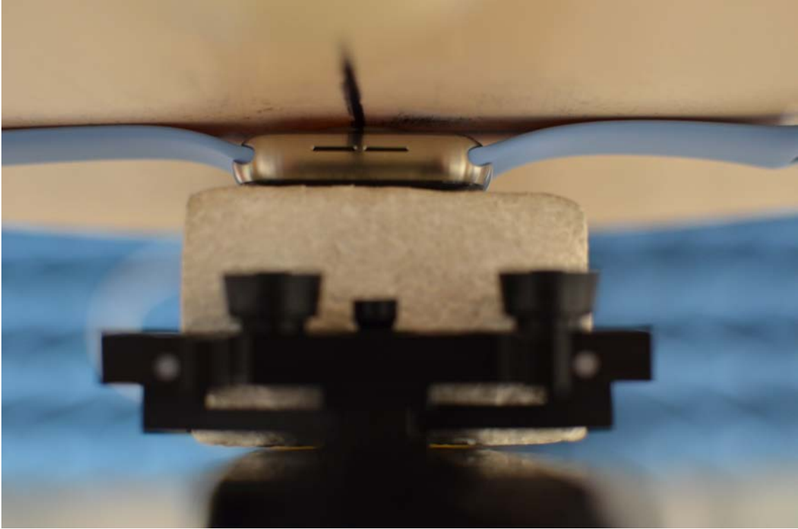
SAR Test Setup Photo 19: Titanium with Sport Wristband, Back side at 0.0 cm
