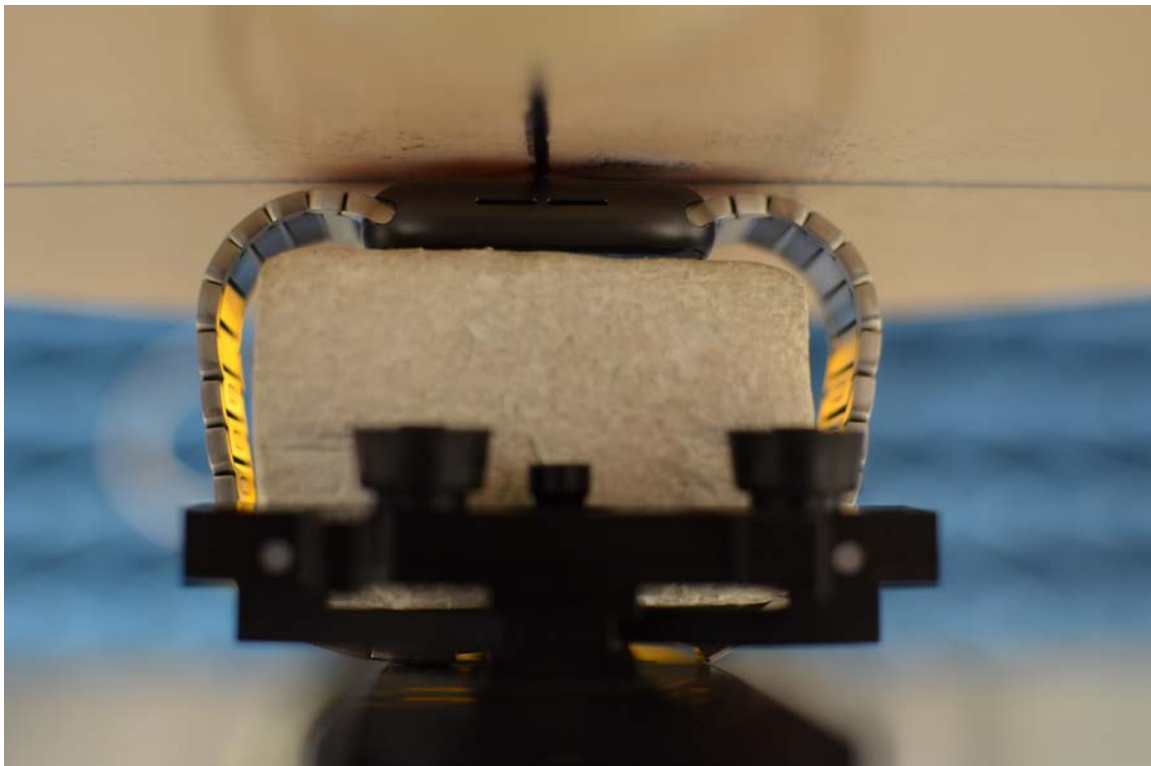
SAR Test Setup Photo 14: Aluminum with Metal Links Wristband, Back side at 0.0 cm
