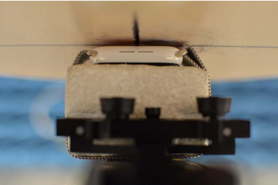
SAR Test Setup Photo 24: Ceramic with Metal Loop Wristband, Back side at 0.0 cm
