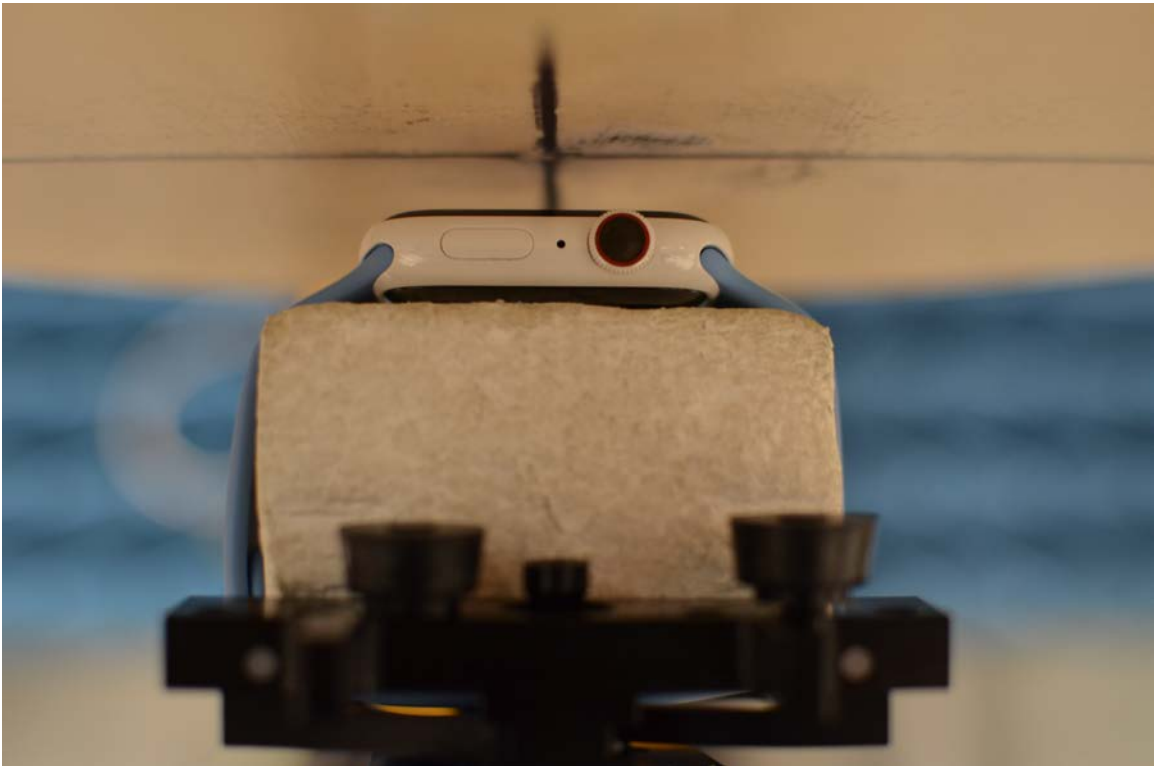
SAR Test Setup Photo 10: Ceramic with Sport Wristband, Front side at 1.0 cm
