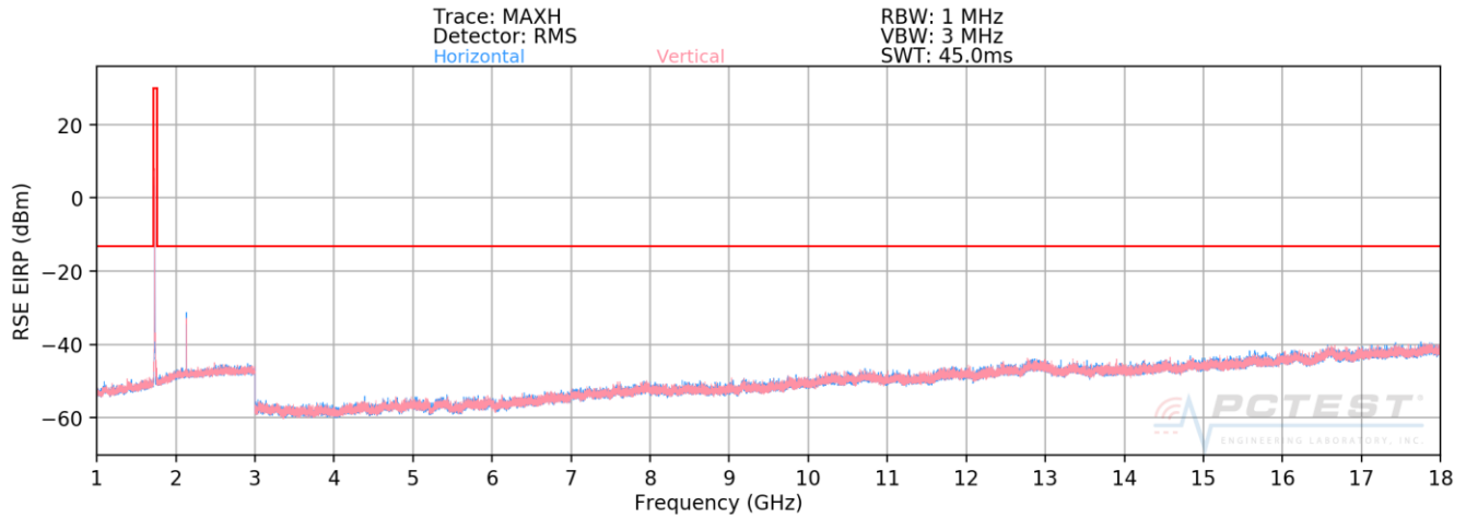
Plot 7-46. Radiated Spurious Plot above 1GHz (AWS WCDMA mode Ch. 1413)
