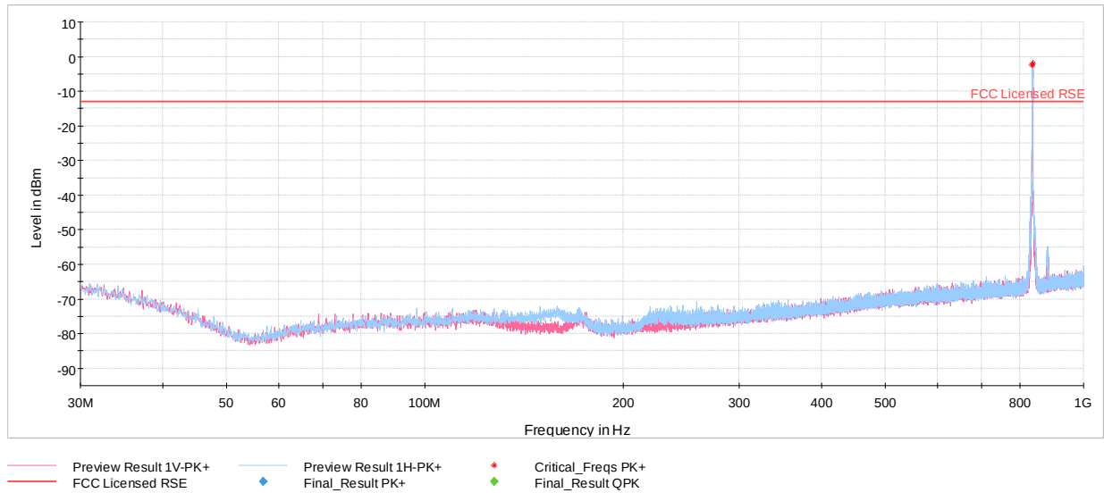
Plot 7-44. Radiated Spurious Plot below 1GHz (Cellular WCDMA Mode Mid channel, with WCP + AC/DC Adapter)
