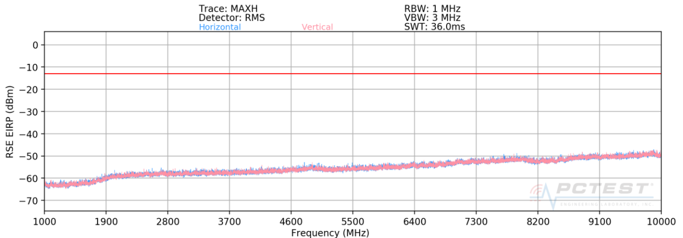
Plot 7-45. Radiated Spurious Plot above 1GHz (Cellular WCDMA Mode Mid channel)
