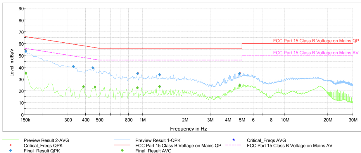
Plot 7-39. Line Conducted Plot with Bluetooth LE (L1 - 1Mbps, ePA, Ch.19 with WCP + Laptop)
