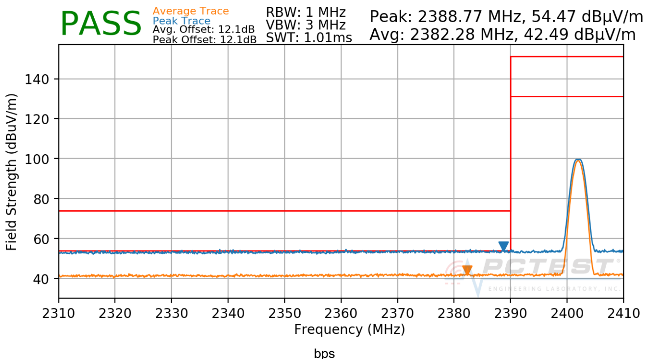
Plot 7-34. Radiated Restricted Lower Band Edge Measurement (Average & Peak)
