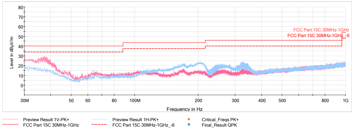
Plot 7-38. Radiated Spurious Plot below 1GHz (1Mbps, ePA, Ch.19 with WCP + AC/DC Adapter)
