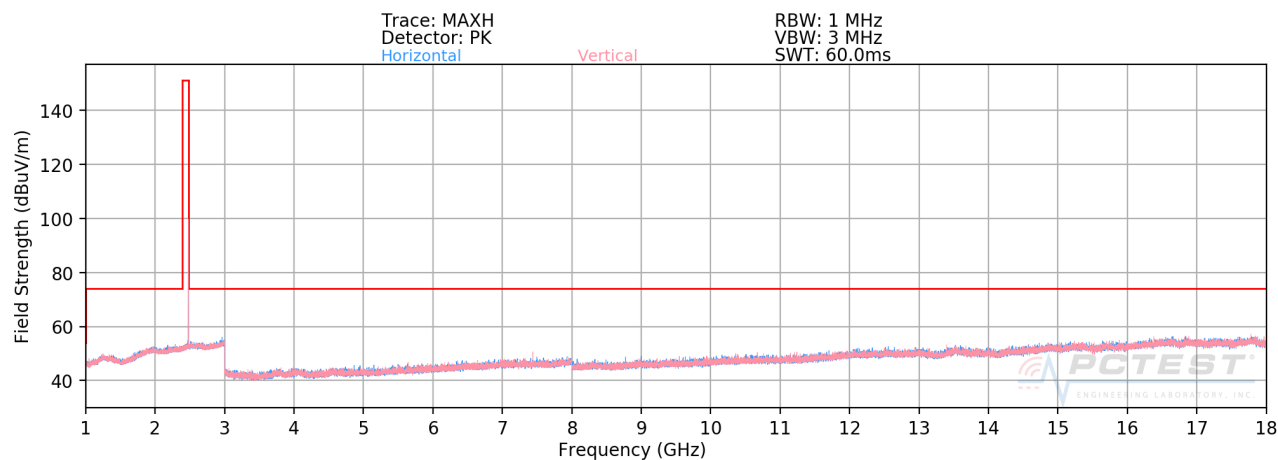
Plot 7-31. Radiated Spurious Plot Above 1GHz (1Mbps, ePA – Ch. 39)
