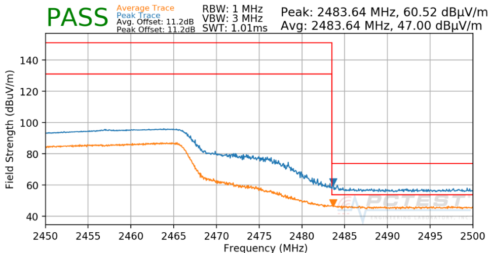
Plot 7-47. Radiated Restricted Upper Band Edge Measurement
