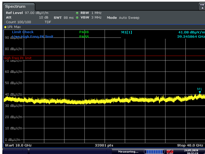
Plot 7-33. Radiated Spurious Plot Above 18GHz (4Mbps, HDR, ePA – Ch. 38, Ant. Pol. V)
