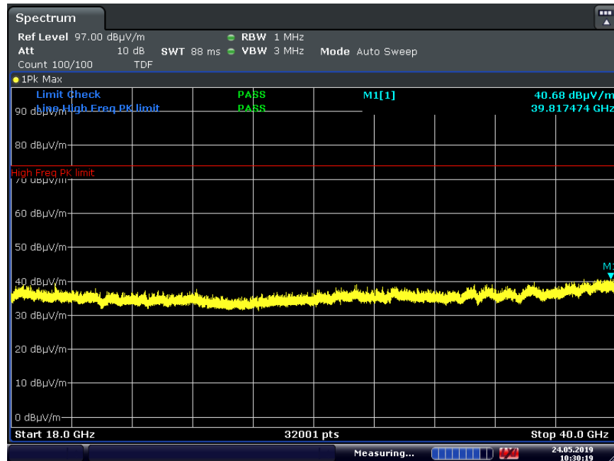
Plot 7-32. Radiated Spurious Plot Above 18GHz (4Mbps, HDR, ePA – Ch. 38, Ant. Pol. H)
