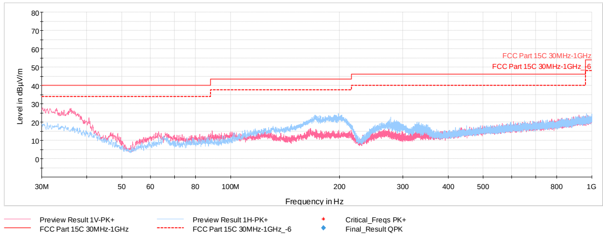
Plot 7-38. Radiated Spurious below 1GHz (4Mbps, HDR ePA, Ch.38 with WCP + AC/DC Adapter attached)
