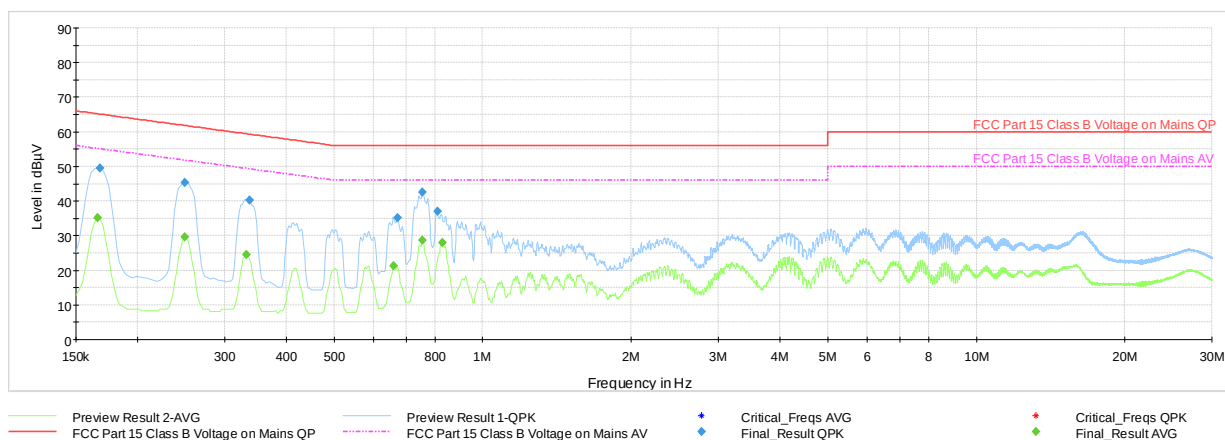
Plot 7-43. Line-Conducted Test Plot – GFSK ePA Ch.39 (L1, with WCP + AC/DC Adapter)
