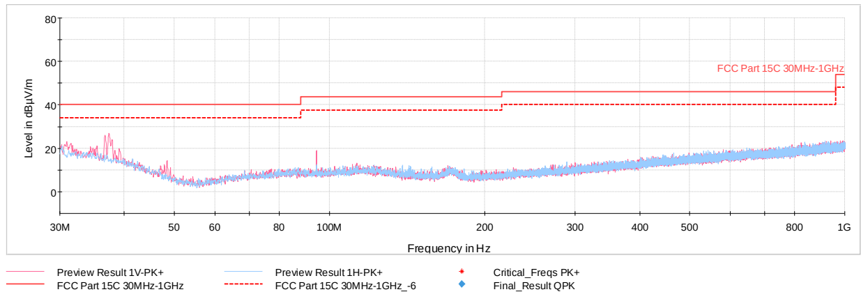
Plot 7-42. Radiated Spurious Plot Below 1GHz (with WCP + AC/DC Adapter)
