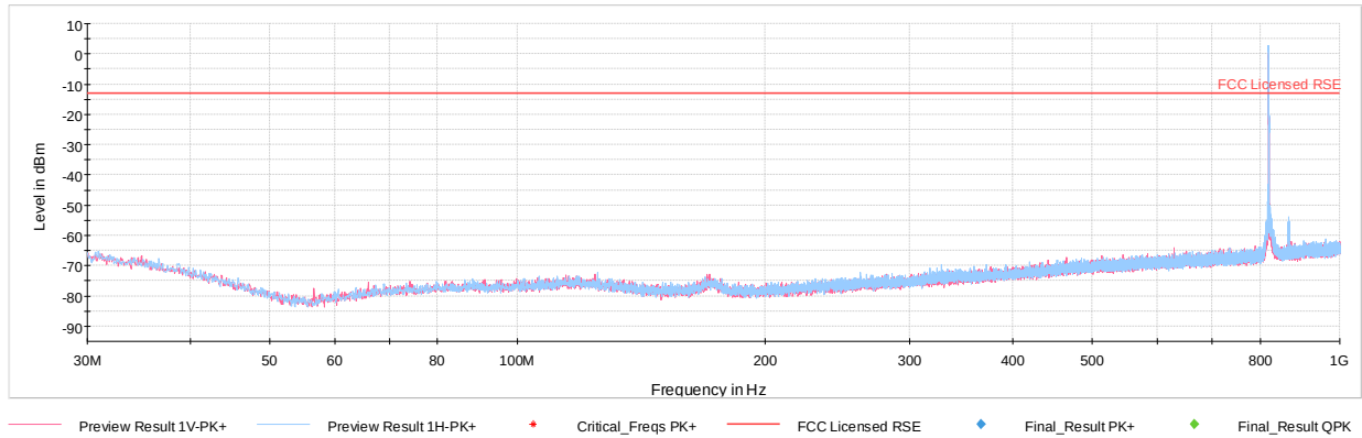
Plot 7-270. Radiated Spurious Plot - Below 1GHz (Band 26/5 – with WCP + AC/DC Adapter)
