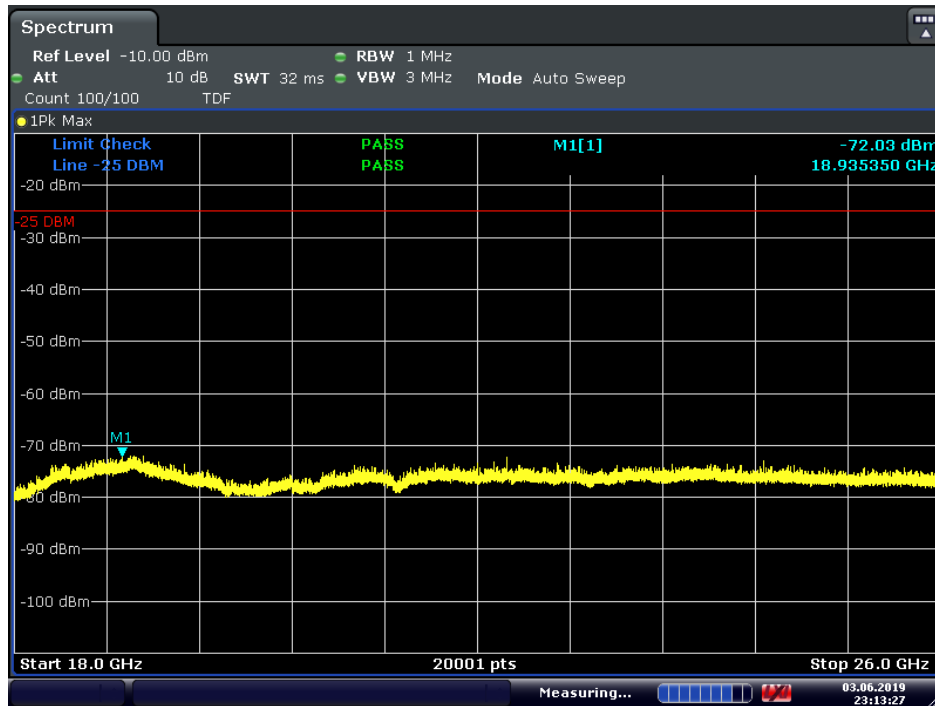
Plot 7-275. Radiated Spurious Plot 18GHz – 26GHz (Band 7, Pol. H)
