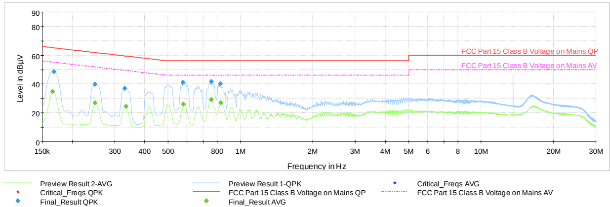
Plot 7-13. Line-Conducted Test Plot (N, with WCP + AC/DC Adapter attached)
