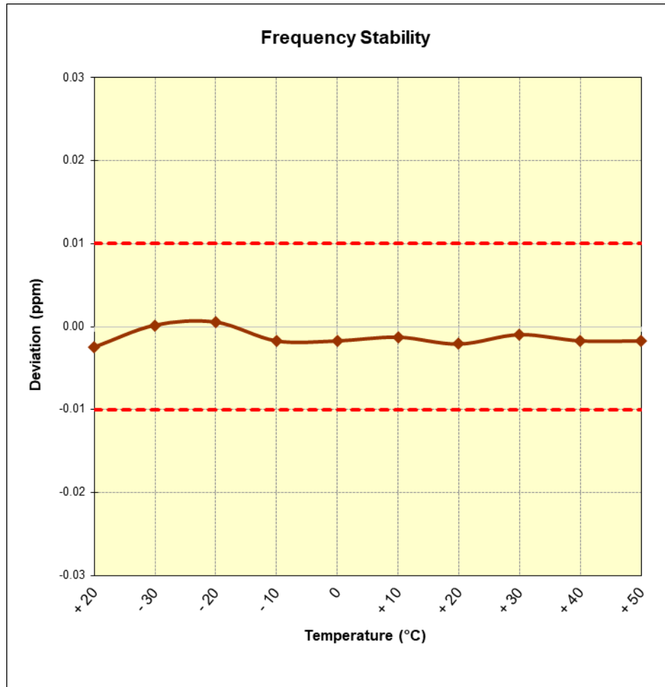
Figure 7-3. Frequency Stability Plot (Reader 10% Ask 1 out of 256)
