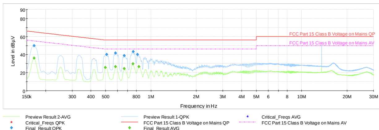
Plot 7-12. Line-Conducted Test Plot (L1, with WCP + AC/DC Adapter attached)
