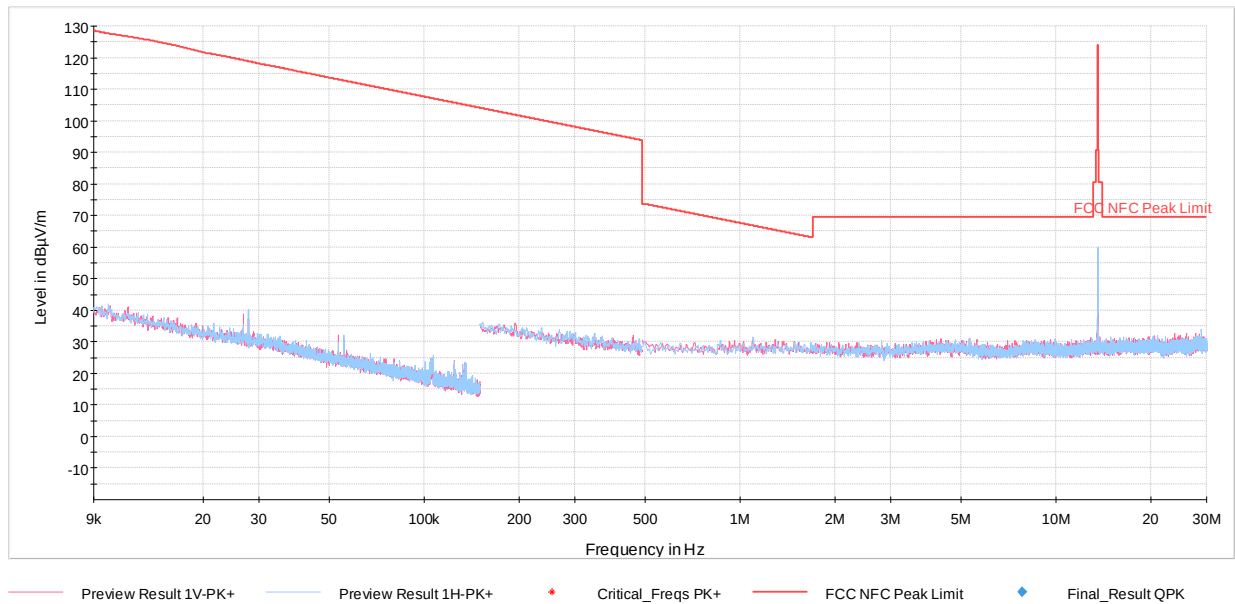
Plot 7-8. Radiated Spurious Plot 9kHz – 30MHz (CE A 848kbps)
