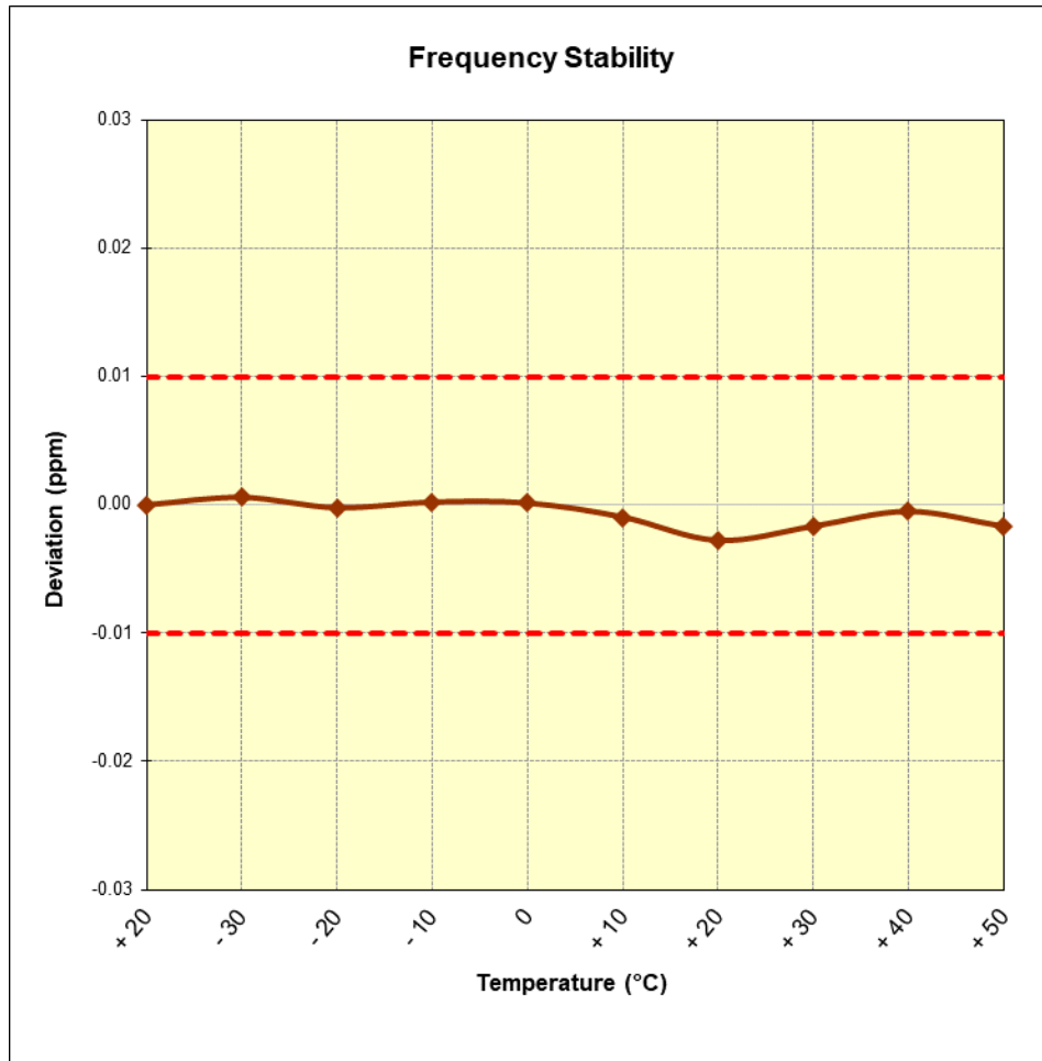
Figure 7-2. Frequency Stability Plot (CE A 848kbps)
