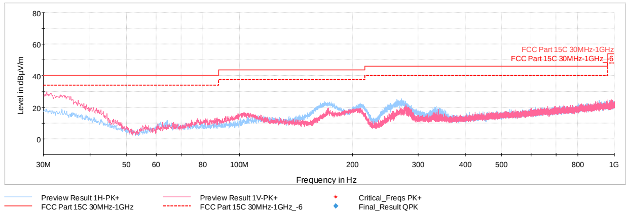
Plot 7-10. Radiated Spurious Plot 30MHz – 1GHz (CE A 848kbps, with WCP + AC/DC Adapter)
