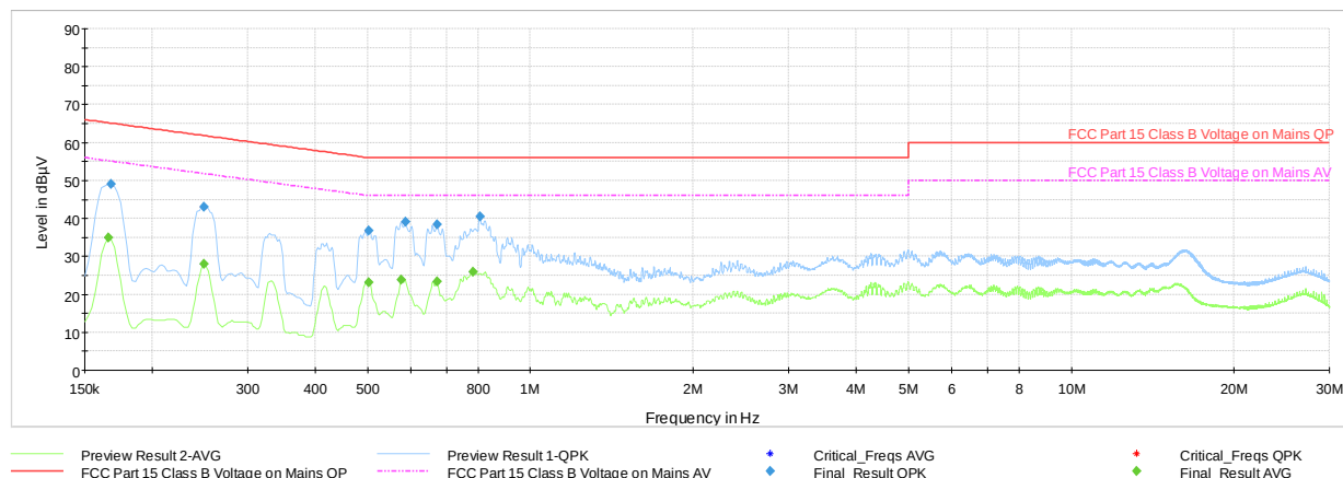
Plot 7-52. Line Conducted Plot with 802.11b (L1, with WCP + AC/DC Adapter)
