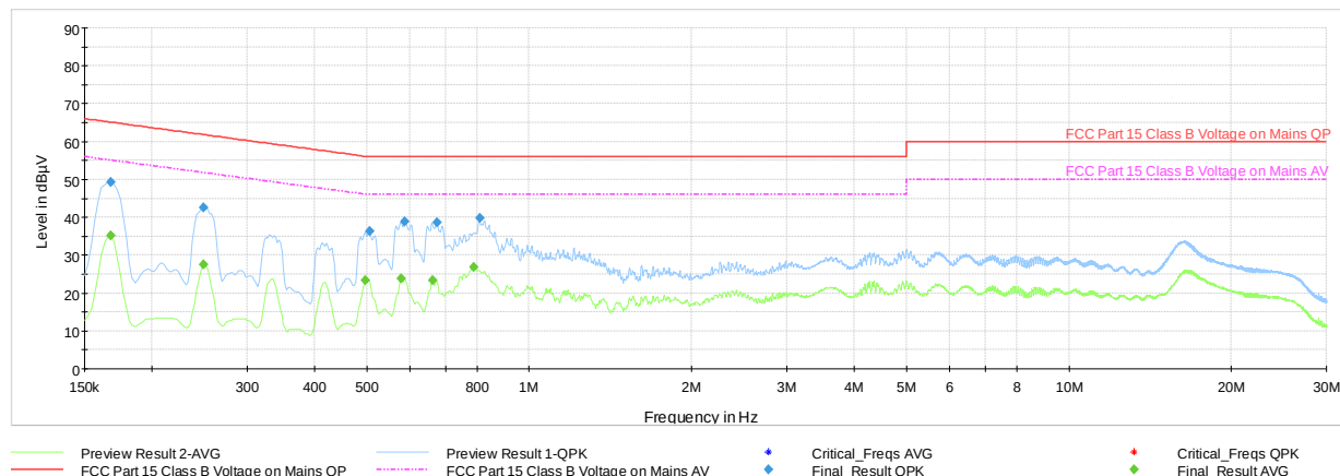
Plot 7-53. Line Conducted Plot with 802.11b (N, with WCP + AC/DC Adapter)
