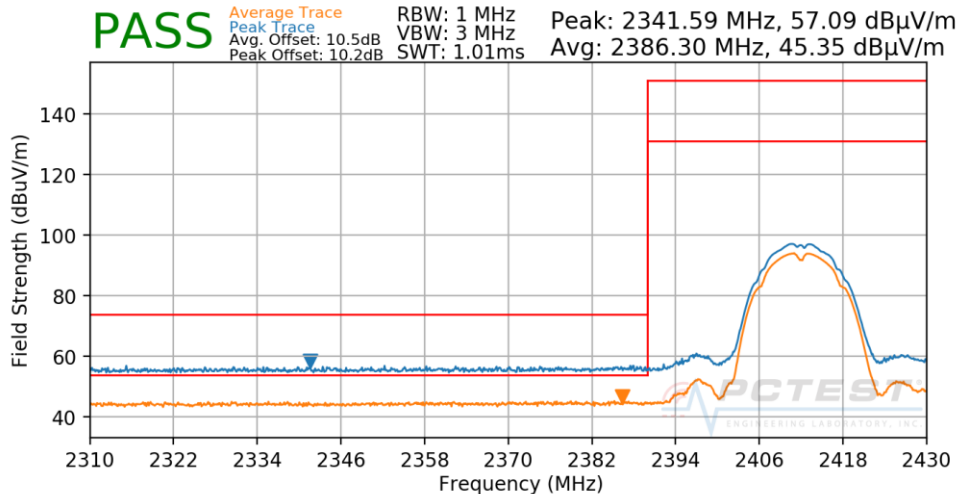
Plot 7-42. Radiated Restricted Lower Band Edge Measurement
