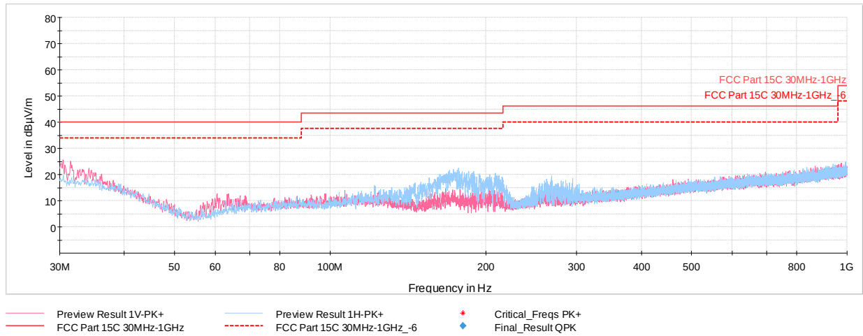
Plot 7-51. Radiated Spurious Plot below 1GHz (802.11b – Ch.6, with WCP + AC/DC Adapter)
