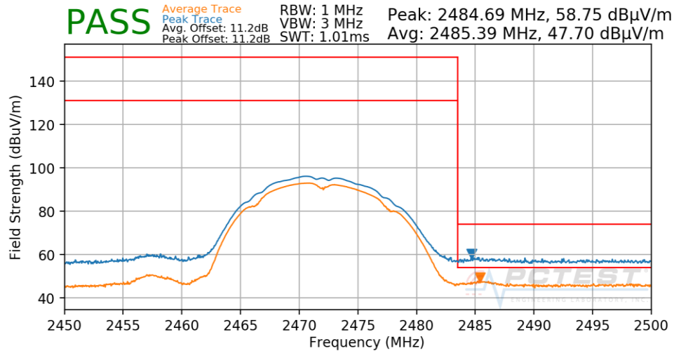
Plot 7-44. Radiated Restricted Upper Band Edge Measurement
