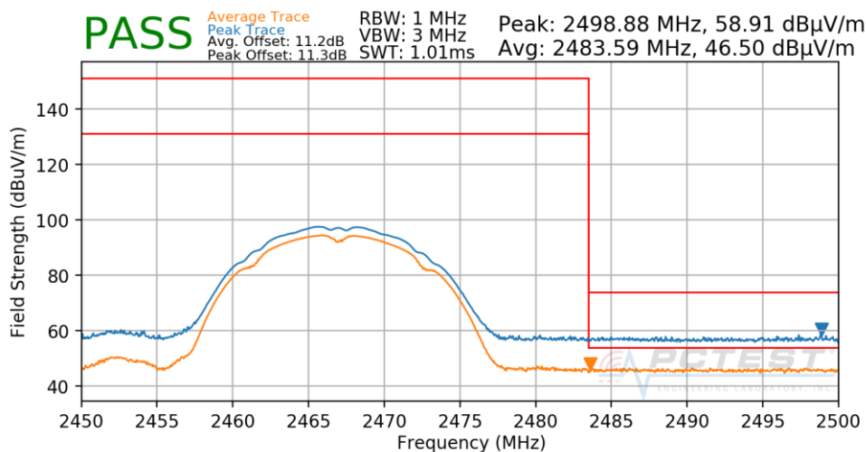
Plot 7-43. Radiated Restricted Upper Band Edge Measurement
