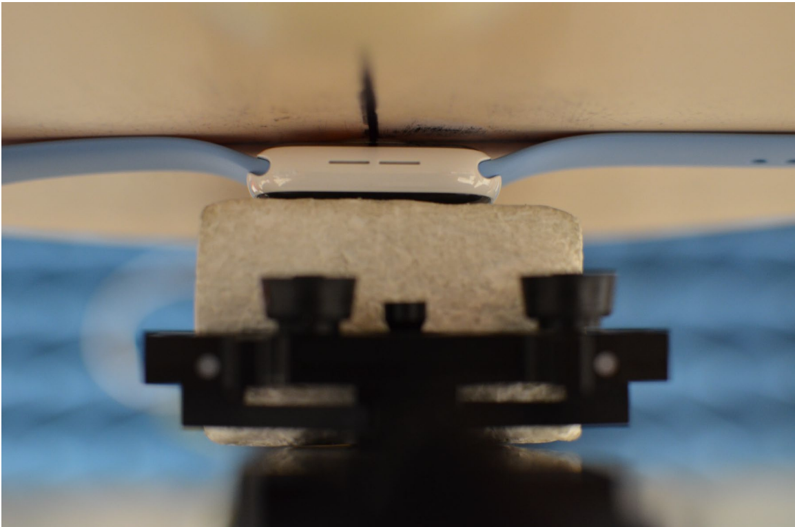
SAR Test Setup Photo 22: Ceramic with Sport Wristband, Back side at 0.0 cm
