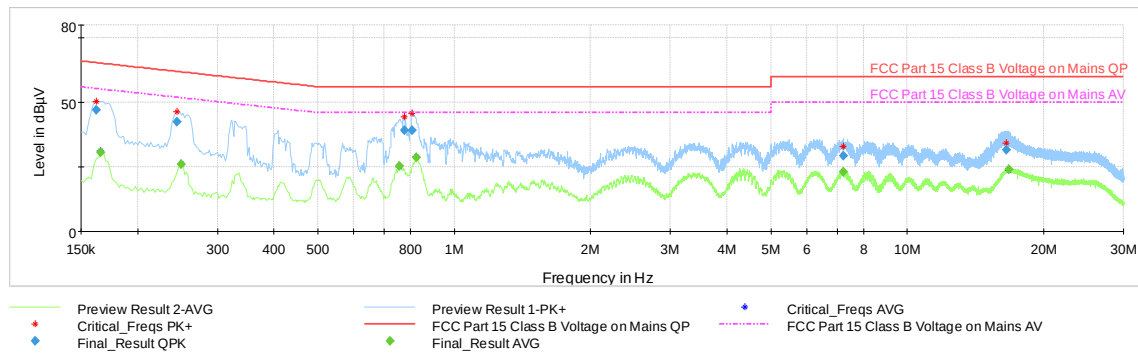
Plot 7-40. AC Line Conducted Emission with Bluetooth LE (N - 1Mbps, ePA, Ch.19, with WCP + AC/DC Adapter)
