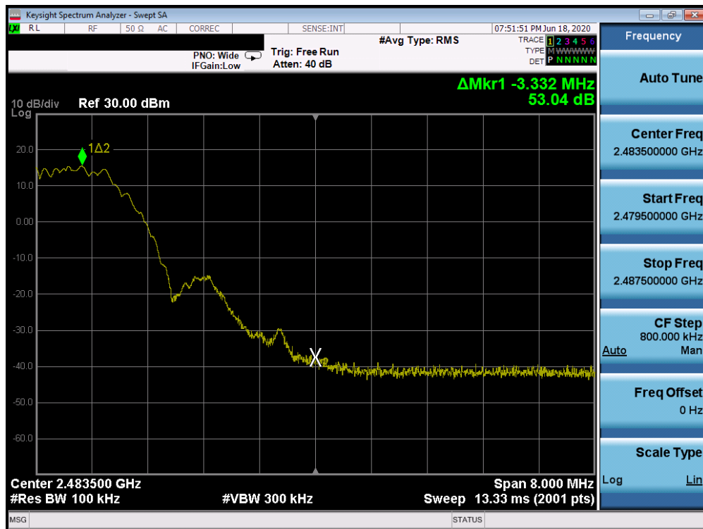
Plot 7-22. Band Edge Plot (Bluetooth (LE), 2Mbps, ePA – Ch. 39)
