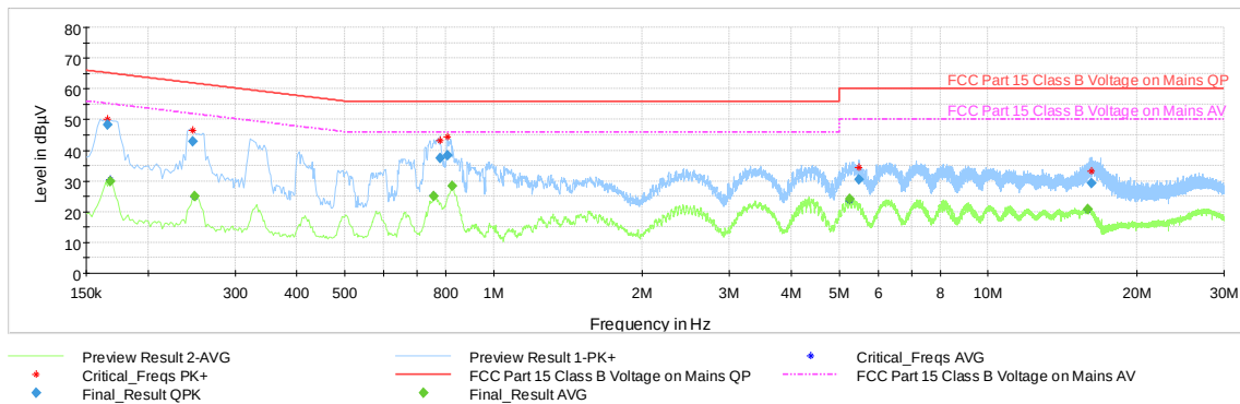
Plot 7-39. AC Line Conducted Emission with Bluetooth LE (L1 - 1Mbps, ePA, Ch.19, with WCP + AC/DC Adapter)
