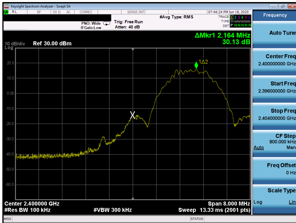
Plot 7-21. Band Edge Plot (Bluetooth (LE), 2Mbps, ePA – Ch. 0)
