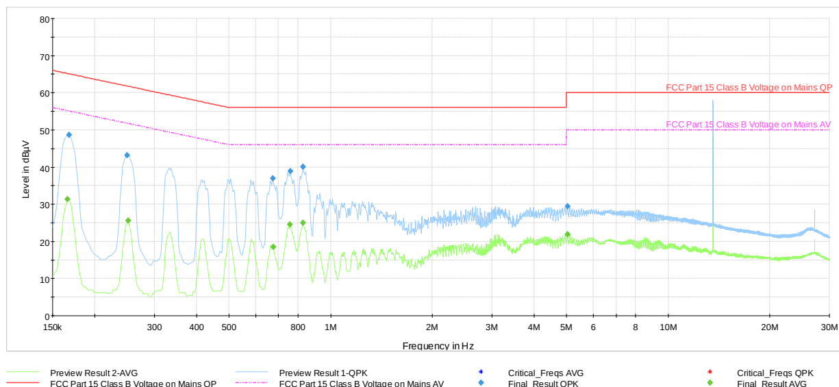
Plot 7-12. AC Line-Conducted Test Plot (L1, with WCP + AC/DC Adapter)
