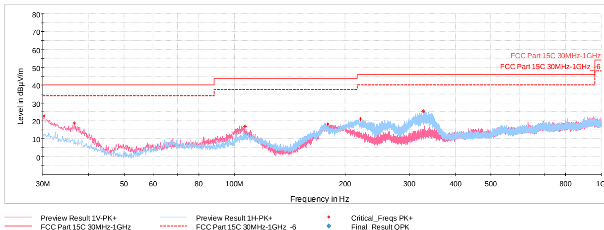
Plot 7-50. Radiated Spurious Emission – Simultaneous Transmission below 1GHz with AC/DC Adapter
