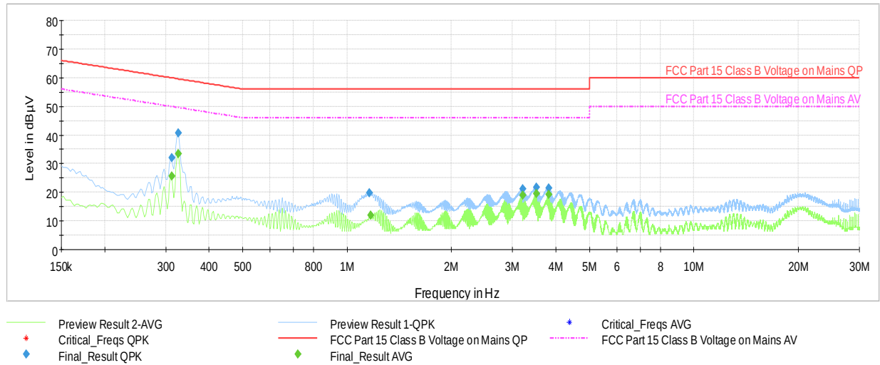
Plot 7-52. AC Line Conducted Plot with 802.11n UNII Band 3 – Ch.165 (N) with Laptop
