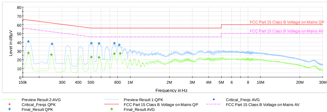
Plot 7-62. AC Line Conducted Emission with 802.11b Ch.6 (N, with WCP + AC/DC Adapter)
