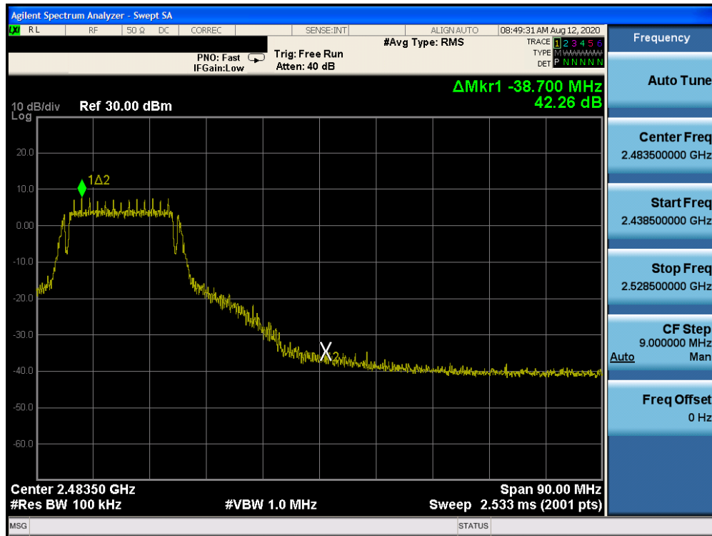
Plot 7-25. Band Edge Plot (802.11g- Ch. 9)
