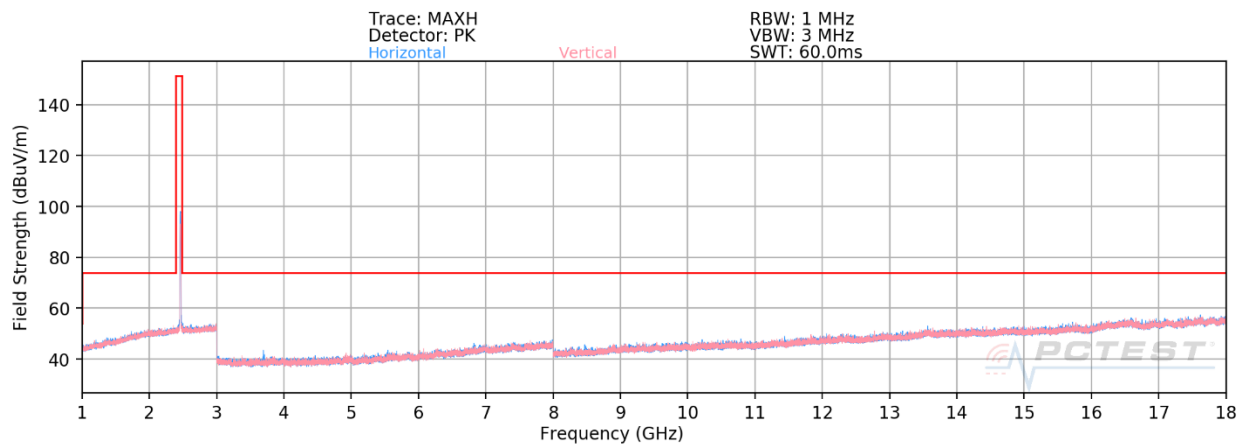
Plot 7-46. Radiated Spurious Emissions 1-18GHz (802.11b – Ch. 11)
