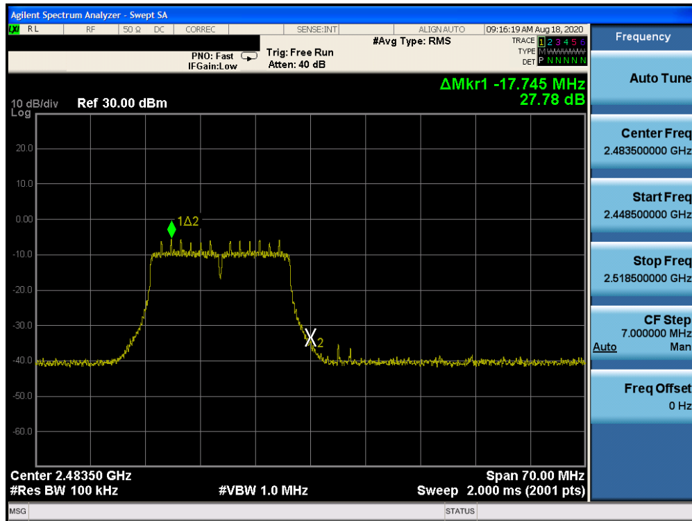
Plot 7-37. Band Edge Plot (802.11n (2.4GHz) – Ch. 13)
