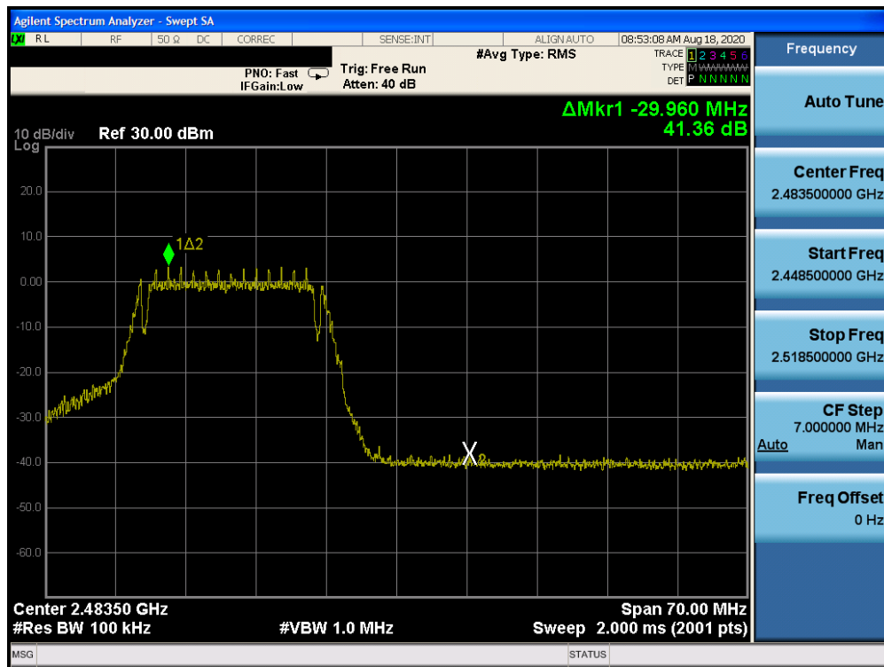
Plot 7-28. Band Edge Plot (802.11g – Ch. 12)
