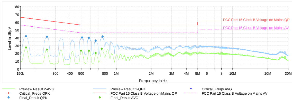
Plot 7-61. AC Line Conducted Emission with 802.11b Ch.6 (L1, with WCP + AC/DC Adapter)
