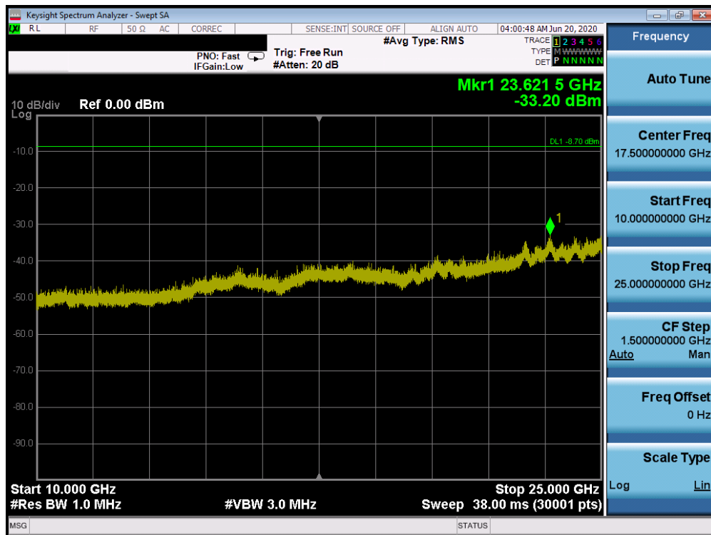
Plot 7-43. Conducted Spurious Plot (802.11b – Ch. 11)
