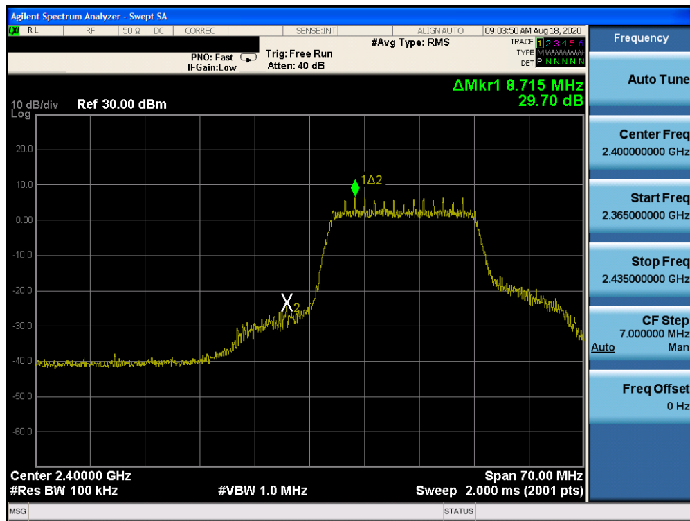
Plot 7-30. Band Edge Plot (802.11n (2.4GHz) – Ch. 1)
