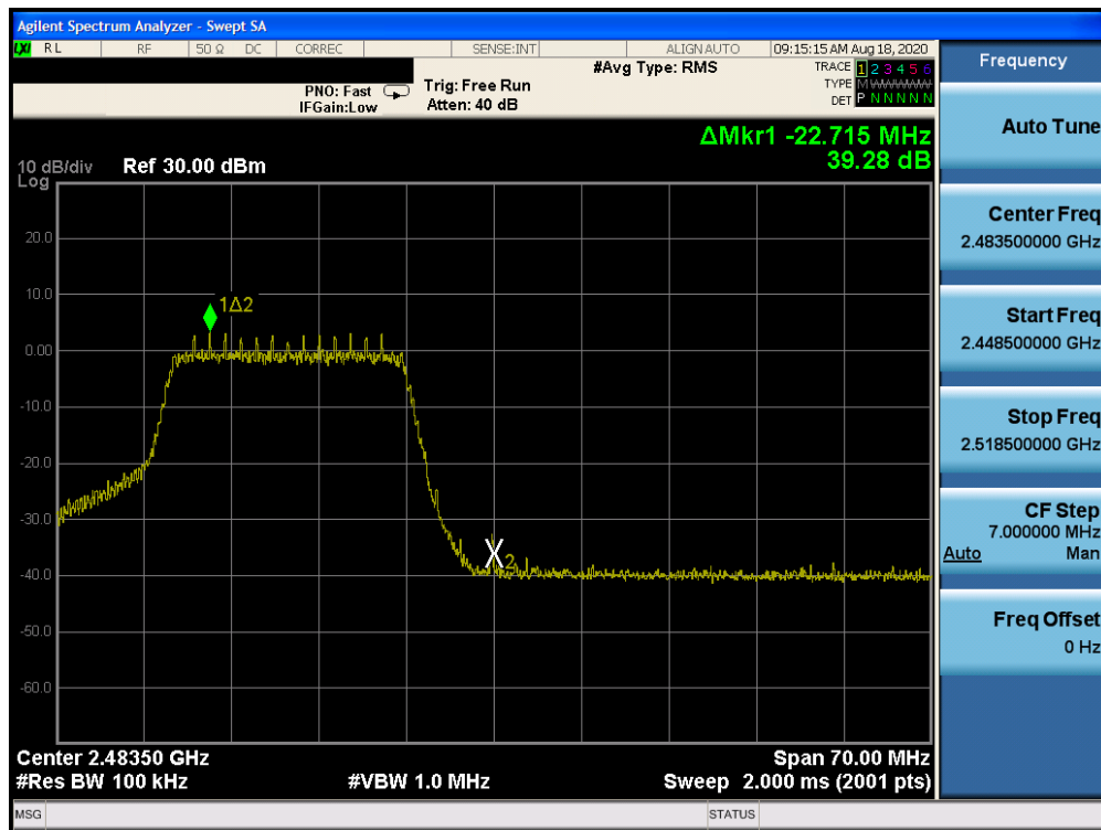
Plot 7-36. Band Edge Plot (802.11n (2.4GHz) – Ch. 12)
