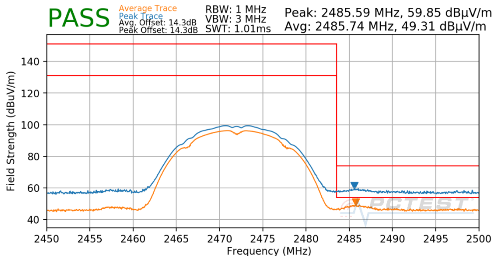
Plot 7-51. Radiated Restricted Upper Band Edge Measurement
