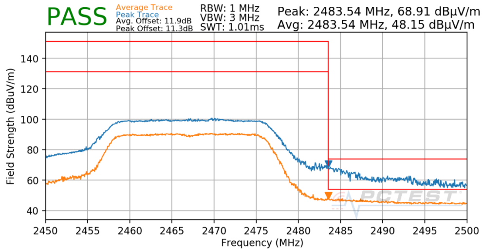
Plot 7-58. Radiated Restricted Upper Band Edge Measurement
