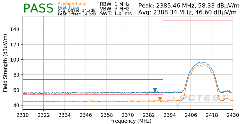
Plot 7-49. Radiated Restricted Lower Band Edge Measurement
