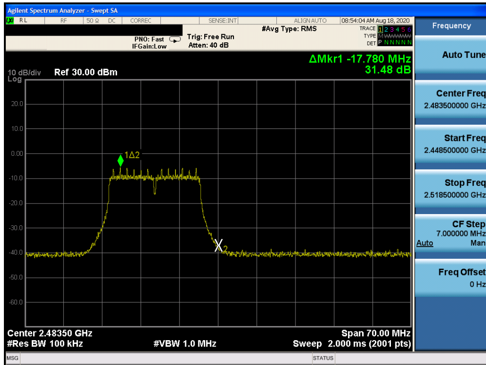
Plot 7-29. Band Edge Plot (802.11g – Ch. 13)
