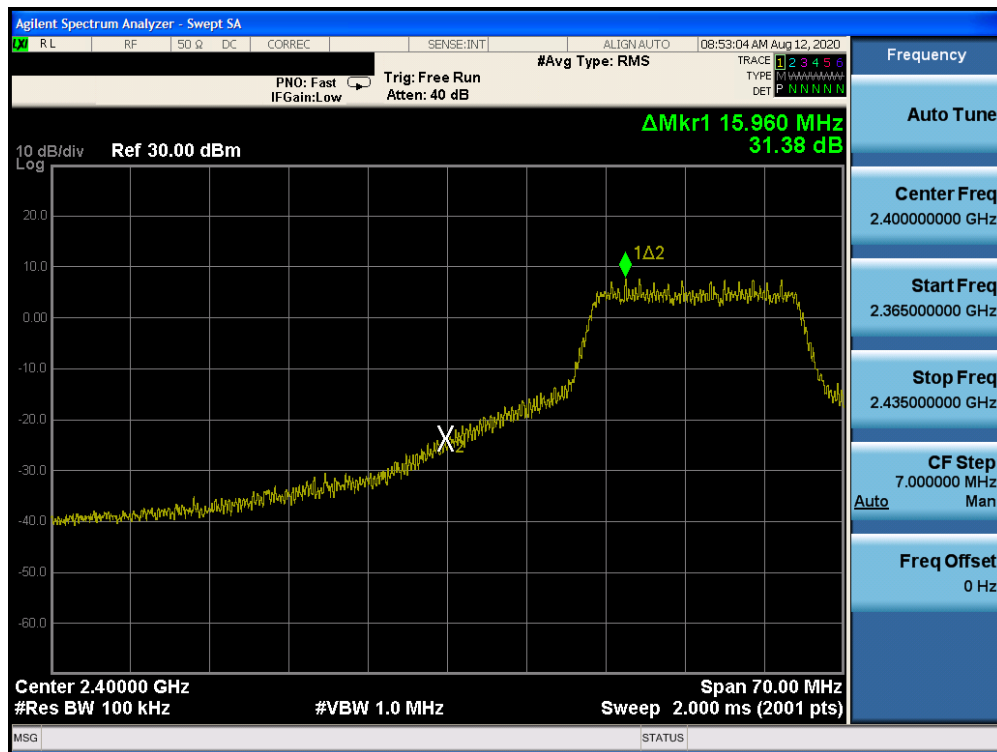
Plot 7-32. Band Edge Plot (802.11n (2.4GHz) – Ch. 3)
