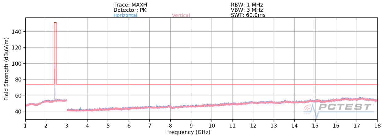
Plot 7-45. Radiated Spurious Emissions 1-18GHz (802.11b – Ch. 6)
