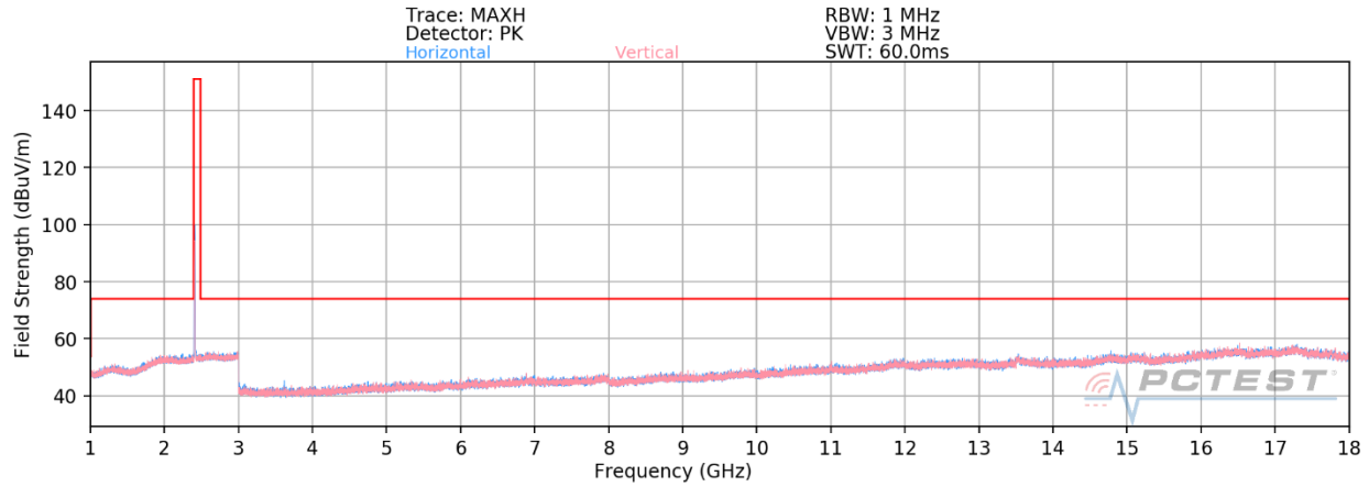
Plot 7-44. Radiated Spurious Emissions 1-18GHz (802.11b – Ch. 1)
