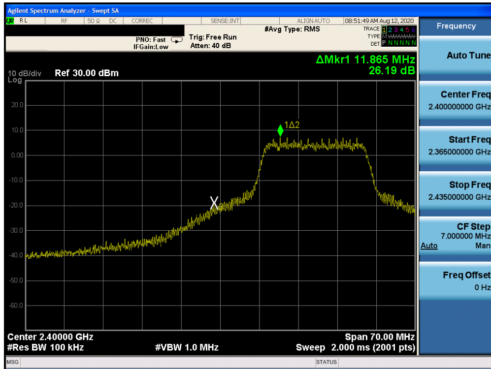
Plot 7-31. Band Edge Plot (802.11n (2.4GHz) – Ch. 2)
