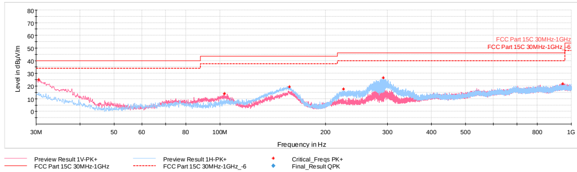
Plot 7-60. Radiated Spurious Emissions 30MHz-1GHz (802.11b – Ch.6, with WCP + AC/DC adapter)
