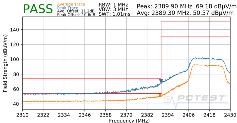
Plot 7-53. Radiated Restricted Lower Band Edge Measurement
