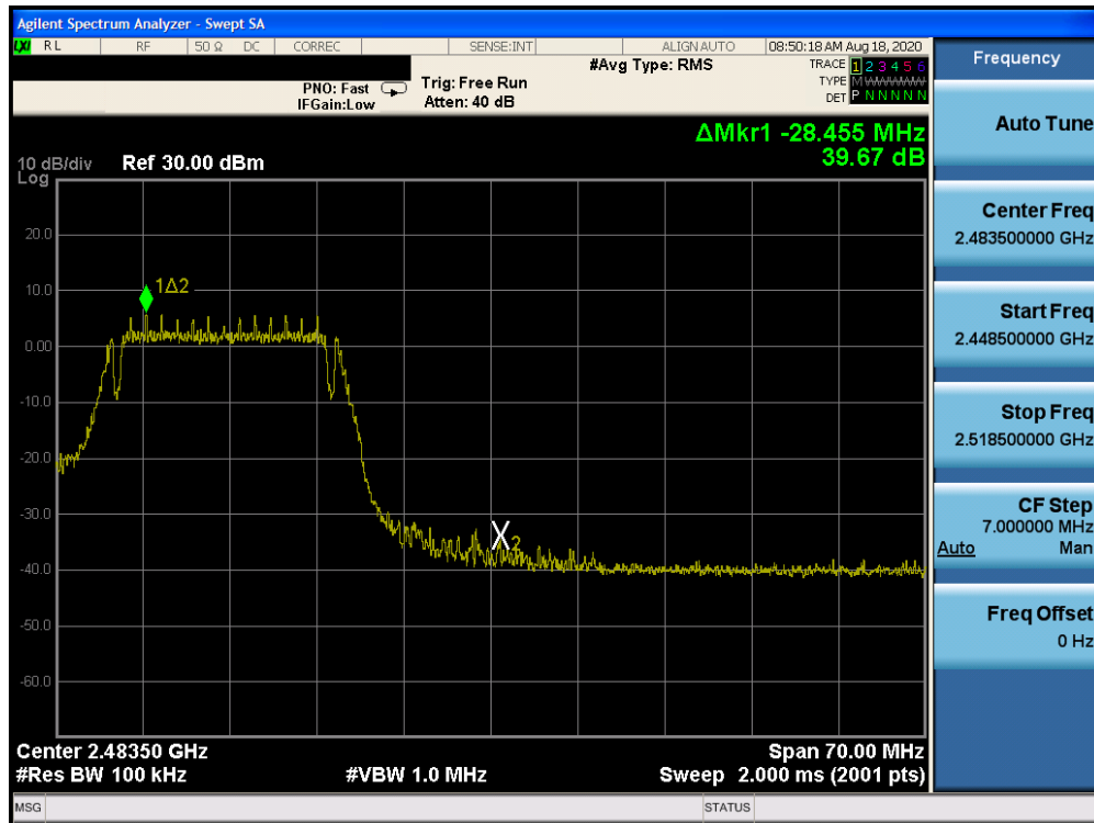
Plot 7-27. Band Edge Plot (802.11g – Ch. 11)
