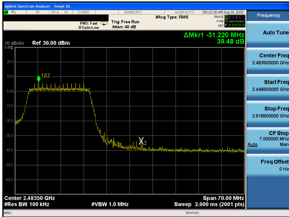
Plot 7-35. Band Edge Plot (802.11n (2.4GHz) – Ch. 11)
