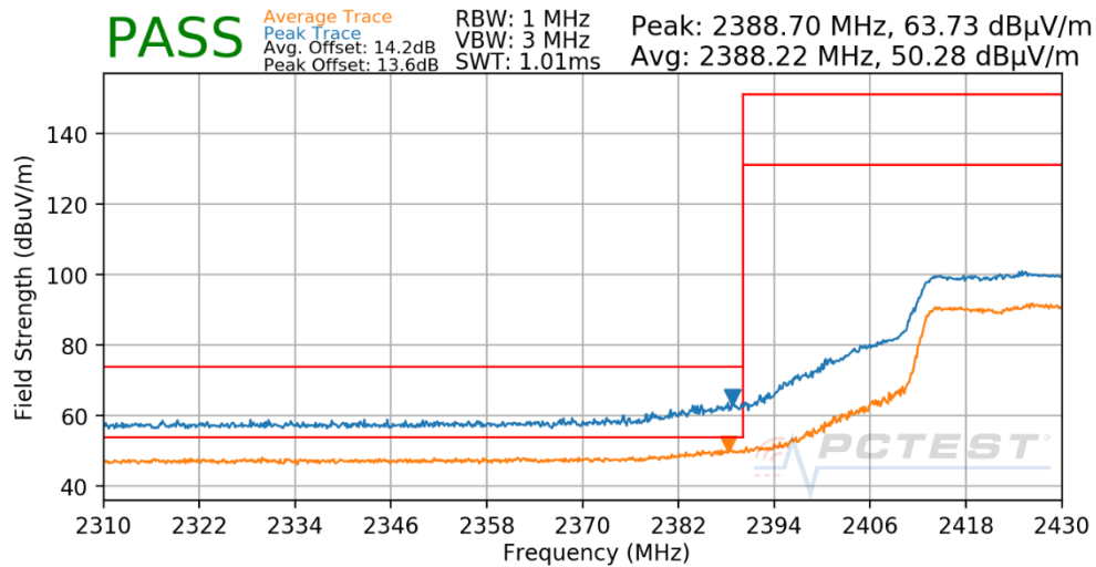
Plot 7-54. Radiated Restricted Lower Band Edge Measurement
