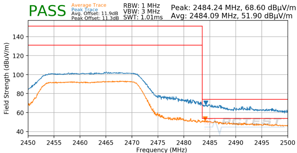
Plot 7-57. Radiated Restricted Upper Band Edge Measurement
