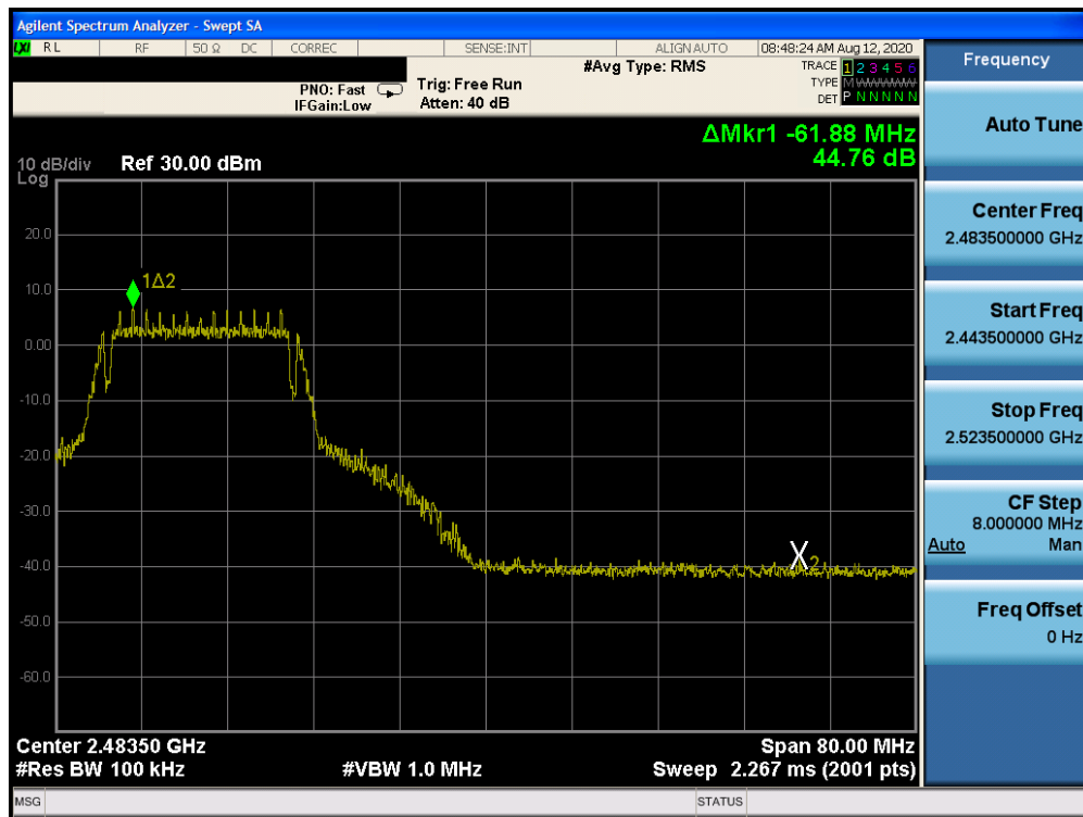
Plot 7-26. Band Edge Plot (802.11g- Ch. 10)
