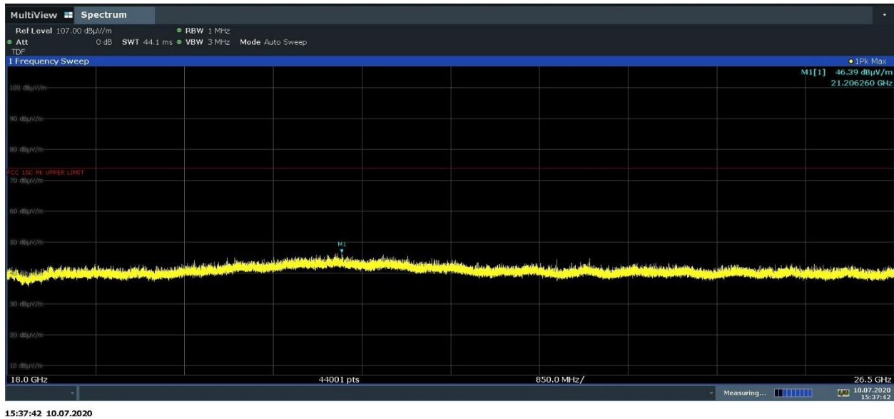
Plot 7-48. Radiated Spurious Emissions 18-26.5GHz (802.11b – Ch. 6, Ant. Pol. V)
