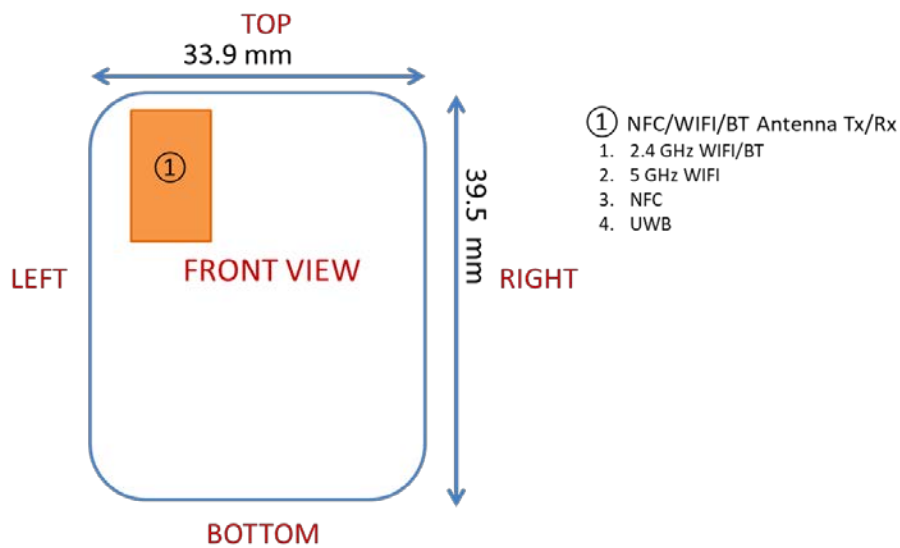
Figure E-1 DUT Antenna Locations
