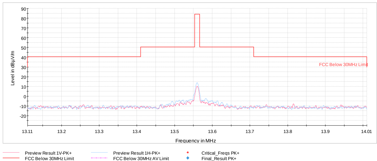
Plot 7-7. In Band Radiated Spurious Emissions (Reader 10% Ask 1 out of 256, with WCP + AC/DC Adapter)
