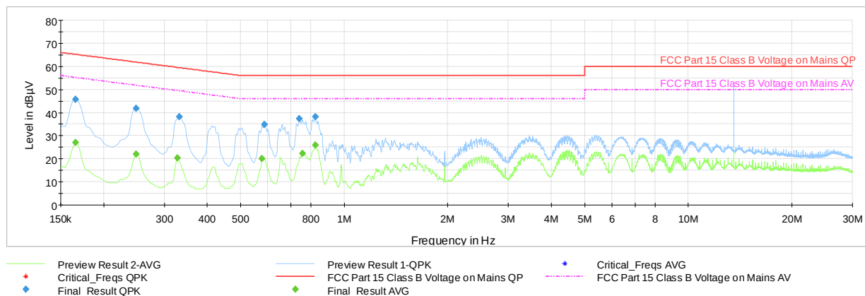
Plot 7-13. AC Line-Conducted Test Plot (N, with WCP + AC/DC Adapter)
