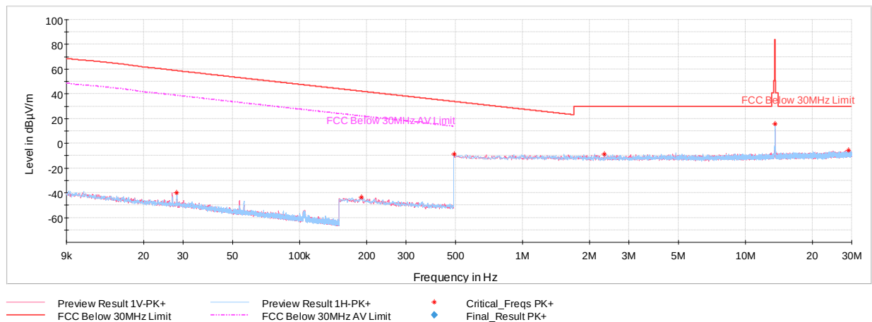
Plot 7-9. Radiated Spurious Emissions 9kHz – 30MHz (Reader 10% Ask 1 out of 256, with WCP + AC/DC Adapter)
