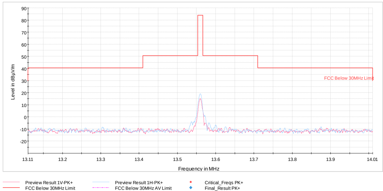
Plot 7-6. In Band Radiated Spurious Emissions (CE A 848kbps, with WCP + AC/DC Adapter)
