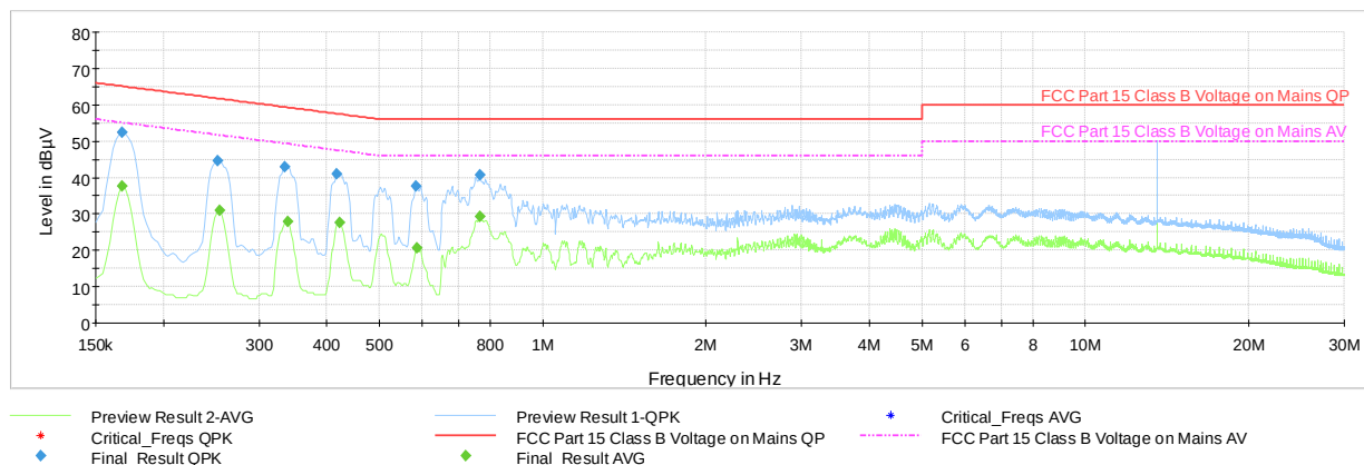
Plot 7-12. AC Line-Conducted Test Plot (L1, with WCP + AC/DC Adapter)
