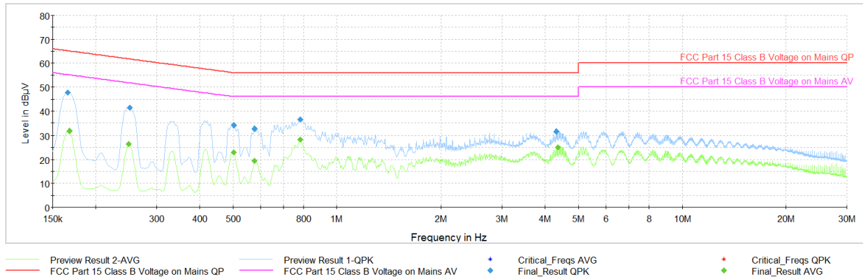
Plot 7-40. AC Line Conducted Plot with Bluetooth HDR (N – 4Mbps, ePA, Ch. 38 with WCP + AC/DC Adapter)
