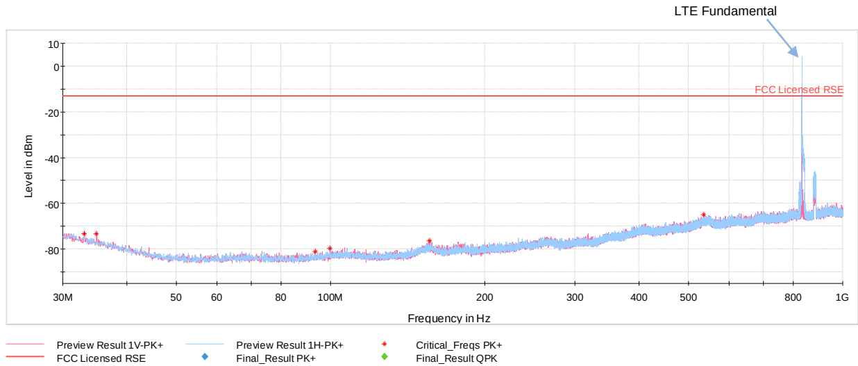
Plot 7-22. Radiated Spurious Emissions Below 1GHz (Band 26)
