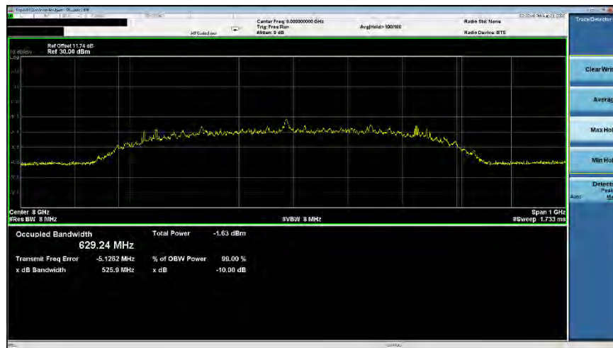
Plot 7-38. ISSED Occupied Bandwidth (Ch. 9, Config 3/Payload 125)
