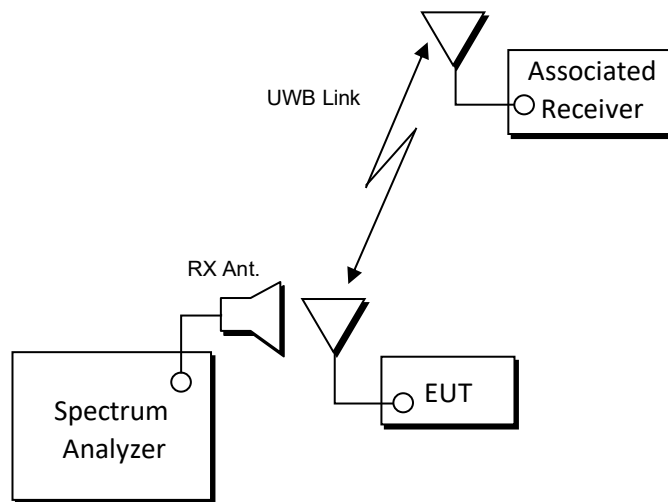
Figure 7-4. Test Setup
