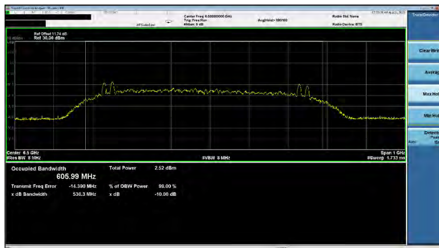
Plot 7-23. ISD Occupied Bandwidth (Ch. 5, Config 0/Payload 125)
