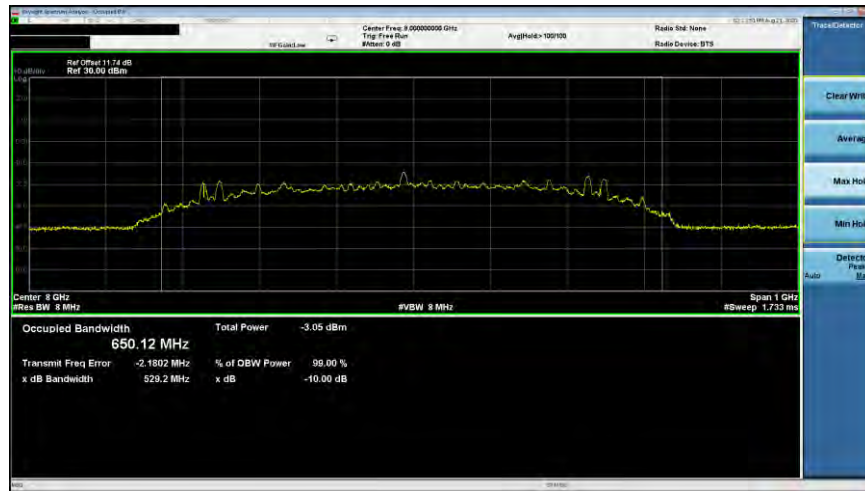
Plot 7-37. ISSED Occupied Bandwidth (Ch. 9, Config 2/Payload 125)
