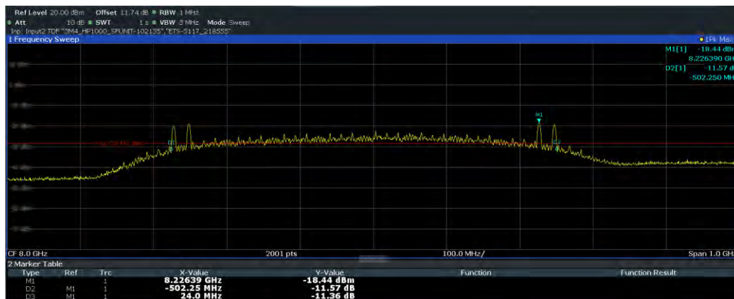
Plot 7-19. 10dBc Bandwidth (Ch. 9, Config 4/Payload 0)
