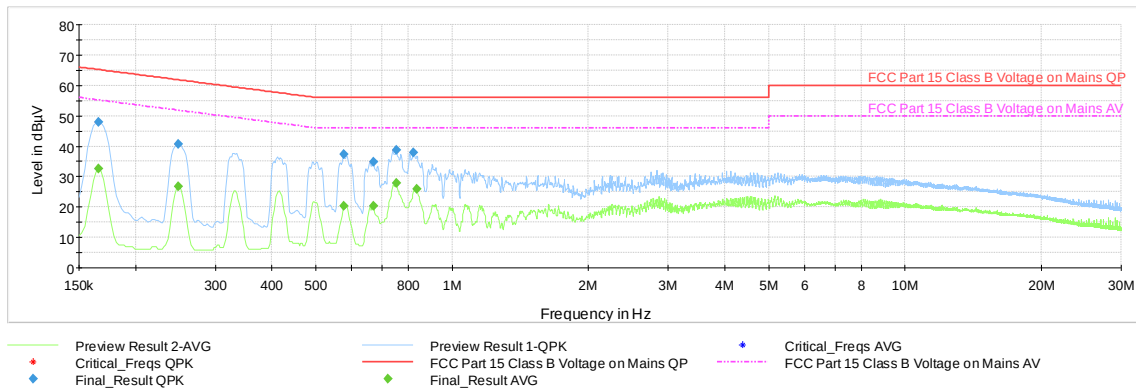
Plot 7-40. AC Line Conducted Plot with Bluetooth LE (N - 1Mbps, ePA, Ch.19, with WCP + AC/DC Adapter)
