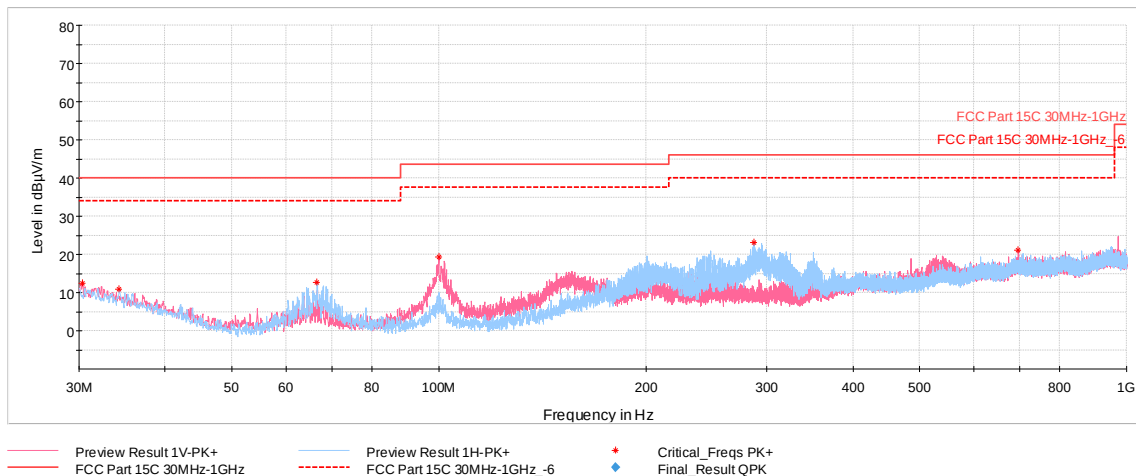
Plot 7-38. Radiated Spurious Emissions 30MHz-1GHz (1Mbps, ePA – Ch.19, with WCP + Laptop)
