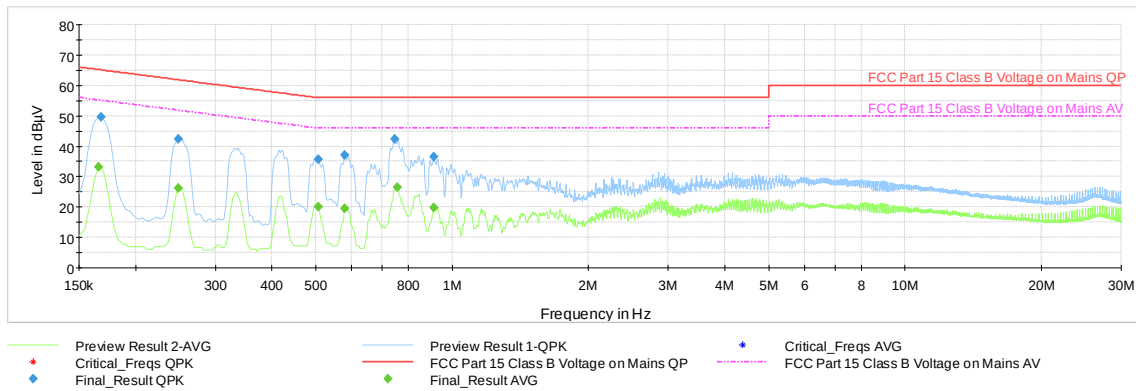
Plot 7-39. AC Line Conducted Plot with Bluetooth LE (L1 - 1Mbps, ePA, Ch.19, with WCP + AC/DC Adapter)
