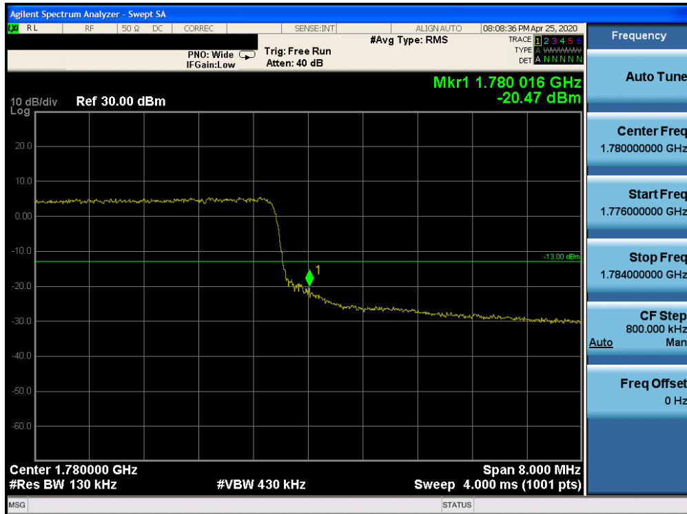
Plot 7-174. Upper Band Edge Plot (Band 66 - 10.0MHz QPSK - Full RB Configuration)
