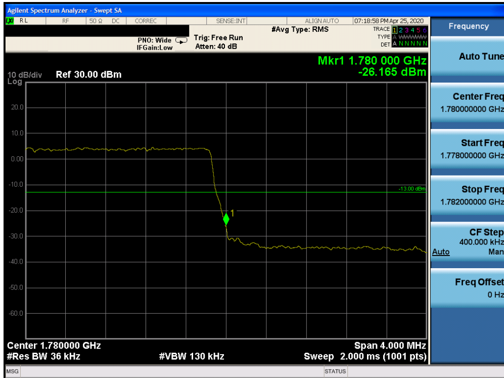
Plot 7-166. Upper Band Edge Plot (Band 66 - 3.0MHz QPSK - Full RB Configuration)
