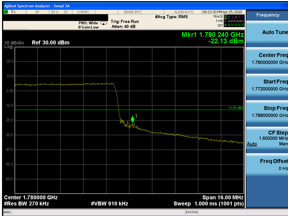
Plot 7-182. Upper Band Edge Plot (Band 66 - 20.0MHz QPSK - Full RB Configuration)
