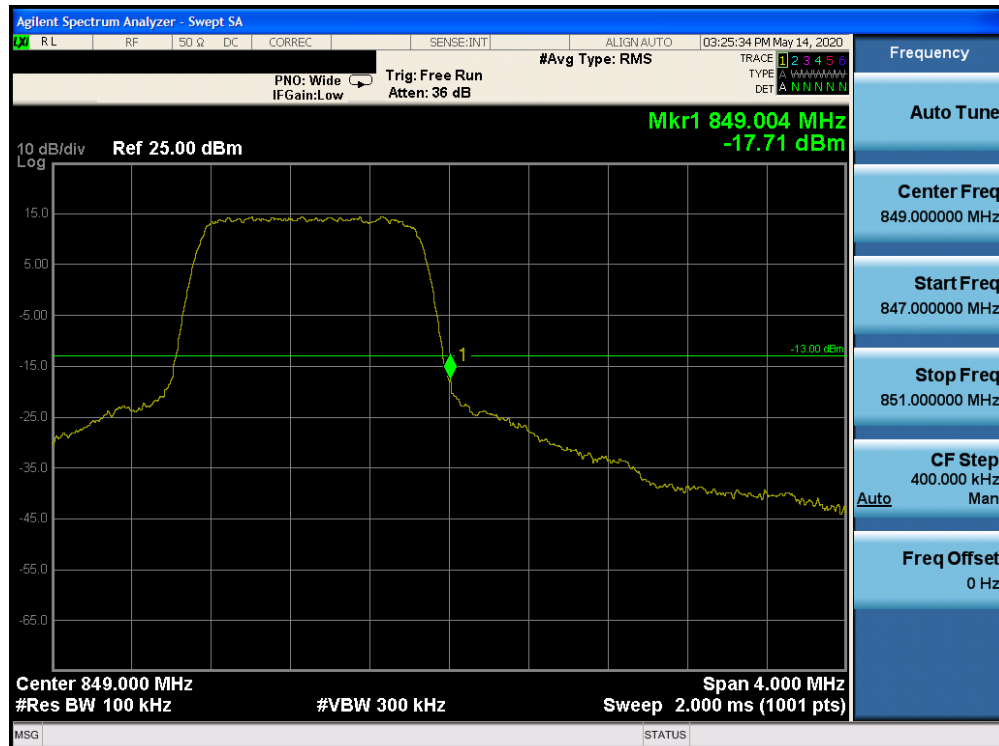
Plot 7-153. Upper Band Edge Plot (Band 5 - 1.4MHz QPSK - Full RB Configuration)
