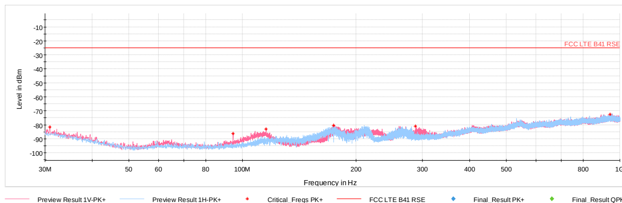
Plot 7-326. Radiated Spurious Emissions – Simultaneous Transmission 30MHz – 1GHz
