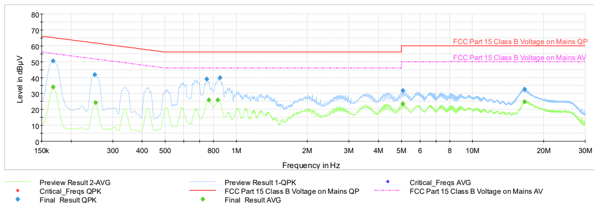
Plot 7-116. AC Line Conducted Plot (Ch. 9, Config 3, Payload 125 N, with AC/DC Adapter)
