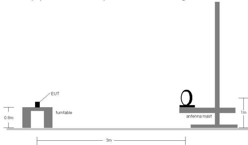
Figure 7-5. Radiated Test Setup
