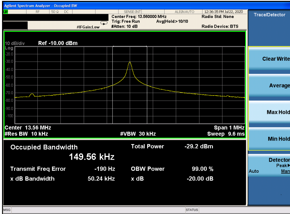
Plot 7-2. 20dB Bandwidth Plot (CE B 848kbps)
