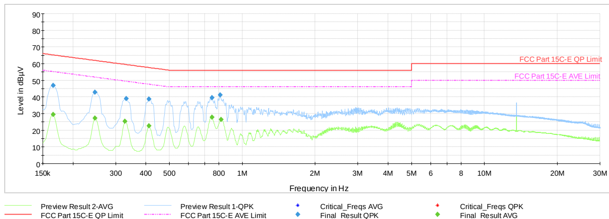
Plot 7-12. AC Line-Conducted Test Plot (L1, CE A 848kbps, with WCP + AC/DC Adapter)
