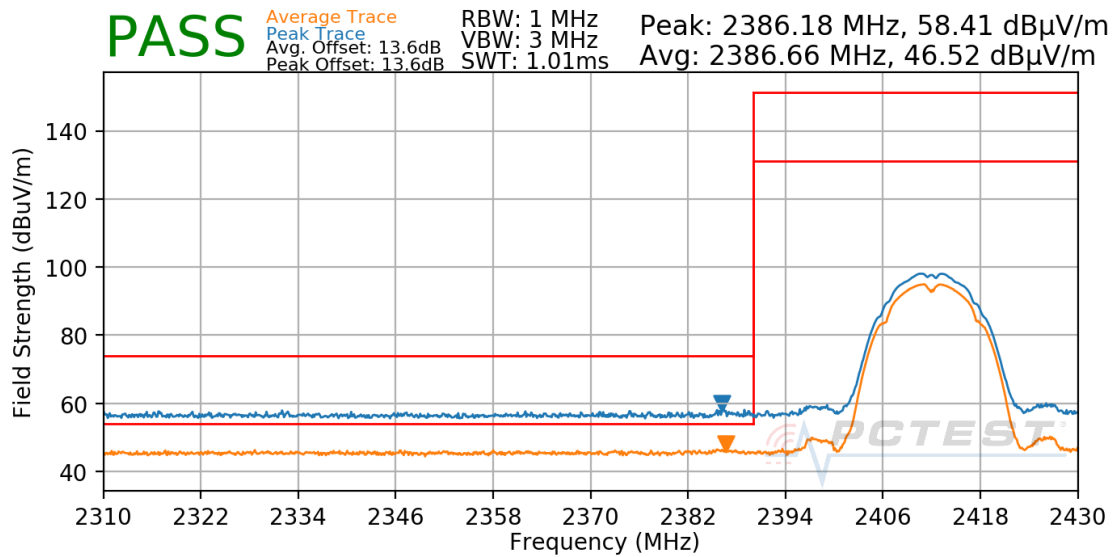
Plot 7-47. Radiated Restricted Lower Band Edge Measurement
