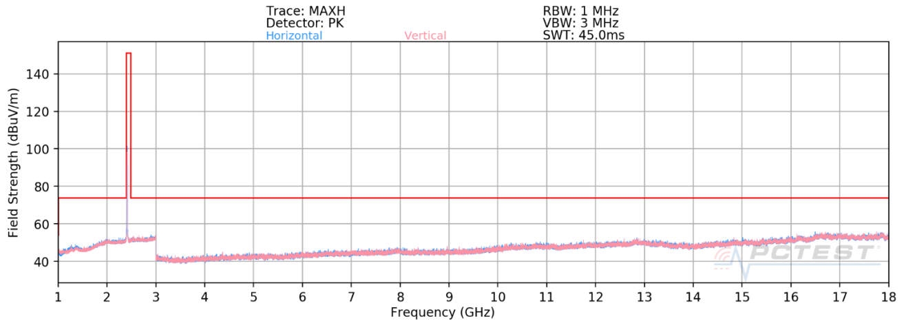
Plot 7-42. Radiated Spurious Emissions 1-18GHz (802.11b – Ch. 1)
