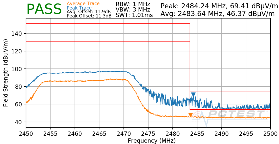
Plot 7-54. Radiated Restricted Upper Band Edge Measurement
