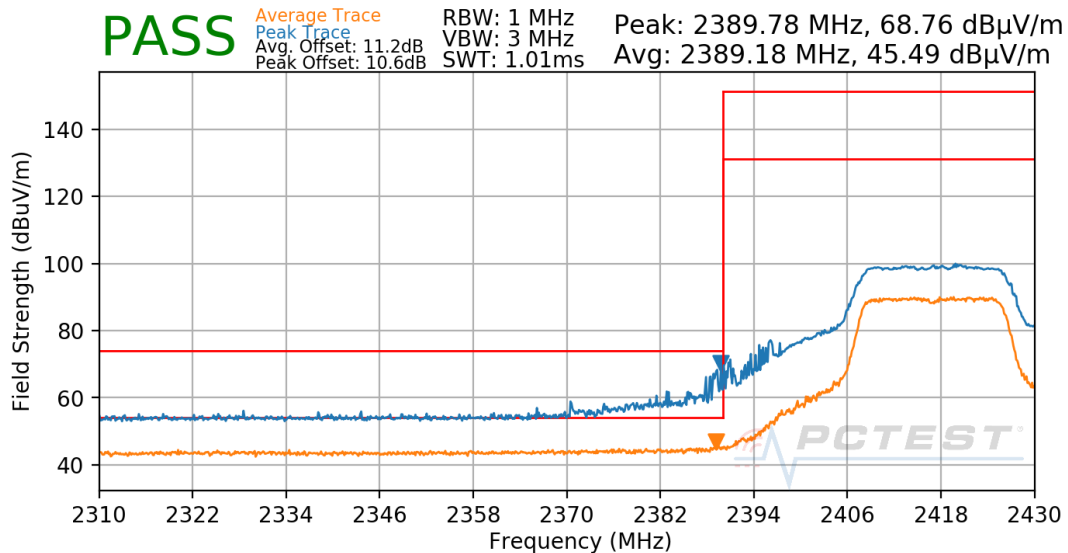
Plot 7-51. Radiated Restricted Lower Band Edge Measurement
