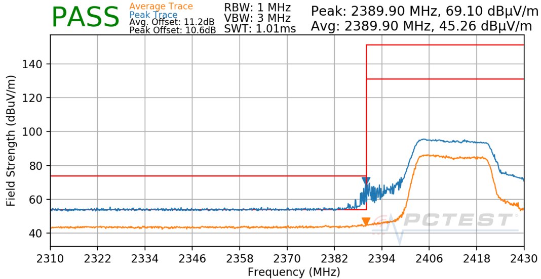
Plot 7-50. Radiated Restricted Lower Band Edge Measurement
