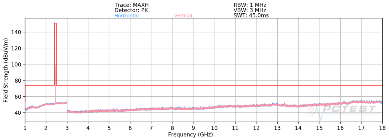
Plot 7-44. Radiated Spurious Emissions 1-18GHz (802.11b – Ch. 11)
