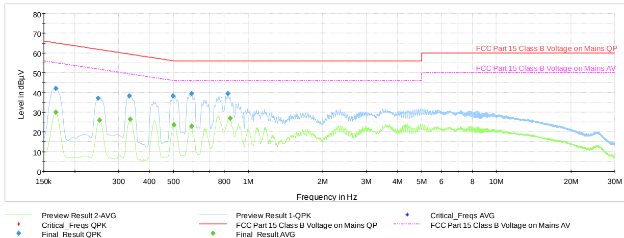
Plot 7-58. AC Line Conducted Emission with 802.11b Ch.11 (L1, with WCP + AC/DC Adapter)
