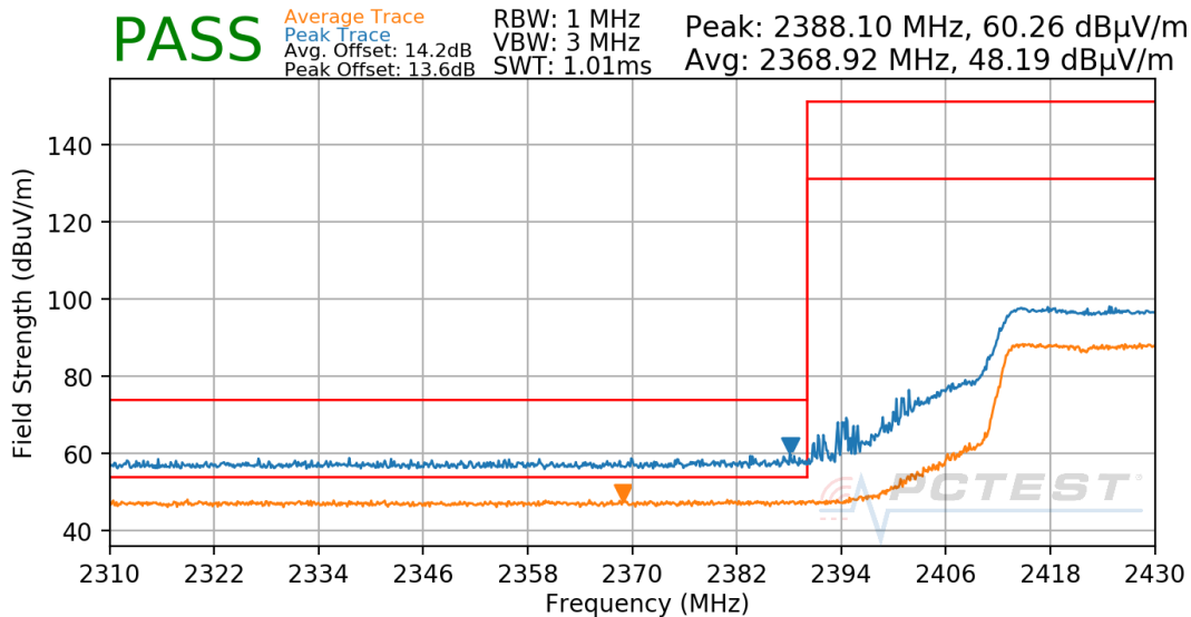
Plot 7-52. Radiated Restricted Lower Band Edge Measurement
