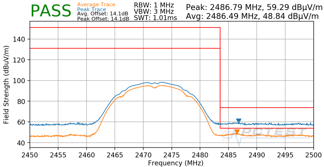
Plot 7-49. Radiated Restricted Upper Band Edge Measurement
