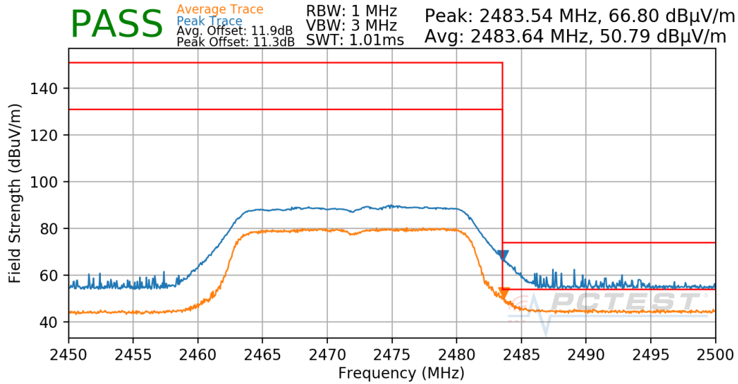
Plot 7-56. Radiated Restricted Upper Band Edge Measurement
