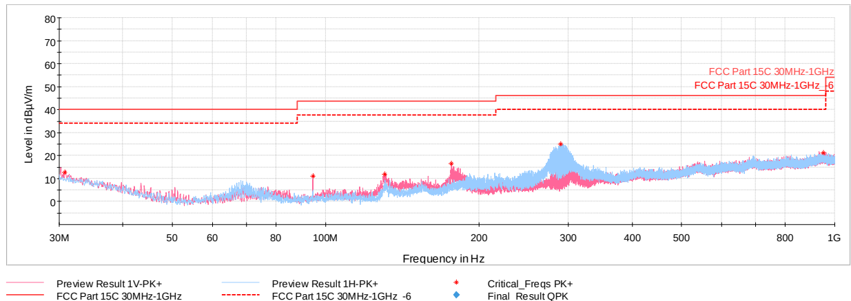
Plot 7-57. Radiated Spurious Emissions 30MHz-1GHz (802.11b – Ch.11, with WCP + laptop)
