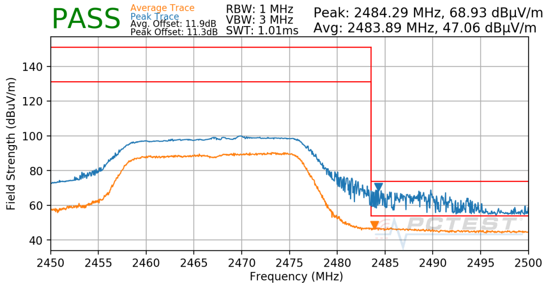
Plot 7-55. Radiated Restricted Upper Band Edge Measurement
