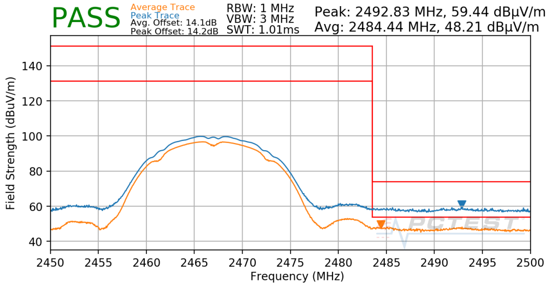
Plot 7-48. Radiated Restricted Upper Band Edge Measurement
