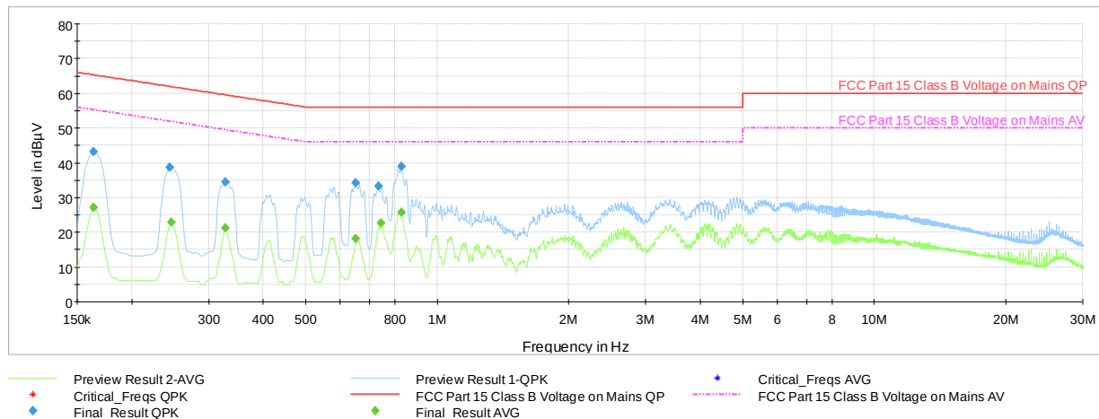
Plot 7-59. AC Line Conducted Emission with 802.11b Ch.11 (N, with WCP + AC/DC Adapter)
