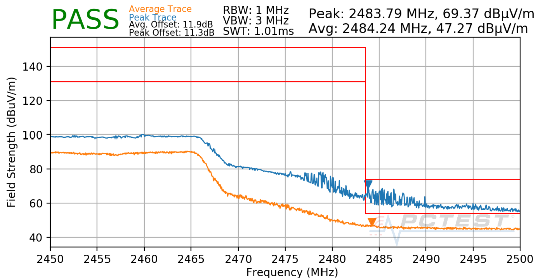
Plot 7-53. Radiated Restricted Upper Band Edge Measurement
