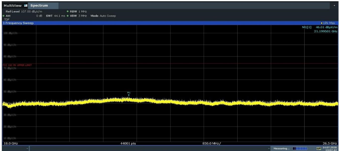
Plot 7-46. Radiated Spurious Emissions 18-26.5GHz (802.11b – Ch. 11, Ant. Pol. V)
