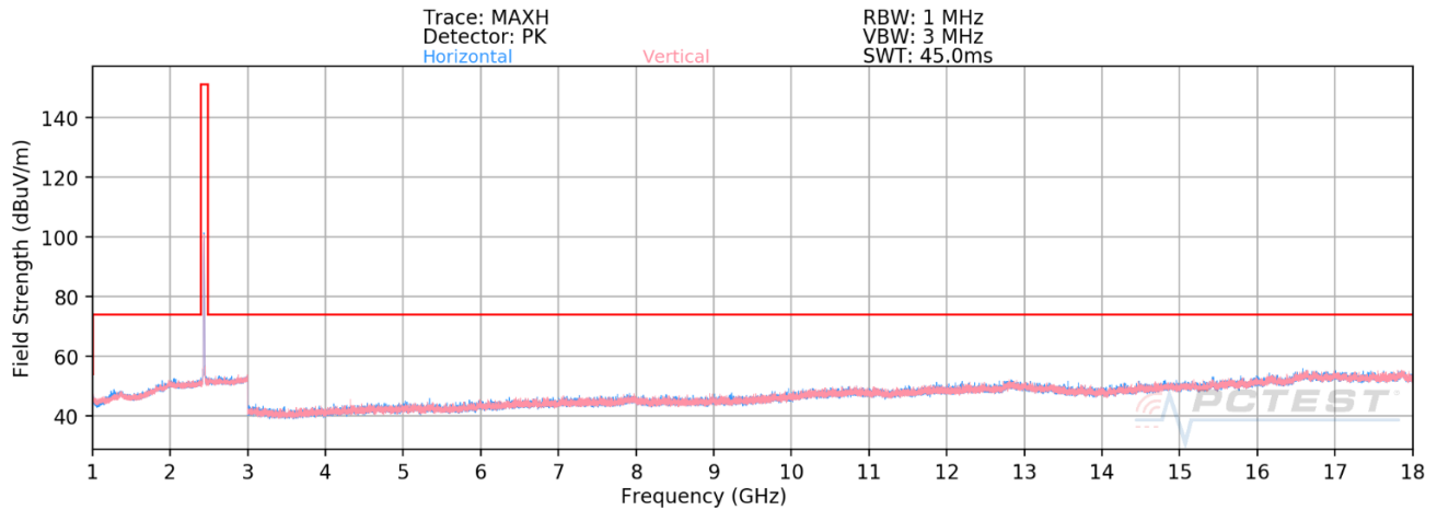
Plot 7-43. Radiated Spurious Emissions 1-18GHz (802.11b – Ch. 6)
