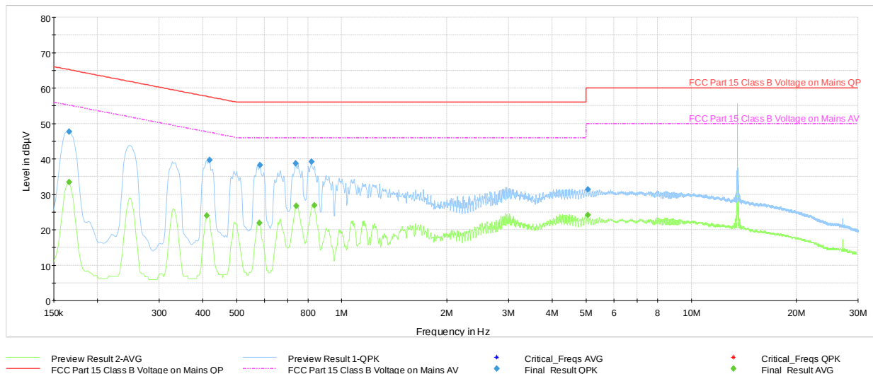
Plot 7-13. AC Line-Conducted Test Plot (N, CE A 848kbps, with WCP + AC/DC Adapter)
