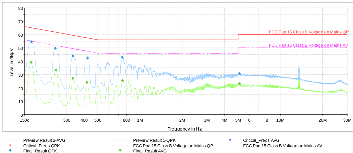
Plot 7-12. AC Line-Conducted Test Plot (L1, CE A 848kbps, with WCP + AC/DC Adapter)
